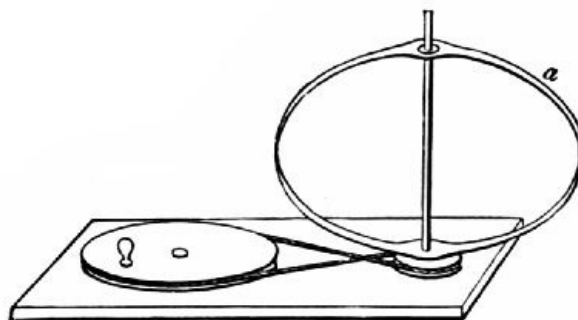
FIG. 71.—Well-known model exhibiting the oblate spheroidal form as a consequence of spinning about a central axis. The brass strip a looks
