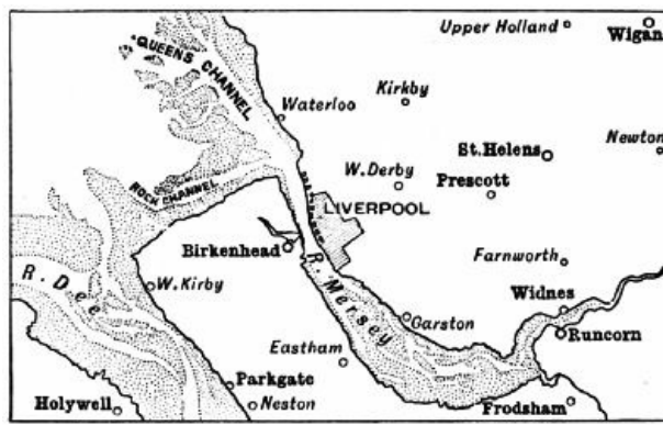
FIG. 108.—The Mersey
