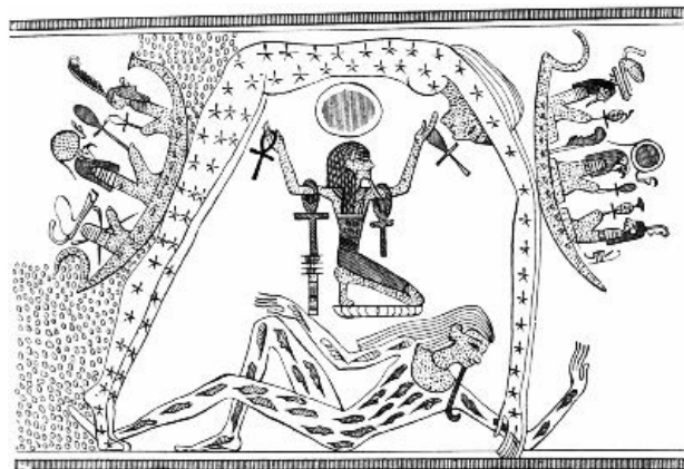
FIG. 5.—Egyptian Symbol of the Universe.
