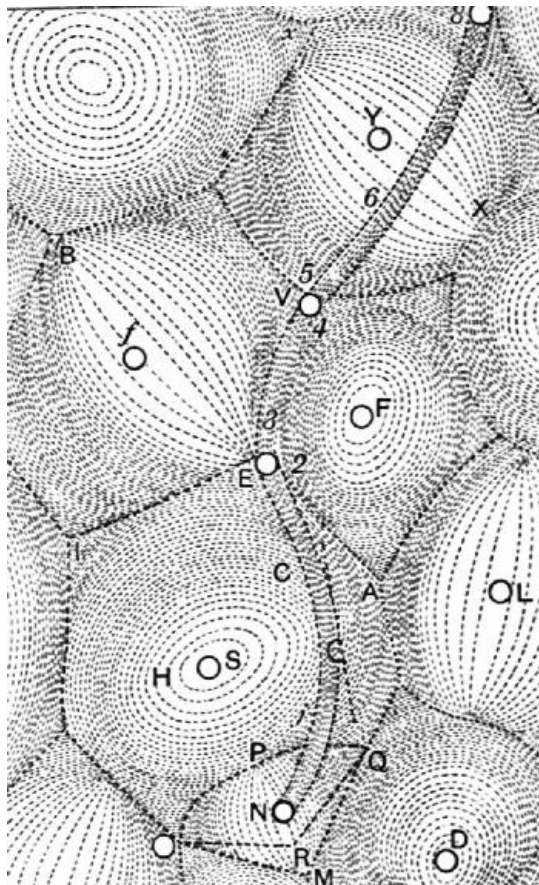
FIG. 55.—Descartes's diagram of vortices, from his Principia .
