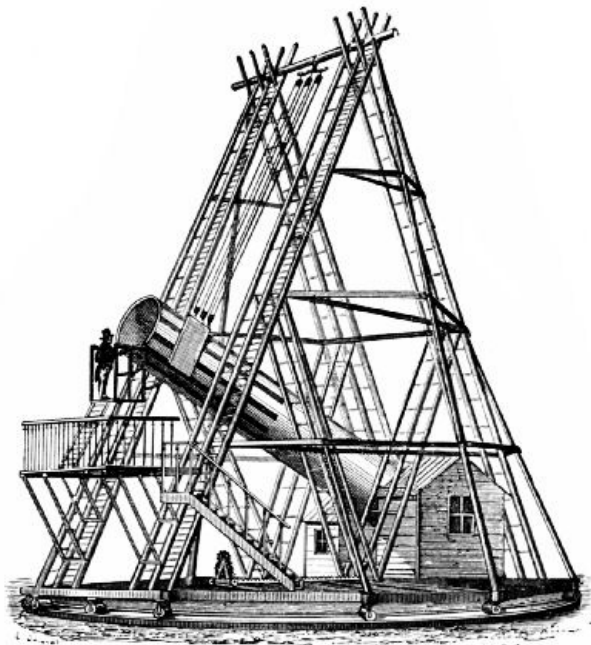
FIG. 83.—Herschel's 40-foot telescope.
