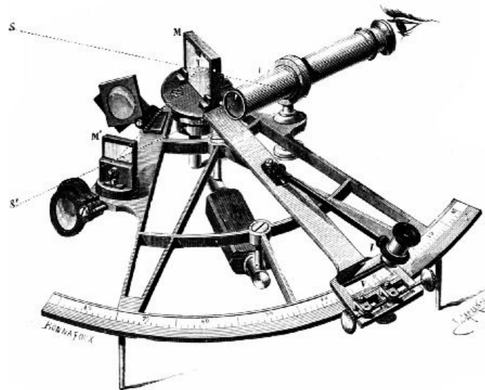
FIG. 67.—The sextant, as now made.
