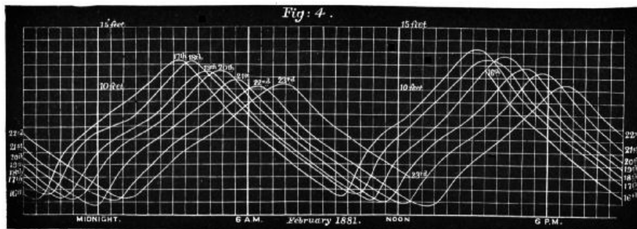
FIG. 120.—Weekly sheet of curves. Tides for successive days are predicted on the same sheet of paper, to economise space.
