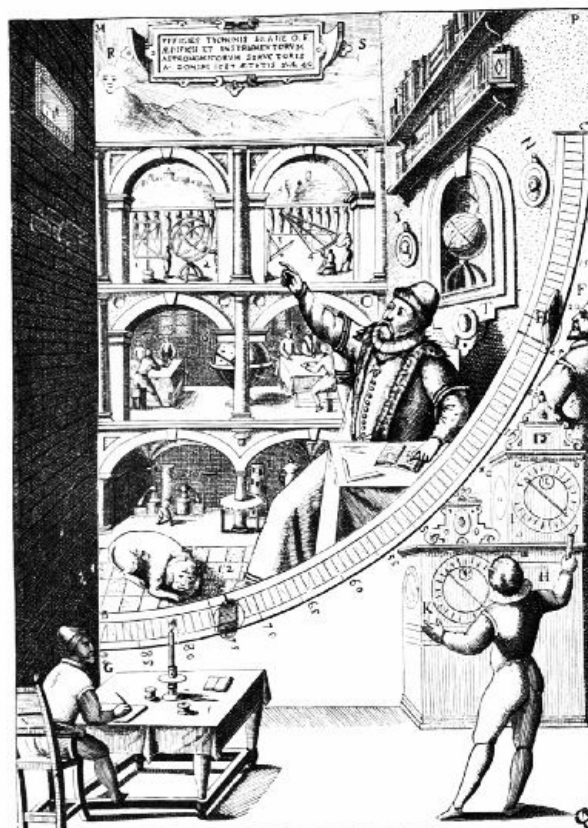
FIG. 24.—Tycho's form of transit circle.
