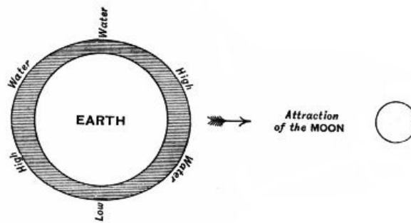
FIG. 112.—Earth and moon (earth's rotation neglected).
