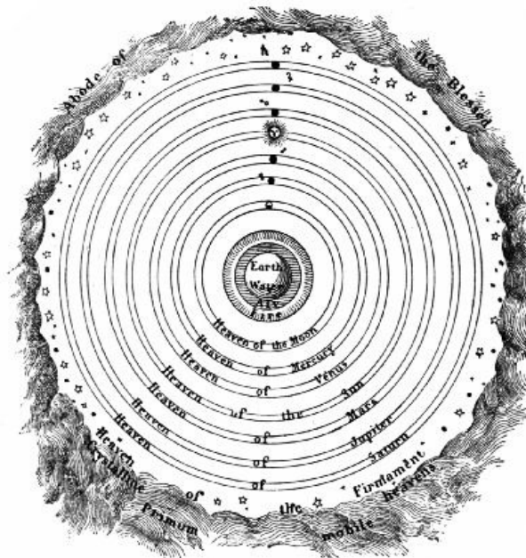
FIG. 8.—Ptolemaic system.
