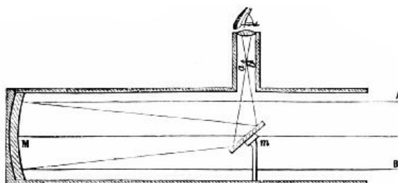
FIG. 82.—Principle of Newtonian reflector.
