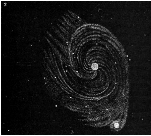
FIG. 80.—Lord Rosse's drawing of the spiral nebula in Canes Venatici, with the stub marks of the draughtsman unduly emphasised into features by the engraver.
