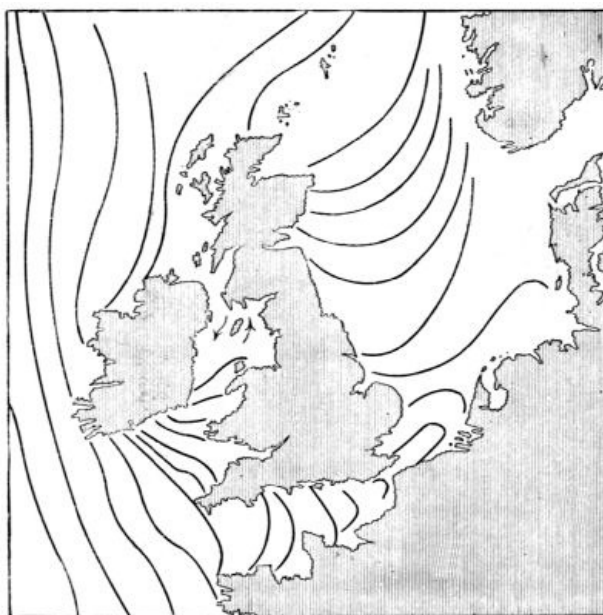
FIG. 109.—Co-tidal lines.
