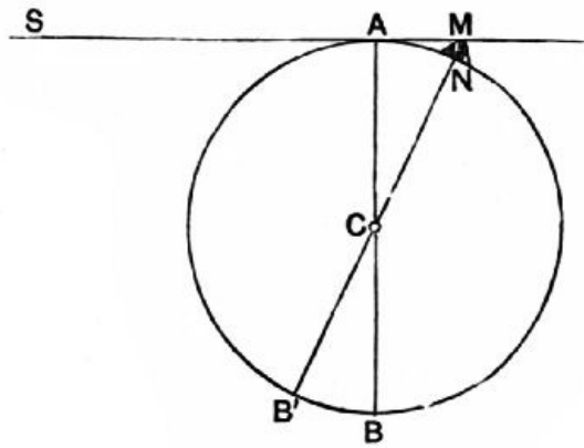
FIG. 42.—Galileo's method of estimating the height of lunar mountain. AB'BC is the illuminated half of the moon. SA is a solar ray just catching the peak of the mountain M . Then by geometry, as MN is to MA , so is MA to MB' ; whence the height of the mountain, MN , can be determined. The earth and spectator are supposed to be somewhere in the direction BA produced, i.e. towards the top of the page.
