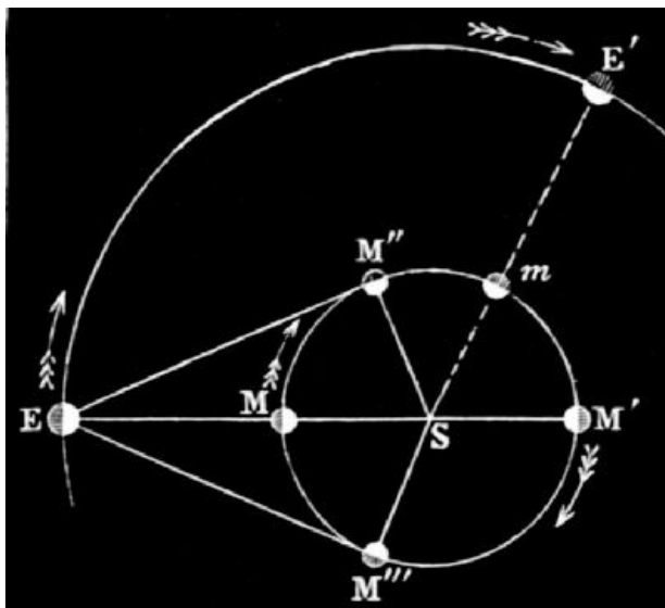
FIG. 13.—Orbit of Mercury and Earth.
