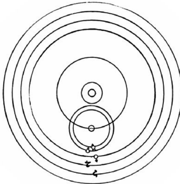
FIG. 11.—Egyptian system.
