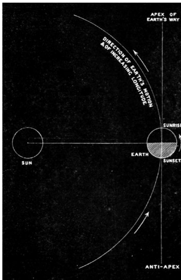
FIG. 97.—Diagram of direction of earth's orbital motion, showing that after midnight, i.e. between midnight and noon, more asteroids are likely to be swept up by any locality than between noon and midnight. [From Sir R.S. Ball.]
