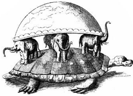
FIG. 6.—Hindoo Earth.
