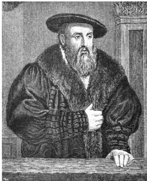
FIG. 34.—Portrait of Kepler, older.
