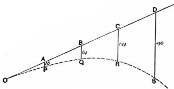
FIG. 35.—Curve described by a projectile, showing how it drops from the line of fire, OD , in successive seconds, the same distances AP , BQ , CR , &c., as are stated above for a dropped body.
