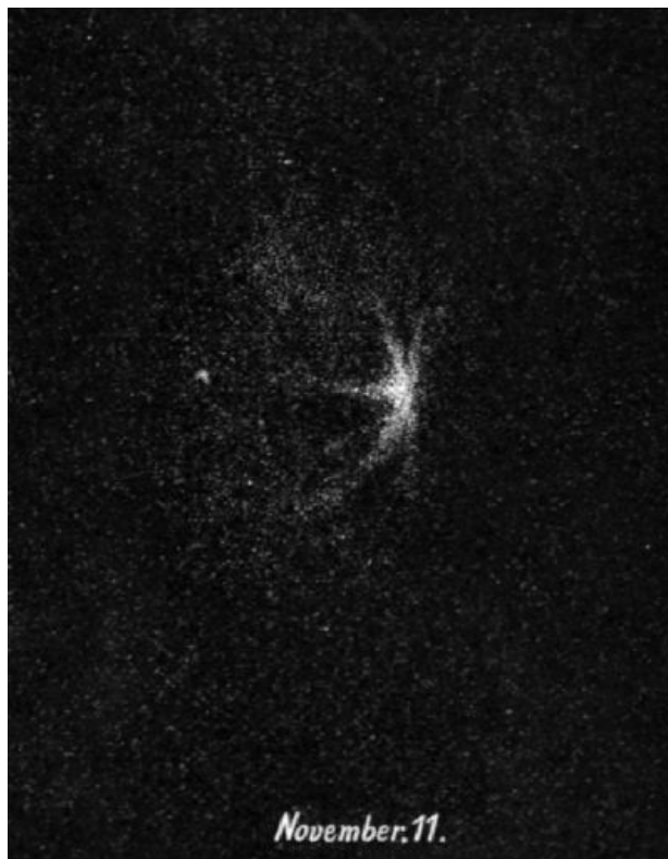
FIG. 103.—Encke's comet.
