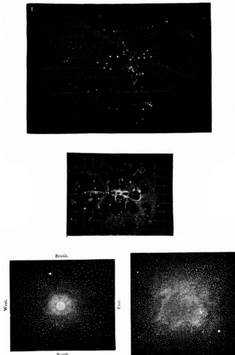
FIG. 43.—Some clusters and nebulae.
