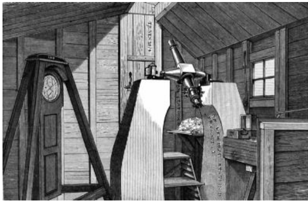
FIG. 76.—A Transit-instrument for the British astronomical expedition, 1874. Shewing in its essential features the simplest form of such an instrument.
