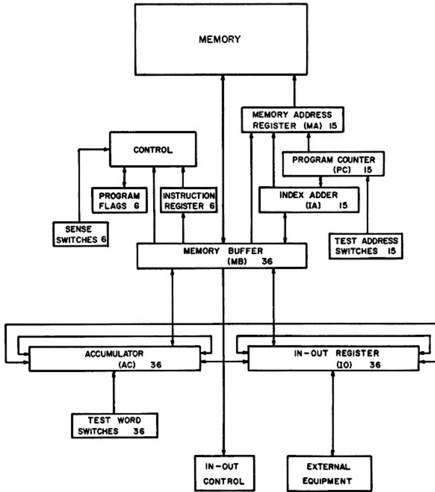
SYSTEM BLOCK DIAGRAM FIGURE 1
