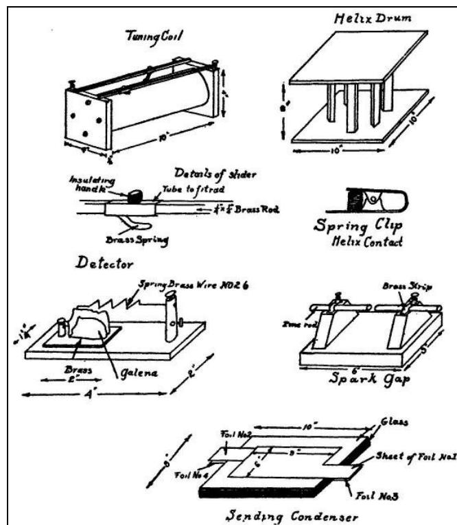
Details of instruments for field use.
