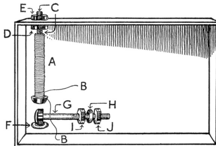
Fig. 191. The cigar-box telegraph.
