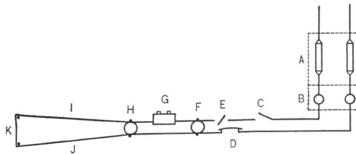
FIG. 190. Electrical apparatus: At the right are the incoming wires. Dotted lines show outlines of fuse block. A, 2 cartridge fuses, 15 A; B, 2 plug fuses, 10 A; C, knife switch; D, fuse gap; E, snap switch; F, H, lamp sockets; G, flush switch; I, J, K, nichrome resistance wire, No. 24 (total length of loop, 6 feet), passing around porcelain posts at left.
