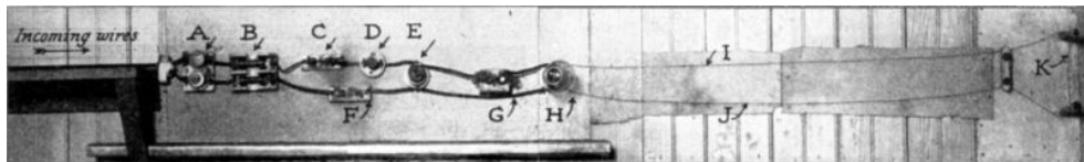
FIG. 121. Electrical apparatus: A, plug fuse; B, cartridge fuse; C, knife switch; D, snap switch; E, socket with nail plug in it; F, fuse gap; G, flush switch; H, lamp socket; I, J, K, resistance wire.
