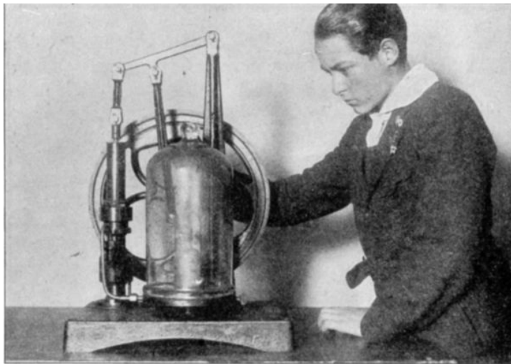
FIG. 6. An air pump.
