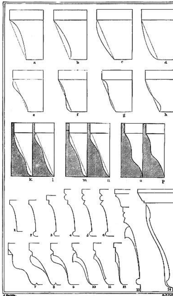
CORNICE PROFILES.
