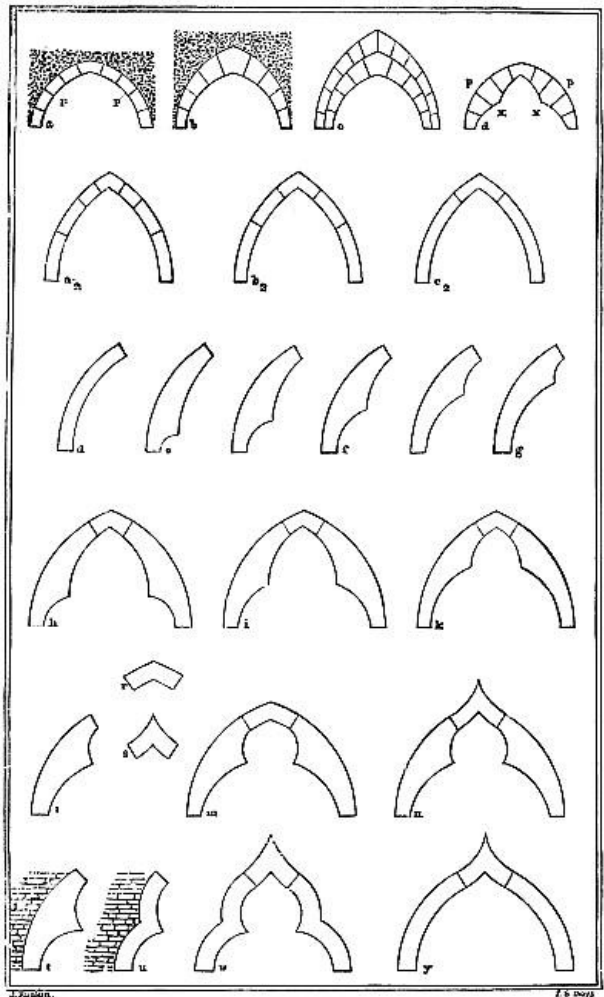
ARCH MASONRY.
