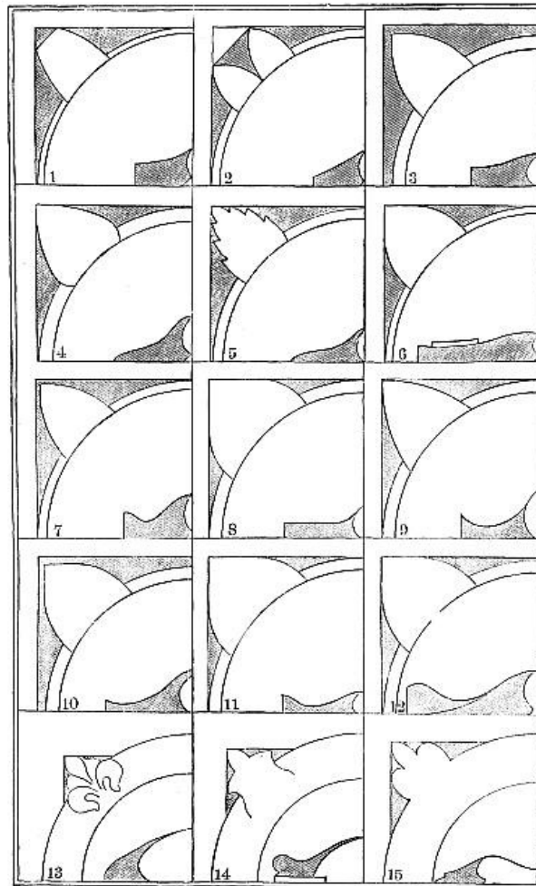
PLANS OF BASES.
