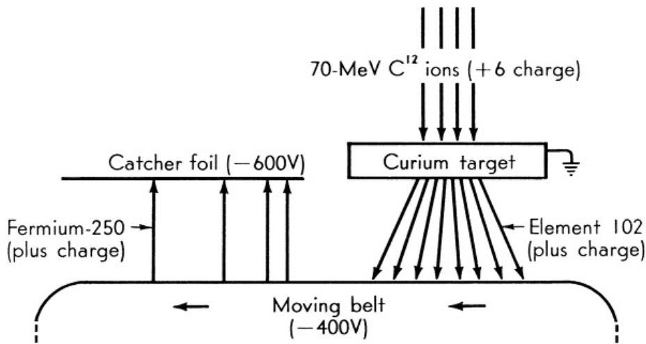
Fig. 4. The experimental arrangement used in the discovery of element 102.
