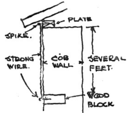
WALL COPINGS.
