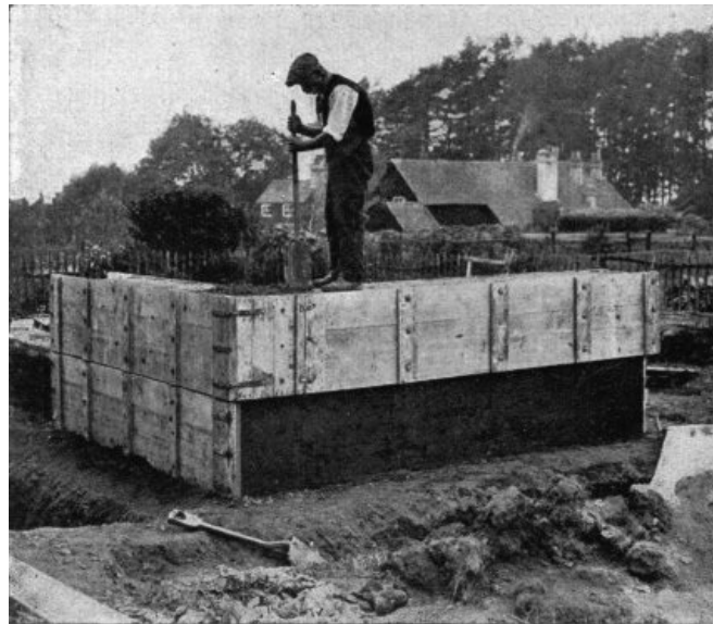
THE BEGINNING OF A PISÉ FRUIT-HOUSE.
