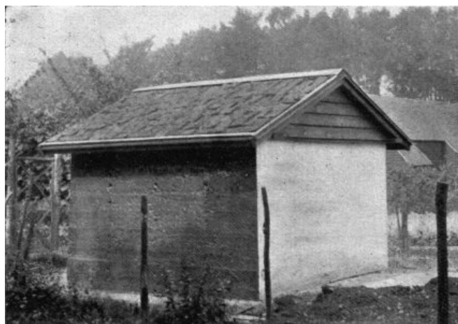
THE FRUIT-HOUSE COMPLETED WITH ROOF OF PEAT BLOCKS ON ROUGH BOARDING.
