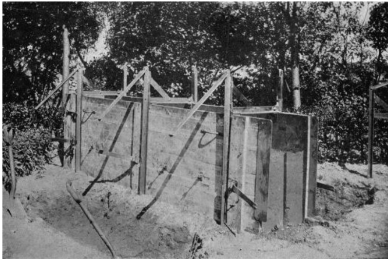
MARK V SHUTTERING. Shuttering about to be removed from a first section of Pisé walling. Top cross-braces have been thrown back and clamps to legs released. It is now only necessary to detach the stays and lift away the shutters. Where, as here, there is no masonry plinth, the bearing-pins are only required for the succeeding courses of Pisé, and need not be inserted for the first.
