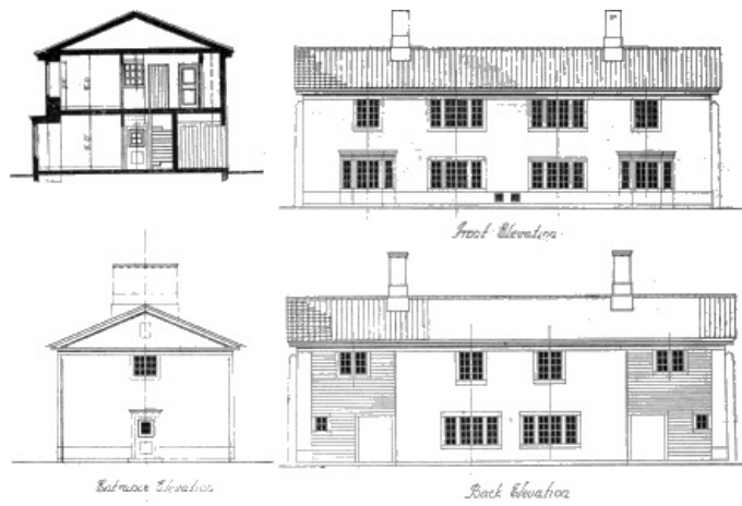
FRONT AND BACK ELEVATIONS OF COTTAGE DESIGNED BY SIR EDWIN LUTYENS AND MR. ALBAN SCOTT.
