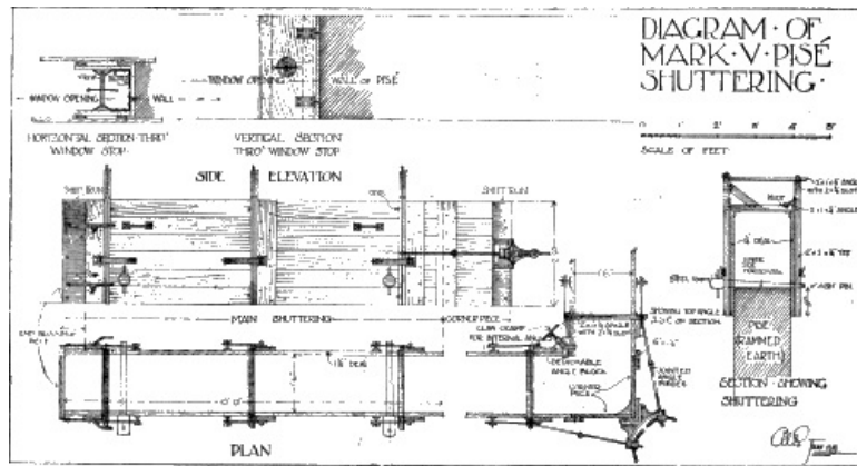
DIAGRAM OF MARK V PISE SHUTTERING
