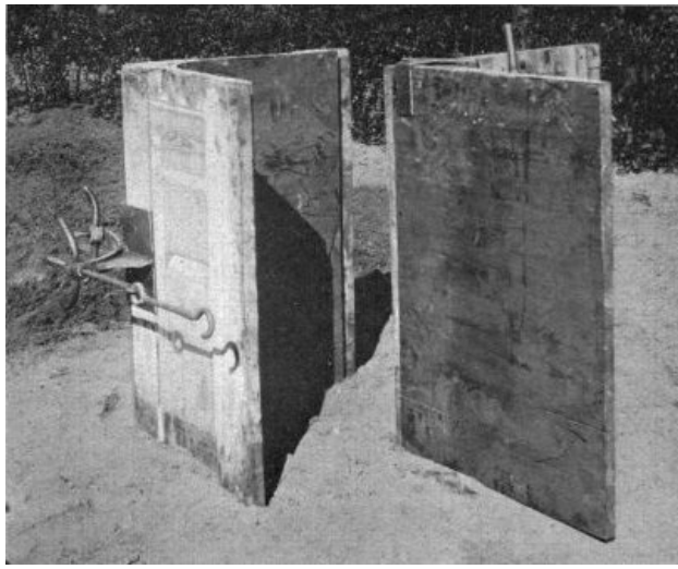
MARK V SHUTTERING. Showing screw-up securing tackle of exterior corner-piece and its rounded interior. Also screw-cramp at interior angle of shuttering.
