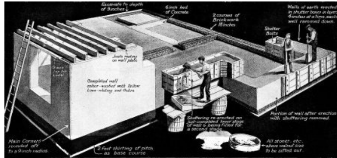
SKETCH OF A PISÉ HOUSE IN COURSE OF ERECTION. With acknowledgements to The Sphere .
