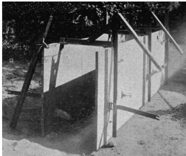
MARK V SHUTTERING.
