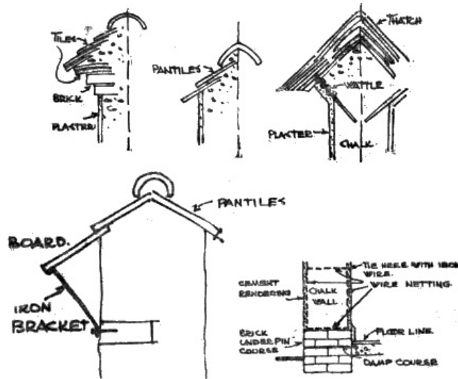
WALL COPINGS.
