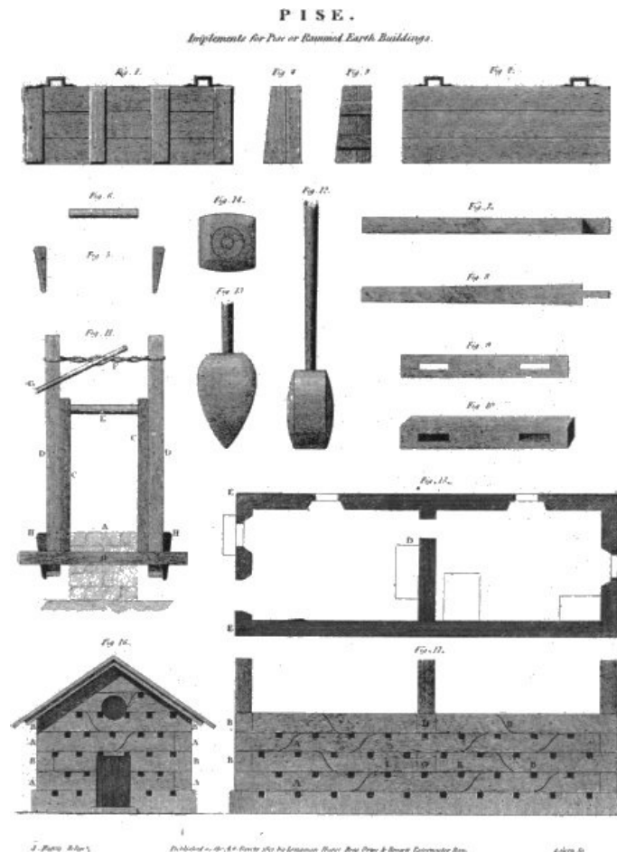
PISÉ. Implements for Pisé or Rammed Earth Buildings PISÉ PLANT AND IMPLEMENTS. (Reproduced from an old Encyclopædia.)
