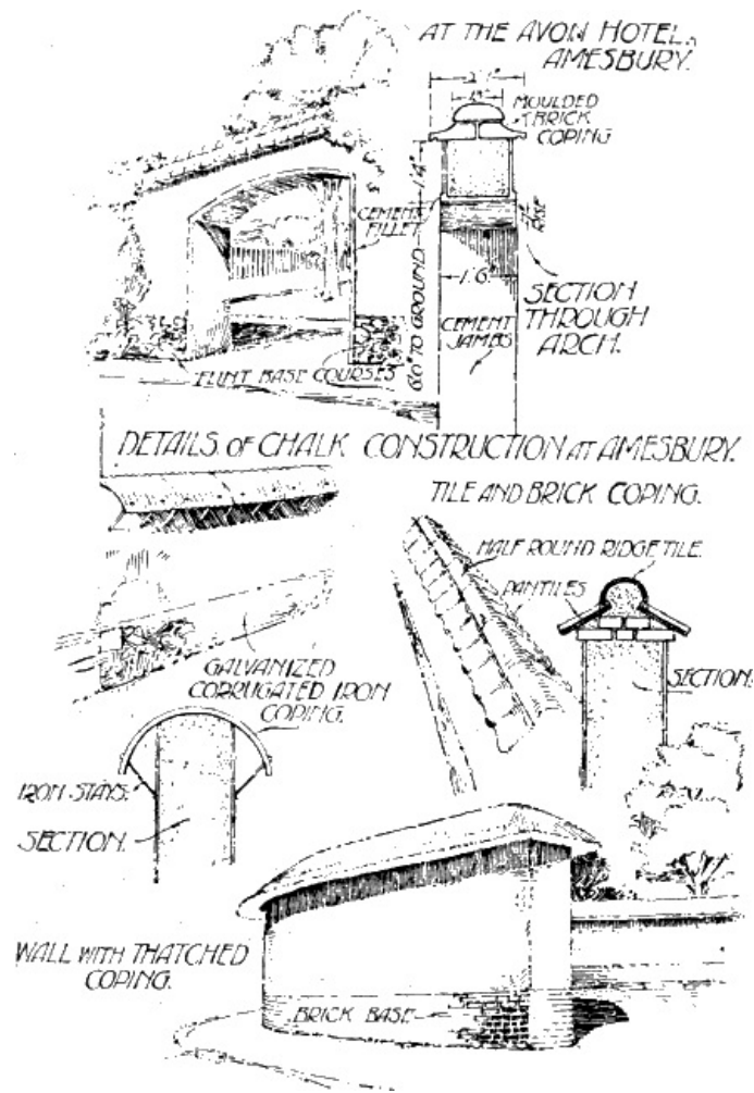
DETAILS OF CHALK CONSTRUCTION AT AMESBURY. (From a sketch by W. R. Jaggard, F.R.I.B.A., the copyright of the Department of Scientific and Industrial Research.)
