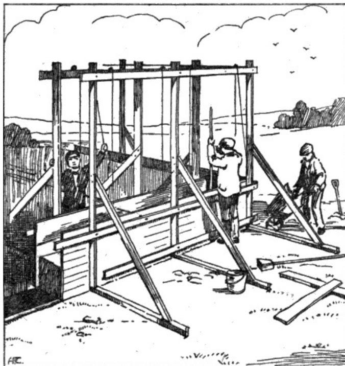
PATENT SHUTTERING FOR PISÉ DE TERRE By W. Alban Richards and Co.
