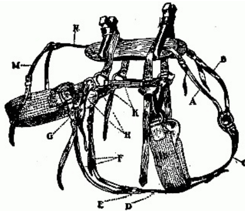
Mr. Ernest Britten's Pack Rig.
