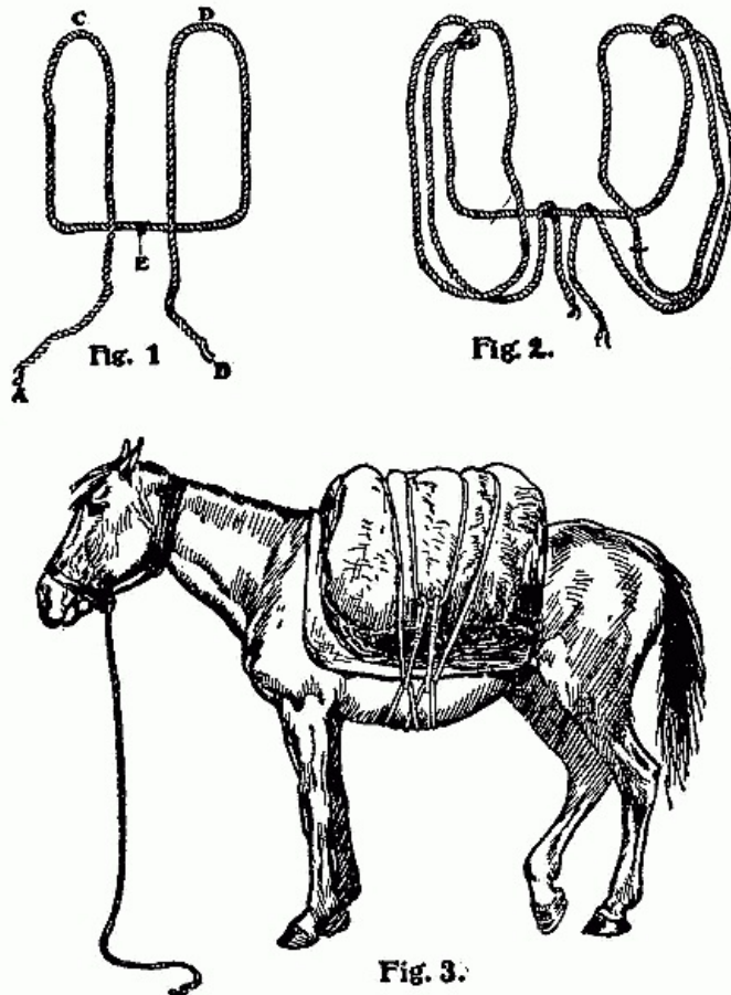
The Squaw Hitch.
