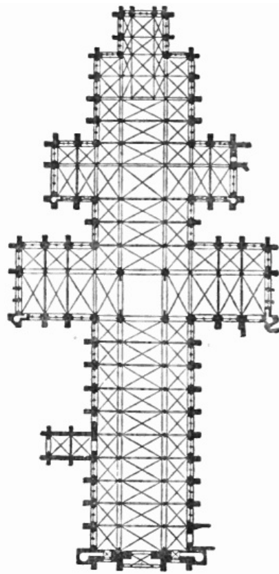
Plan of Salisbury Cathedral
