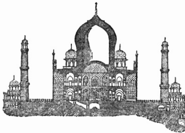
Section of Taj Mahal, Agra
