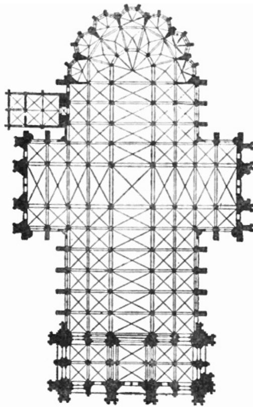
Plan of Cologne Cathedral
