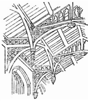
Hammer Beam Roof
