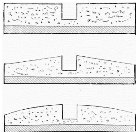
FIG. 61.—SECTIONS OF SETTING BOARDS.
