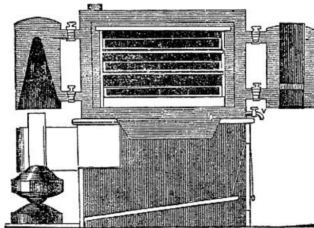
Fig. 43. Egg-Hatcher, or Eccalobeeon.
