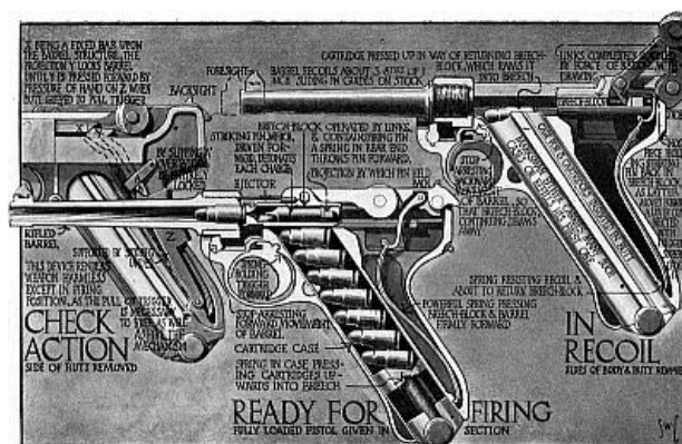
A GERMAN AUTOMATIC PISTOL. The action is fully described on the illustration.
