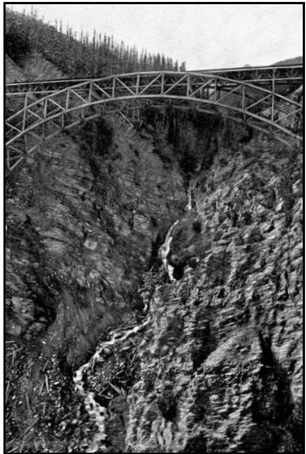
STONY CREEK BRIDGE—Height 296 feet.
