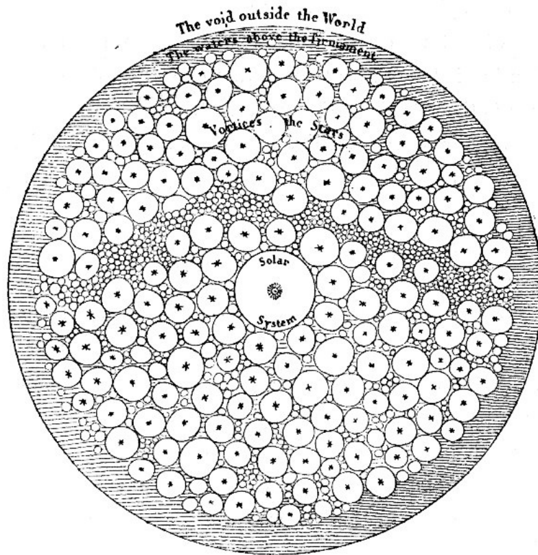
FIG. 23.—VORTICES OF THE STARS.
