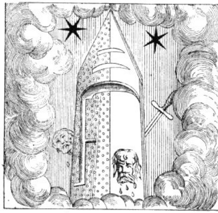
FIG. 55.—REPRESENTATION OF A COMET, 16TH CENTURY.
