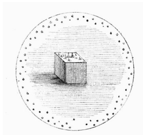
FIG. 30.—PLATO'S CUBICAL EARTH.
