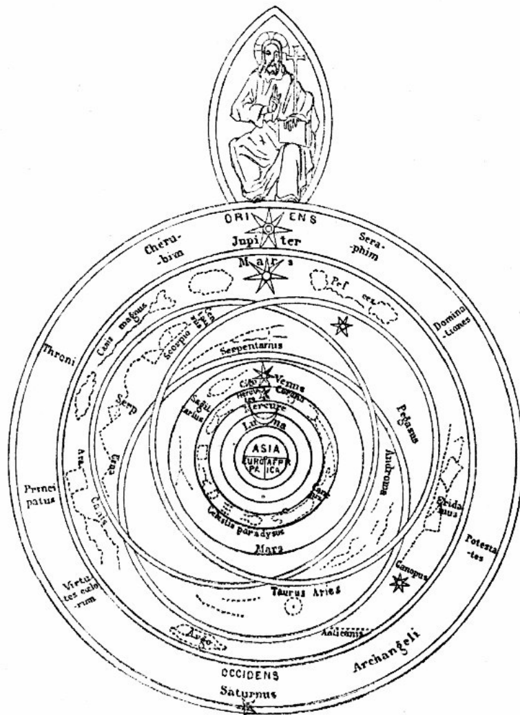
FIG. 16.—HEAVENS OF THE MIDDLE AGES.
