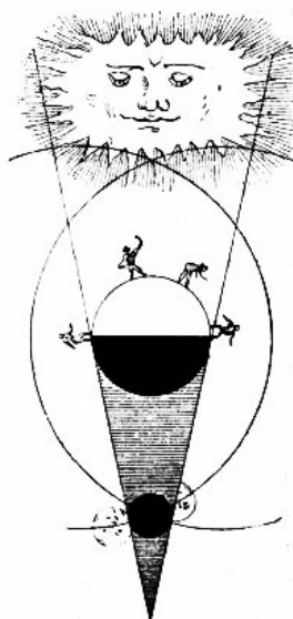
FIG. 35.—THE EARTH'S SHADOW.
