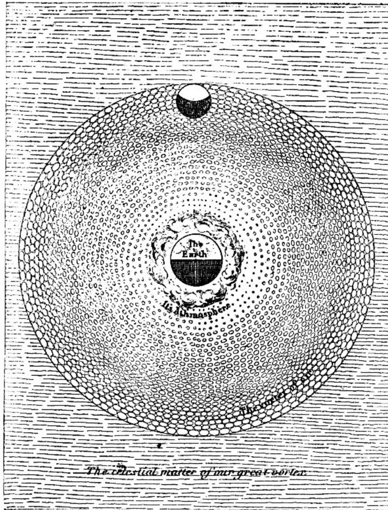
FIG. 22.—DESCARTES' THEORY OF VORTICES.
