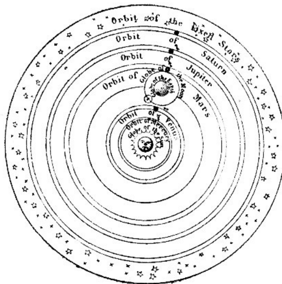
FIG. 20.—THE COPERNICAN SYSTEM.
