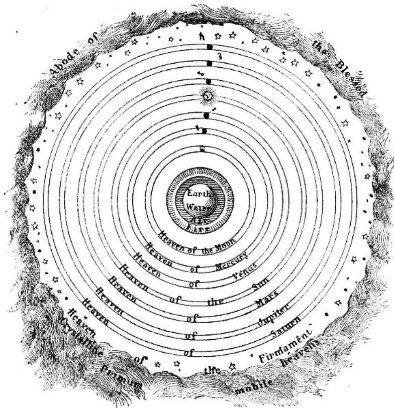
FIG. 14.—PTOLEMY'S ASTRONOMICAL SYSTEM.
