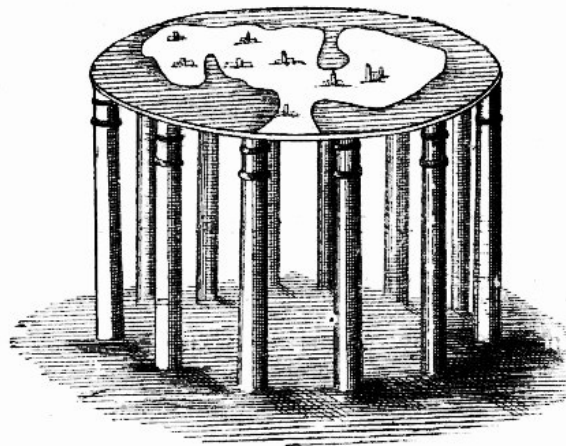
FIG. 27.—THE EARTH OF THE VEDIC PRIESTS.
