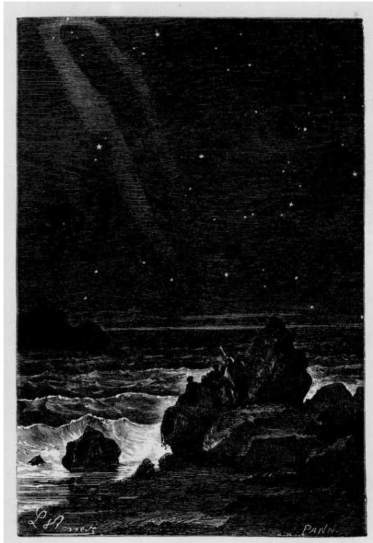
THE CONSTELLATIONS FROM THE SEA-SHORE.
