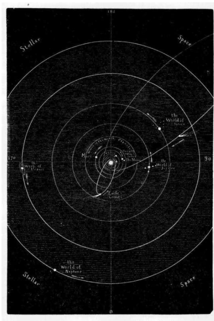
PLATE IX.—THE SOLAR SYSTEM.
