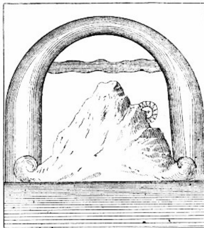
FIG. 41.—EXPLANATION OF SUNRISE.
