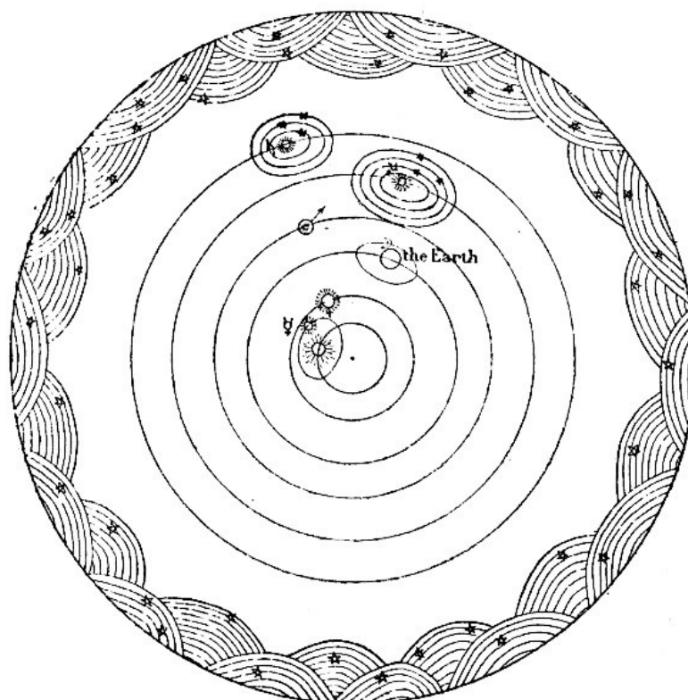
FIG. 24.—VARIATION OF DESCARTES' THEORY.
