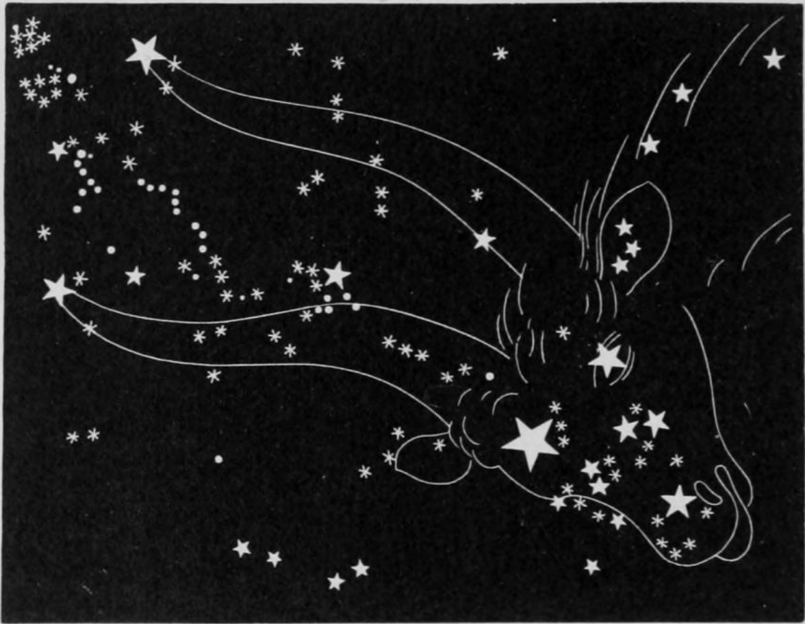
THE "GOLDEN HORNS" OF TAURUS.
