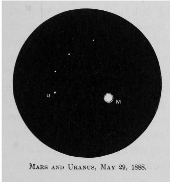
MARS AND URANUS, MAY 29, 1888.
