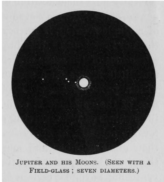
JUPITER AND HIS MOONS. (SEEN WITH A FIELD-GLASS; SEVEN DIAMETERS.)
