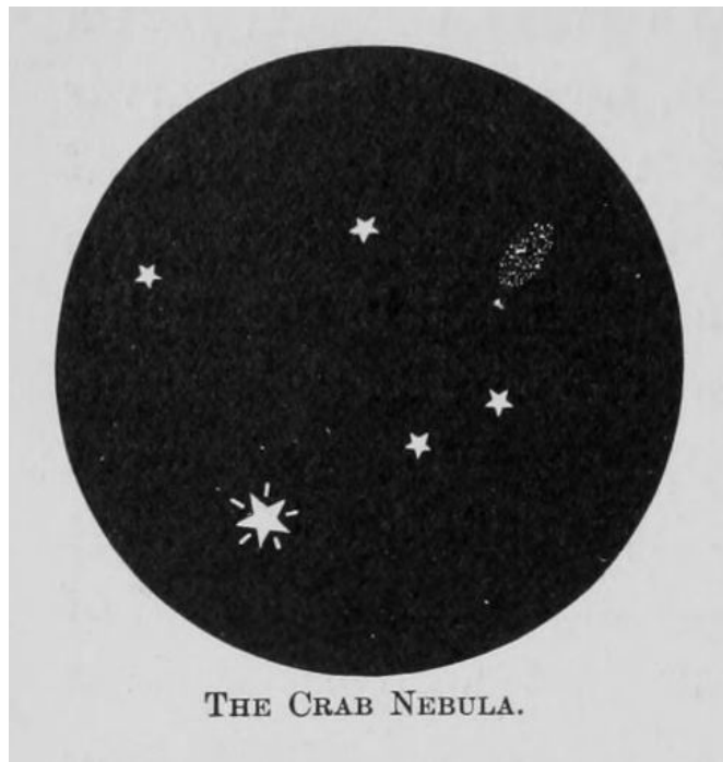
THE CRAB NEBULA.
