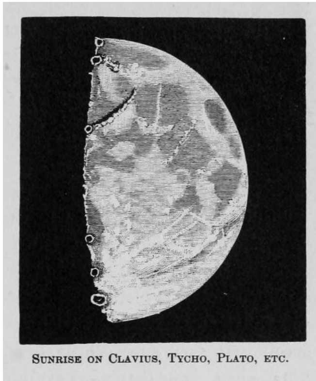
SUNRISE ON CLAVIUS, TYCHO, PLATO, ETC.
