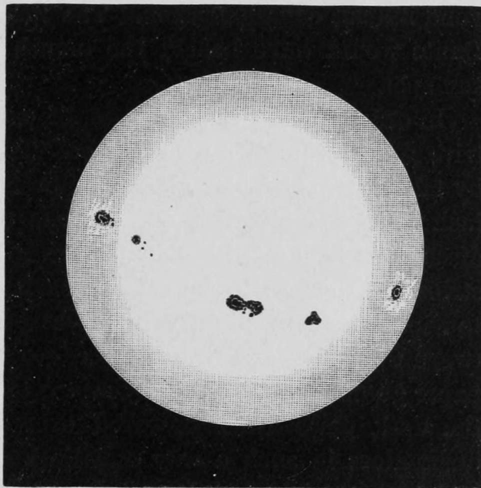
THE SUN, SEPTEMBER 1, 1883.
