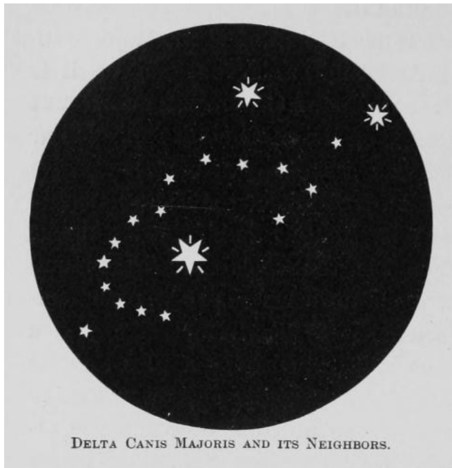
DELTA CANIS MAJORIS AND ITS NEIGHBORS.
