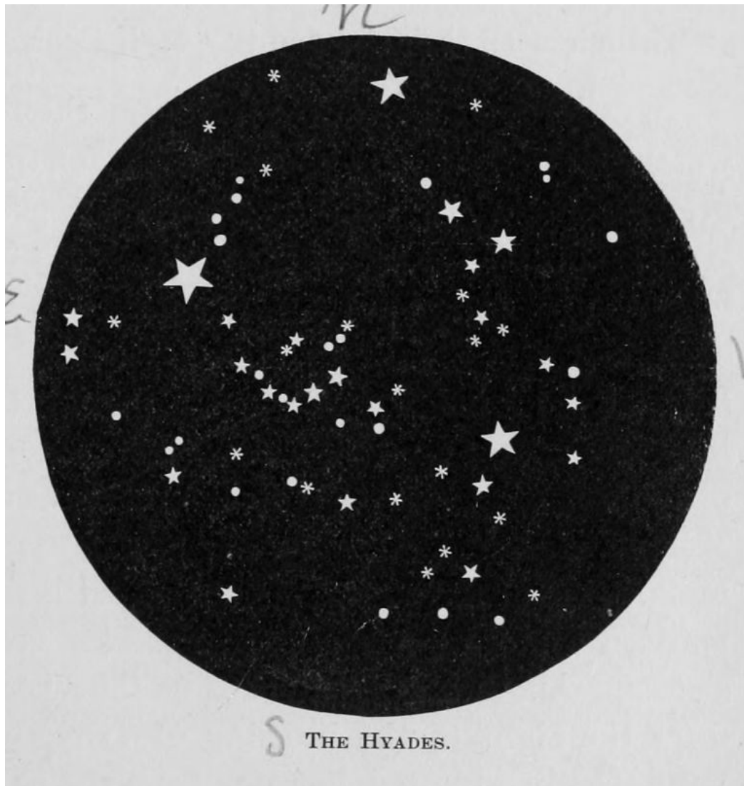
THE HYADES.
