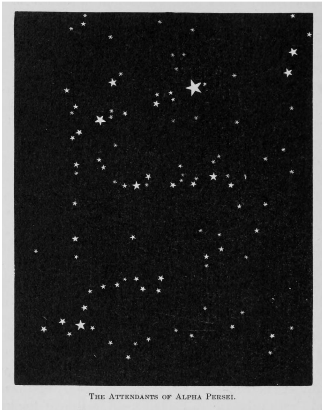
THE ATTENDANTS OF ALPHA PERSEI.
