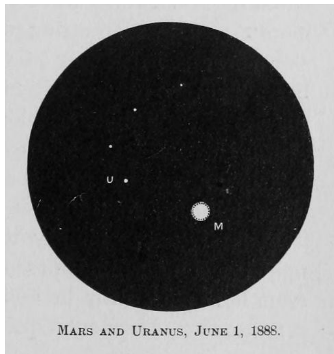
MARS AND URANUS, JUNE 1, 1888.
