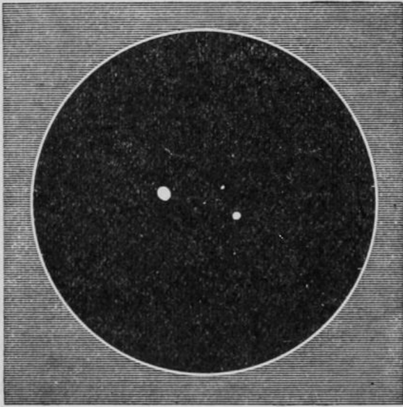
MIZAR, ALCOR, AND THE SIDUS LUDOVICIANUM.
