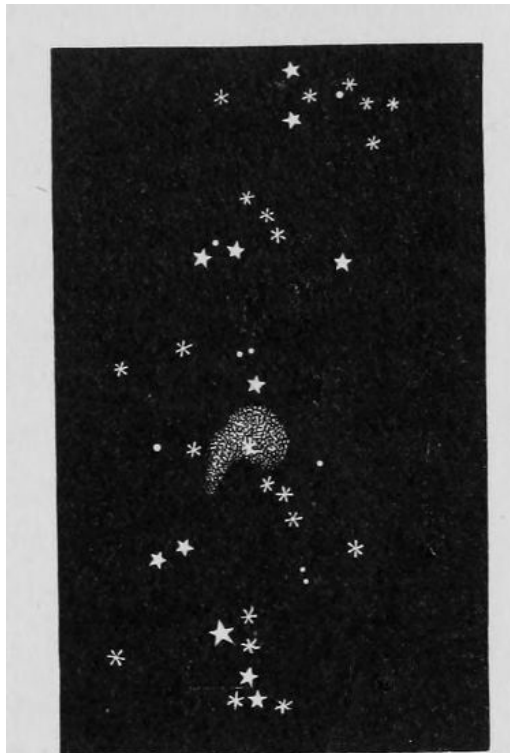
THE SWORD OF ORION AND THE GREAT NEBULA.
