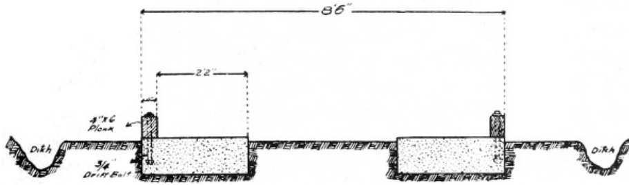
Figure 2. Cross section of concrete road. Scale—1 inch equals 2 feet.
