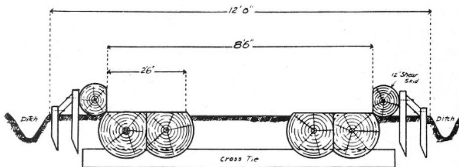
Figure 1. Cross section of pole road. Scale—1 inch equals 2 feet.
