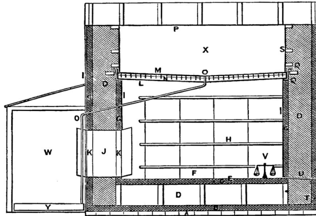
Fig. 28.—NYCE'S FRUIT PRESERVING HOUSE. (LONGITUDINAL SECTION.)
