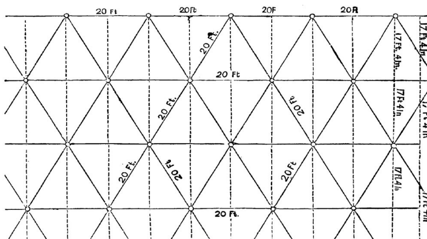
Fig. 26.—DIAGRAM OF PLANTING QUINCUNX.
