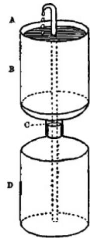
Fig. 24. A, surface of brine. B, upper can filled with brine. C, necks of cans telescoped. D, lower can full of water.
