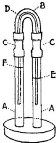
FIG. 18. E, water surface. F, brine surface.
