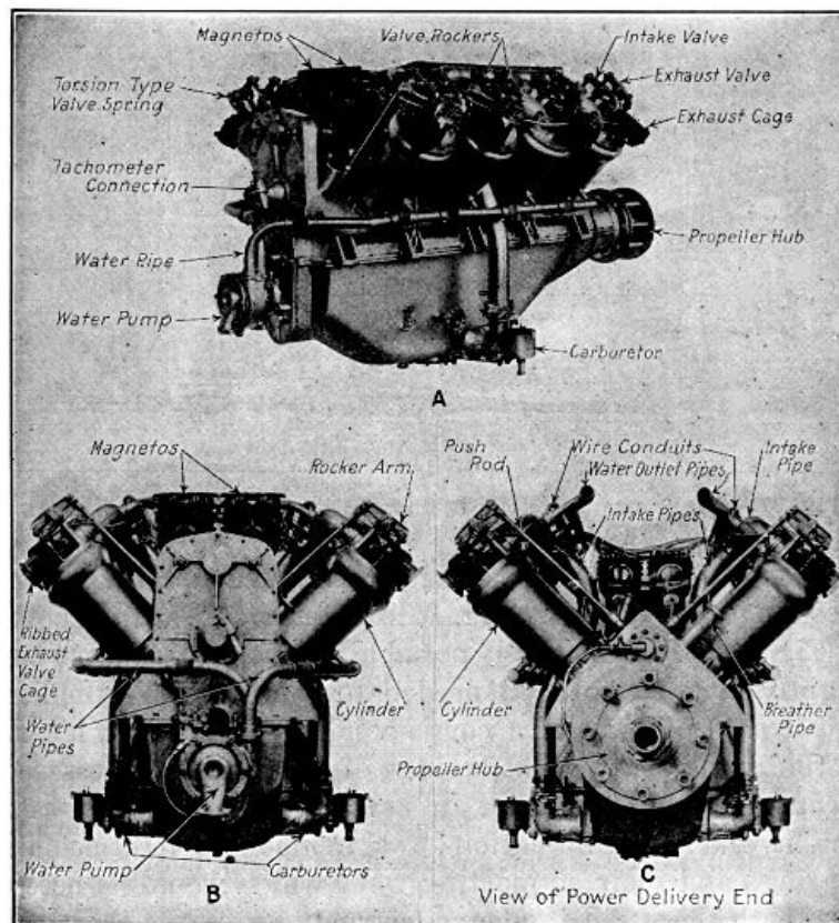
Fig. 36.—The Curtiss Eight-Cylinder, 200 Horse-Power Aviation Engine.
