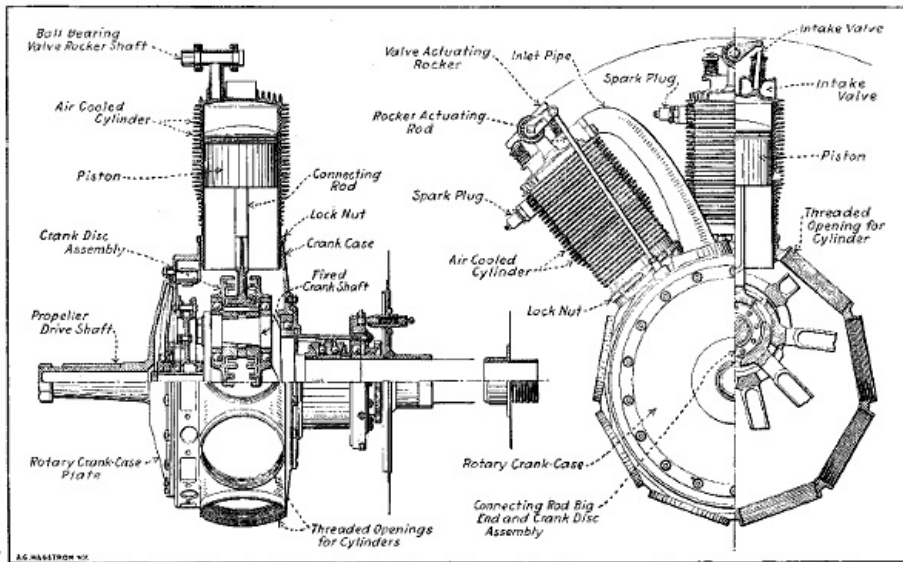
Fig. 216.—Part Sectional Views of Le Rhone Rotary Cylinder Engine, Showing Method of Cylinder Retention, Valve Operation and Novel Crank Disc Assembly.
