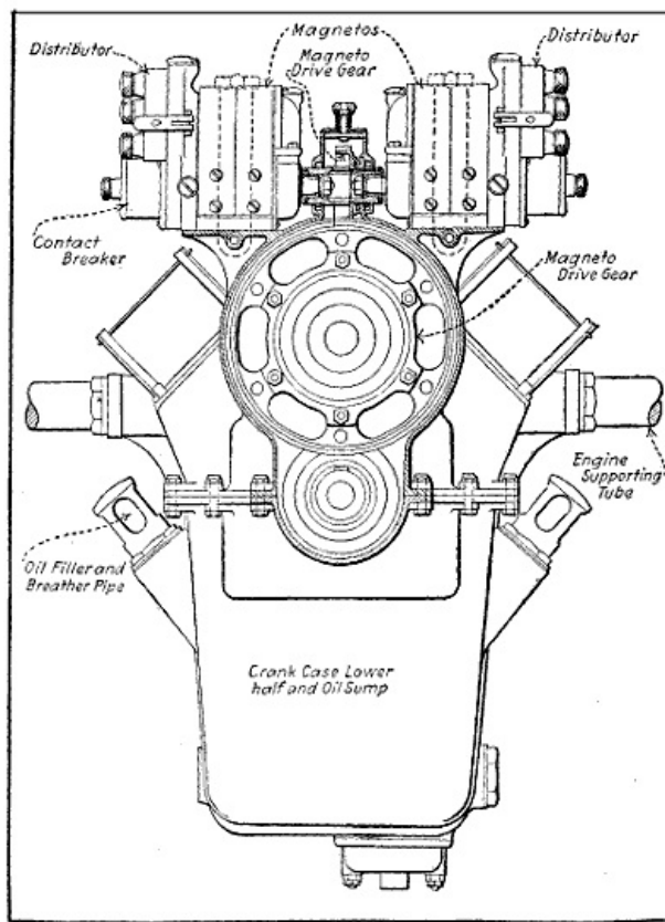
Fig. 228.—End View of Renault Twelve-Cylinder Engine Crank-Case, Showing Magneto Mounting.
