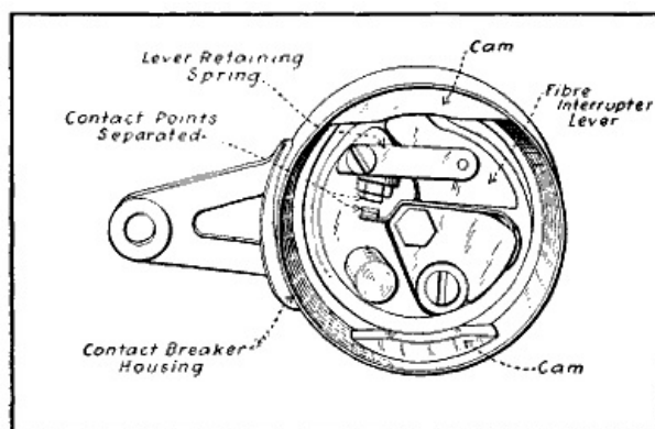
Fig. 65.—The Berling Magneto Breaker Box Showing Contact Points Separated and Interrupter Lever on Cam.
