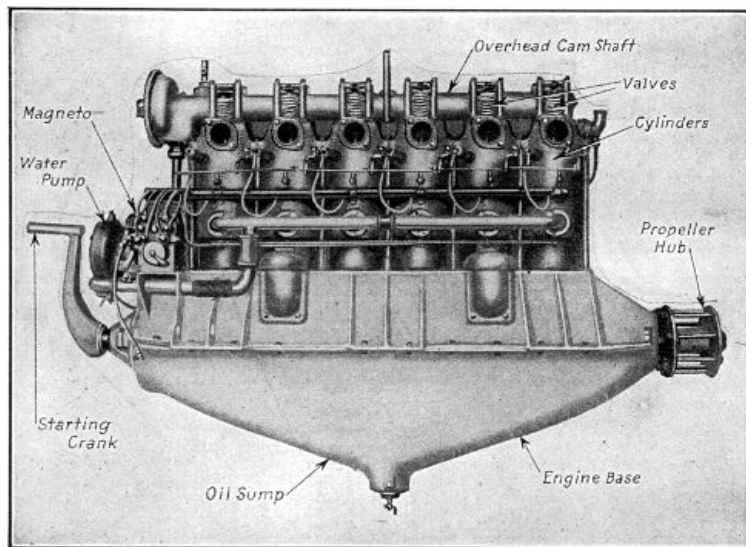
Fig. 35.—The Hall-Scott Six-Cylinder Aviation Engine.
