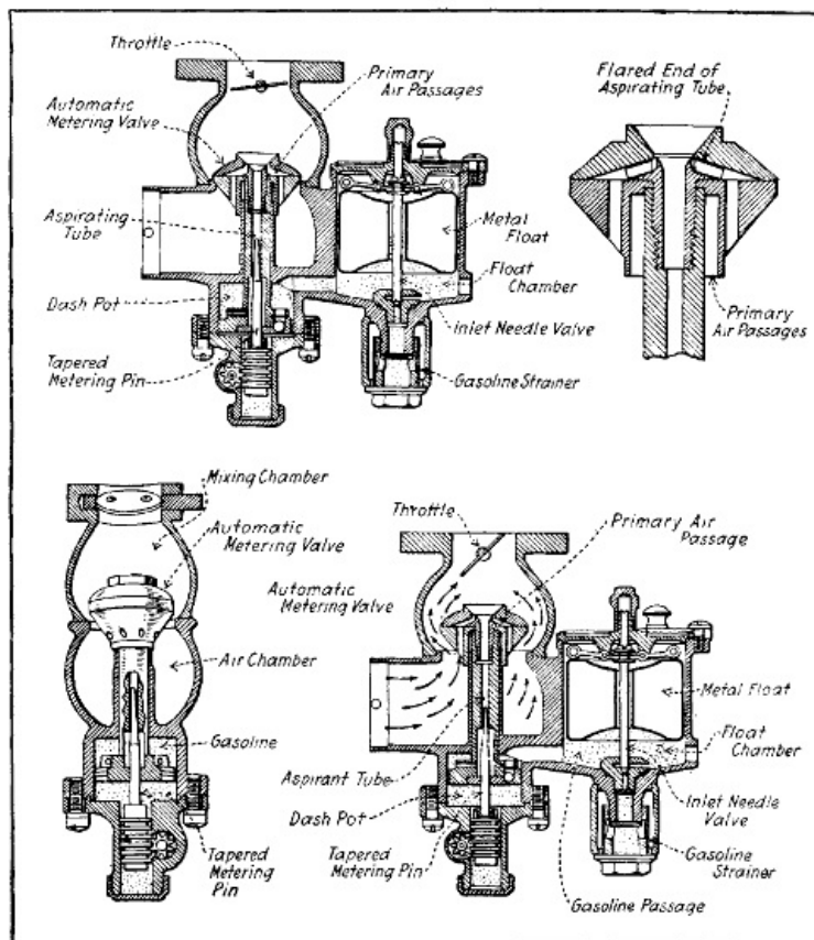
Fig. 47.—The Stewart Metering Pin Carburetor.
