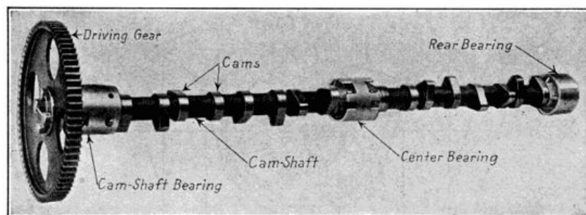
Fig. 104.—Cam-Shaft of Thomas Airplane Motor Has Cams Forged Integral. Note Split Cam-Shaft Bearings and Method of Gear Retention.
