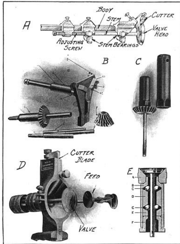
Fig. 183.—Tools for Restoring Valve Head and Seats.
