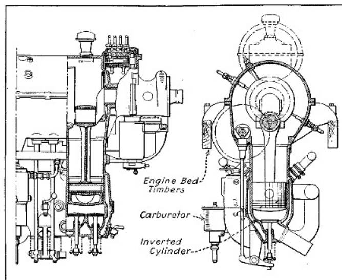
Fig. 144.—Unconventional Mounting of German Inverted Cylinder Motor.
