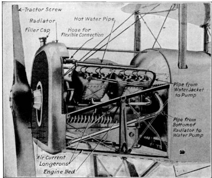
Fig. 83.—How Water Cooling System of Thomas Airplane Engine is Installed in Fuselage.
