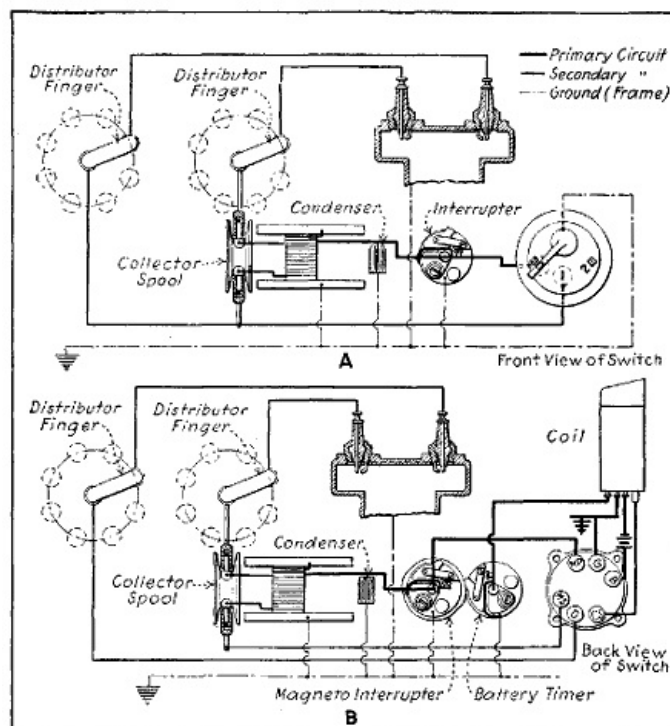
Fig. 64.—Wiring Diagrams of Berling Magneto Ignition Systems.
