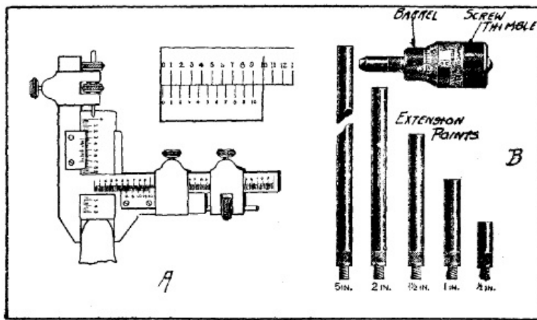
Fig. 176.—At Left, Special Form of Vernier Caliper for Measuring Gear Teeth; at Right, Micrometer for Accurate Internal Measurements.
