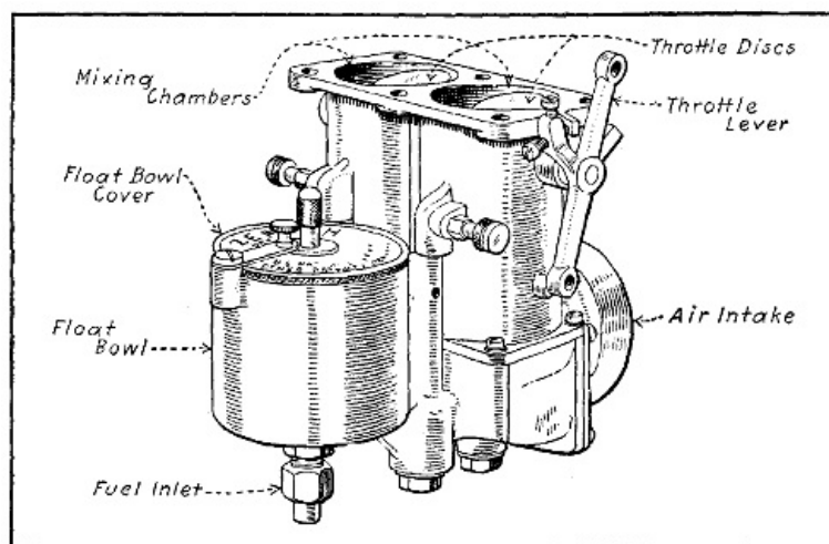
Fig. 53.—The Zenith Duplex Carburetor for Airplane Motors of the V Type.
