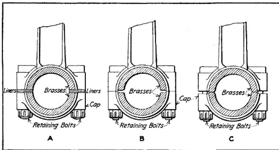
Fig. 188.—Showing Points to Observe When Fitting Connecting Rod Brasses.
