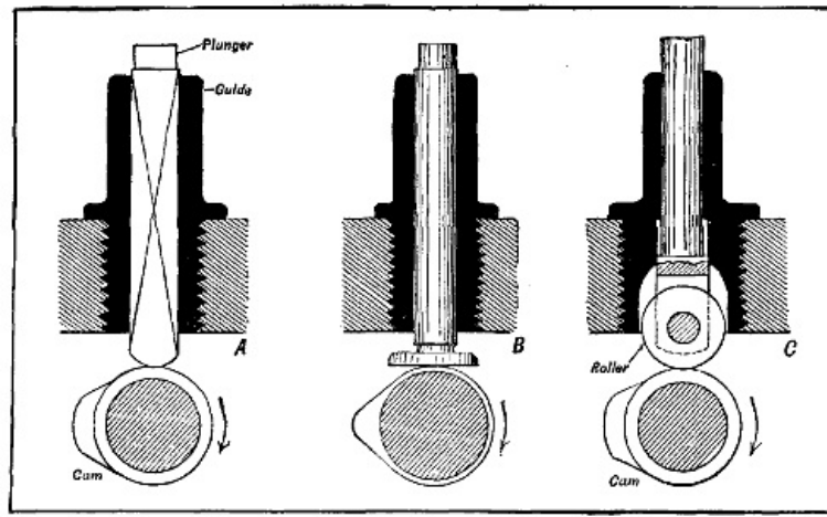
Fig. 102.—Showing Principal Types of Cam Followers which Have Received General Application.
