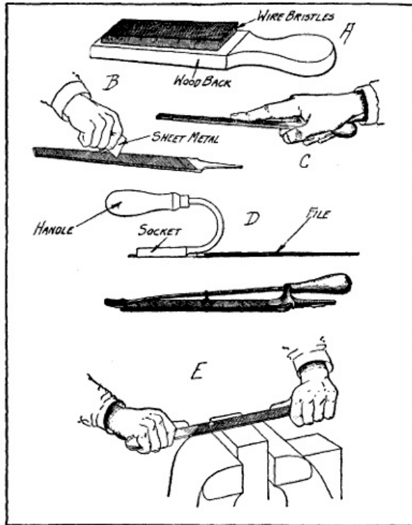
Fig. 165.—Illustrating Use and Care of Files.
