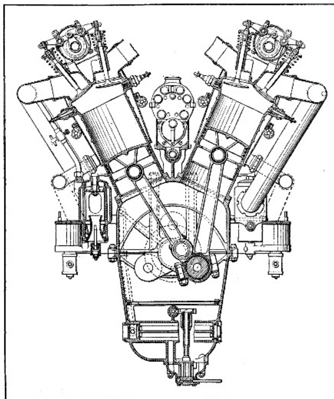
Fig. 132.—Part Sectional View of Renault Twelve-Cylinder Water-Cooled Engine, Showing Connecting Rod Construction and Other Important Internal Parts.
