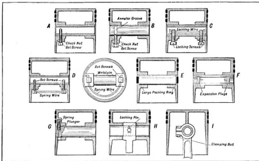
Fig. 117.—Typical Methods of Piston Pin Retention Generally Used in Engines of American Design. A—Single Set Screw and Lock Nut. B—Set Screw and Check Nut Fitting Groove in Wrist Pin. C, D—Two Locking Screws Passing Into Interior of Hollow Wrist Pin. E—Split Ring Holds Pin in Place. F—Use of Taper Expanding Plugs Outlined. G—Spring Pressed Plunger Type. H—Piston Pin Pinned to Connecting Rod. I—Wrist Pin Clamped in Connecting Rod Small End by Bolt.
