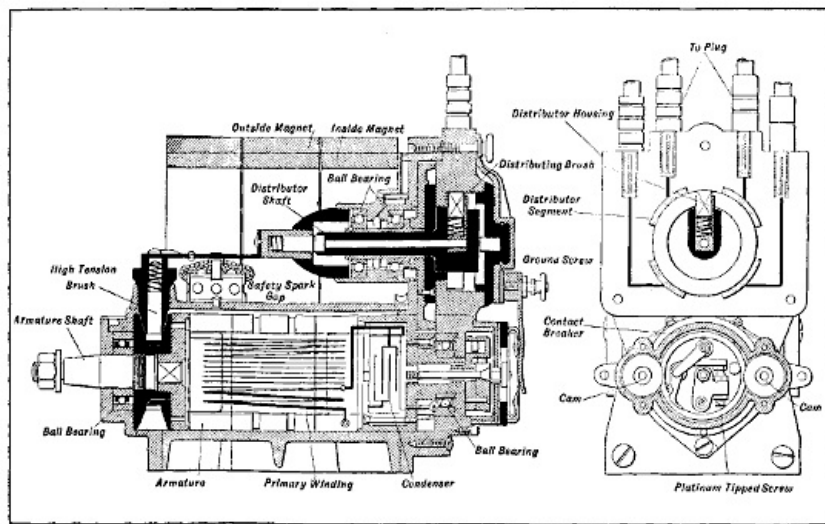
Fig. 60A.—Side Sectional View of Bosch High-Tension Magneto Shows Disposition of Parts. End Elevation Depicts Arrangement of Interrupter and Distributor Mechanism.
