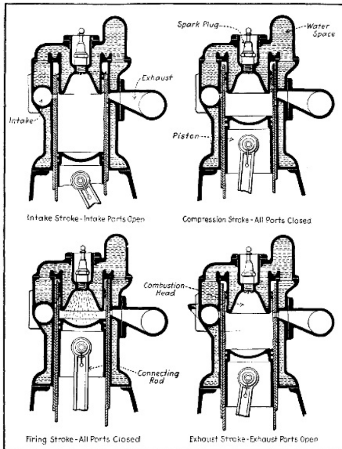
Fig. 106.—Diagrams Showing Knight Sleeve Valve Action.
