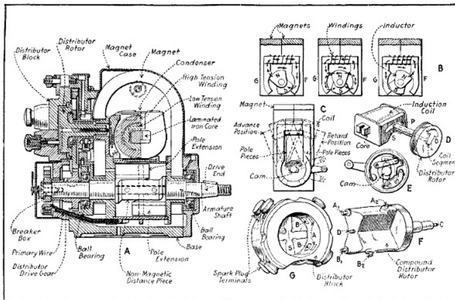
Fig. 69A.—Sectional Views Outlining Construction of Dixie Magneto with Compound Distributor for Eight-Cylinder Engine Ignition.
