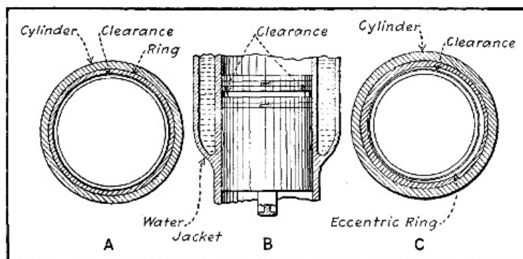
Fig. 124.—Diagrams Showing Advantages of Concentric Piston Rings.
