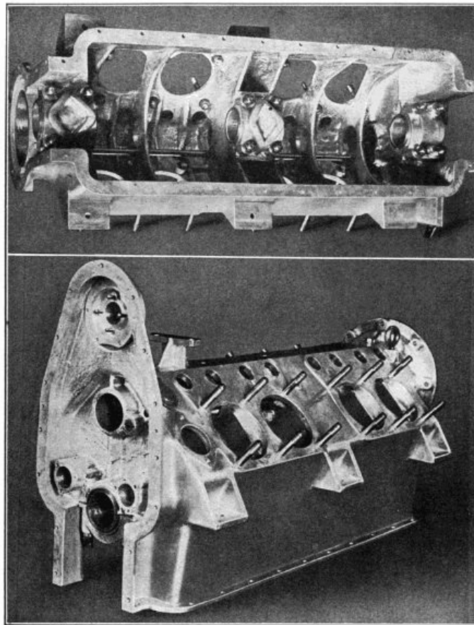
Fig. 141.—Views of Upper Half of Thomas Aeromotor Crank-Case.
