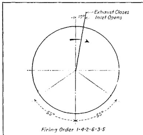
Fig. 241.—Timing Diagram, Wisconsin Aviation Engine.
