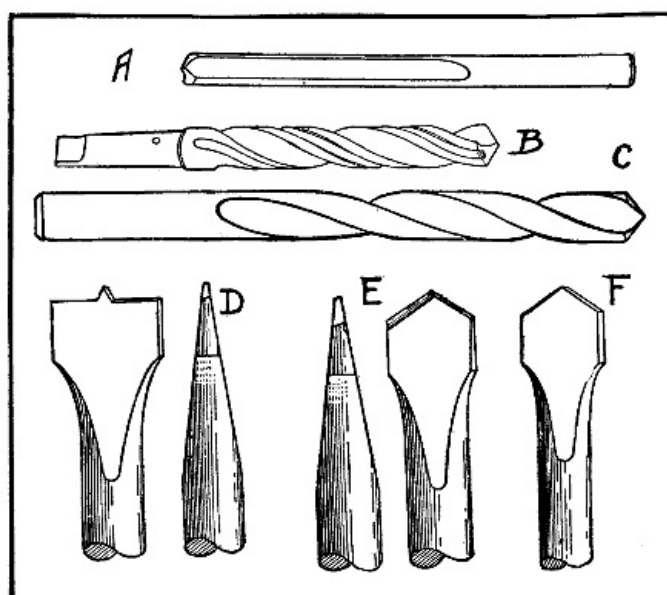
Fig. 168.—Forms of Drills Used in Hand and Power Drilling Machines.
