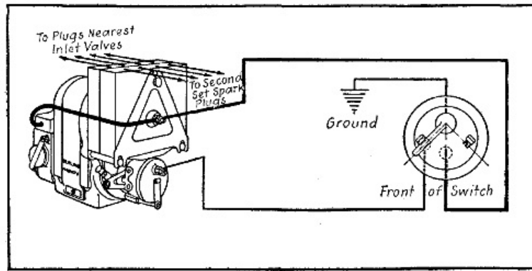
Fig. 62.—Berling Double-Spark Independent System.
