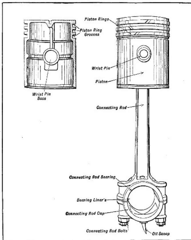
Fig. 118.—Typical Piston and Connecting Rod Assembly.
