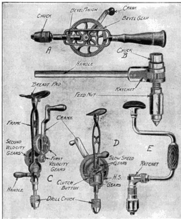
Fig. 167.—Forms of Hand Operated Drilling Machines.
