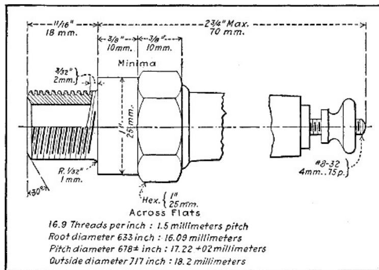
Fig. 73.—Standard Airplane Engine Plug Suggested by S. A. E. Standards Committee.
