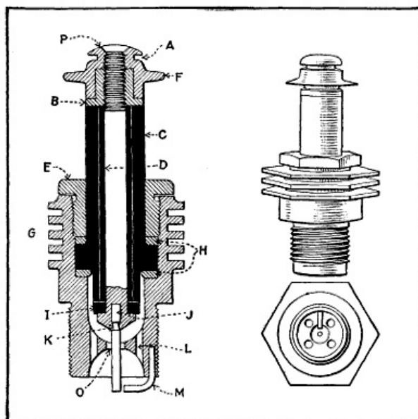
Fig. 74.—Special Mica Plug for Aviation Engines.
