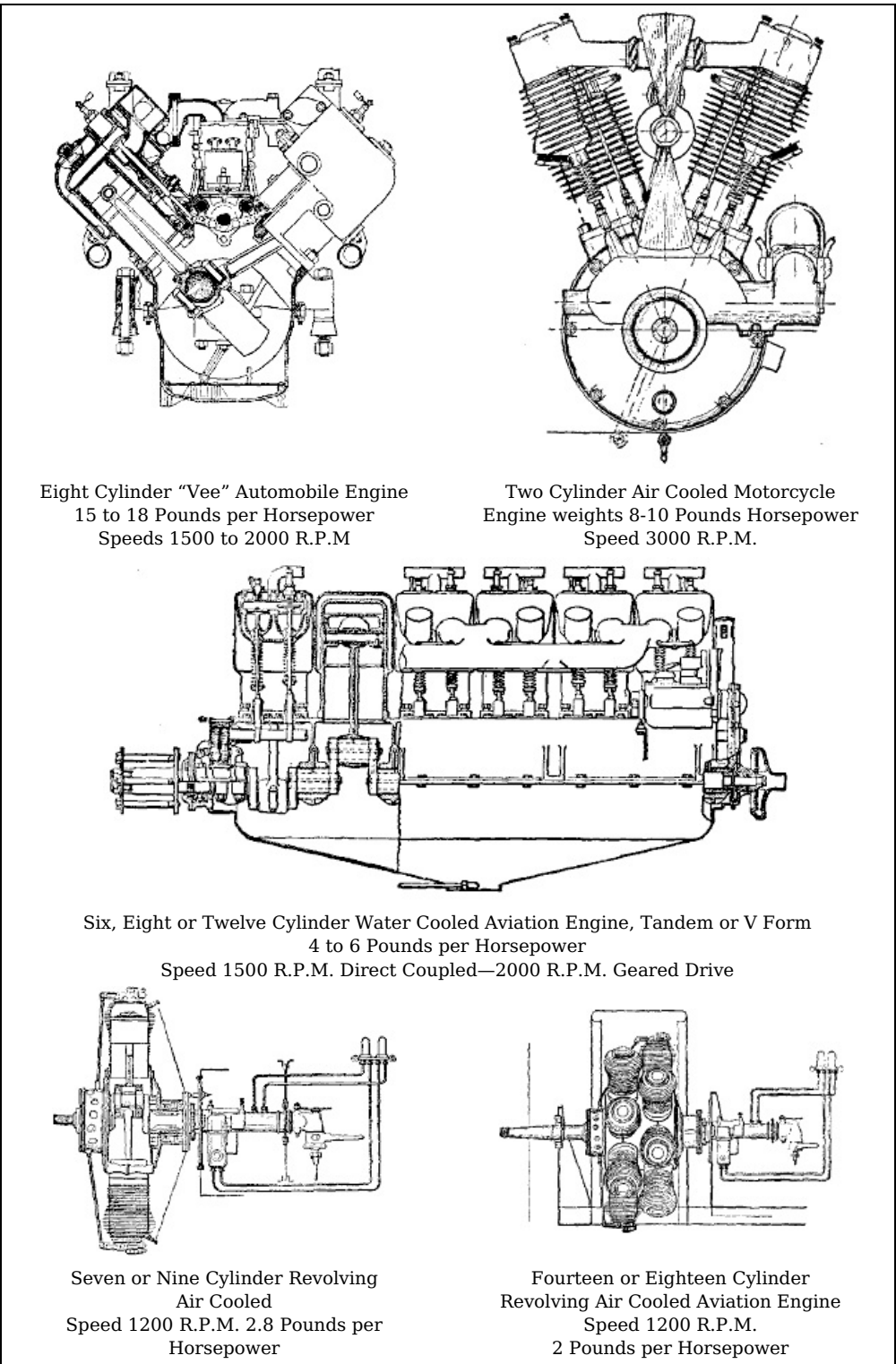
Fig. 3.—Various Forms of Internal Combustion Engines Showing Decrease in Weight to Horse-Power Ratio with Augmenting Speed of Rotation.
