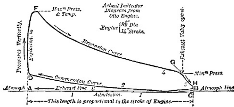
Fig. 13.—Otto Four-Cycle Card.
