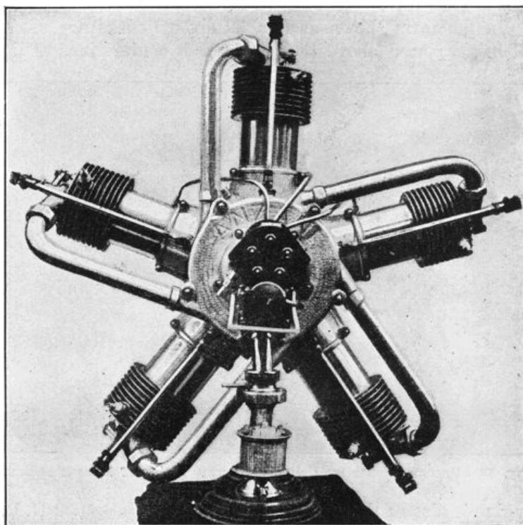
Fig. 38.—Anzani 40-50 Horse-Power Five-Cylinder Air Cooled Engine.
