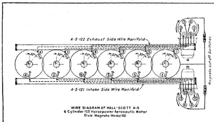
Fig. 70.—Wiring Diagram of Dixie Magneto Installation on Hall-Scott Six-Cylinder 125 Horse-Power Aeronautical Motor.
