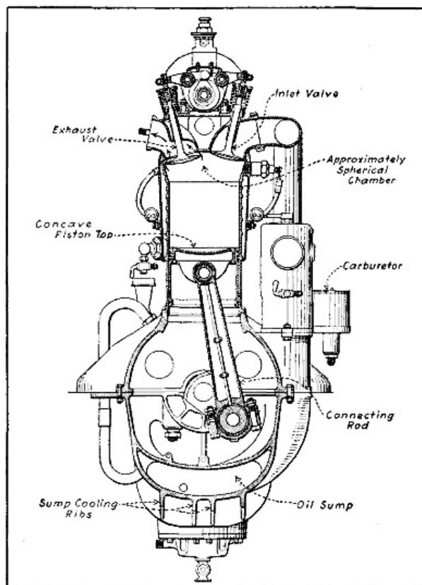
Fig. 20.—Mercedes Aviation Engine Cylinder Section Showing Approximately Spherical
