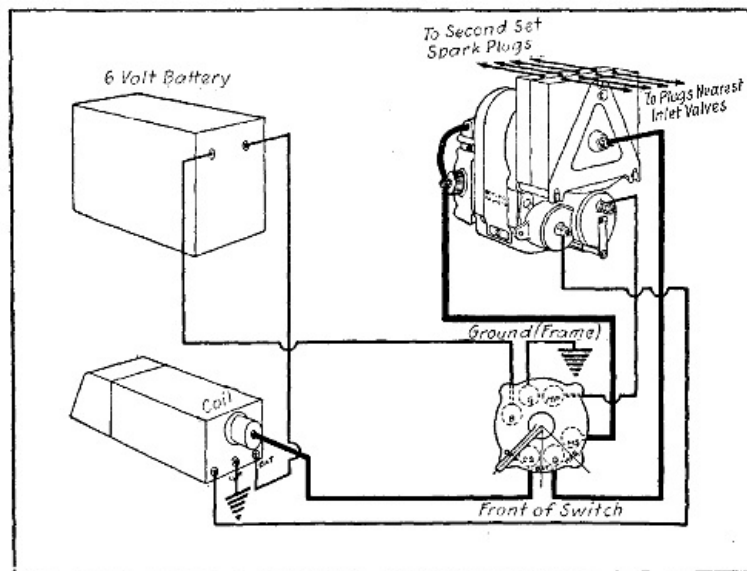
Fig. 61.—Berling Two-Spark Dual Ignition System.
