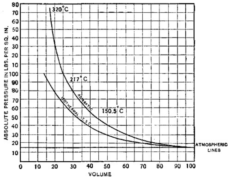
Fig. 11.—Diagram Isothermal and Adiabatic Lines.
