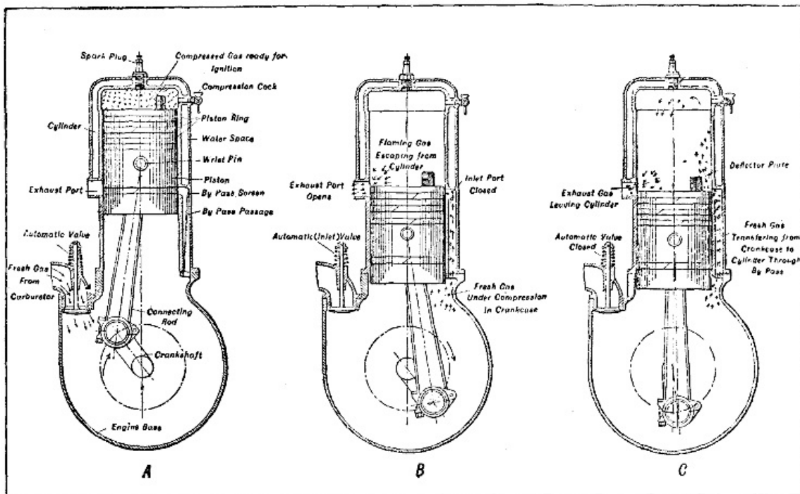
Fig. 8.—Showing Two-port, Two-cycle Engine Operation.
