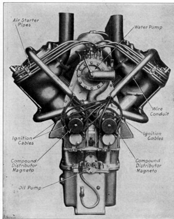
Fig. 71.—How Magneto Ignition is Installed on Thomas-Morse 135 Horse-Power Motor.
