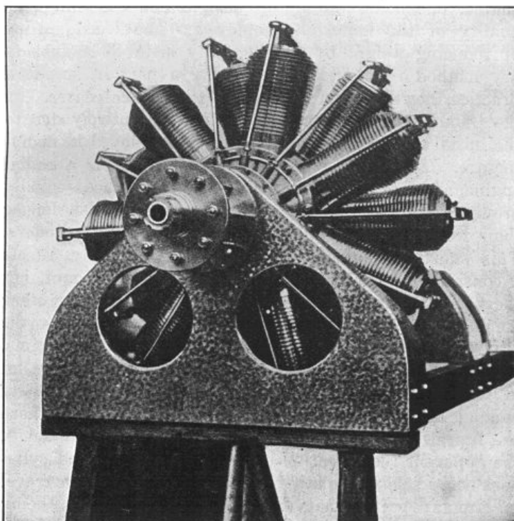
Fig. 40.—The Gnome Fourteen-Cylinder Revolving Motor.
