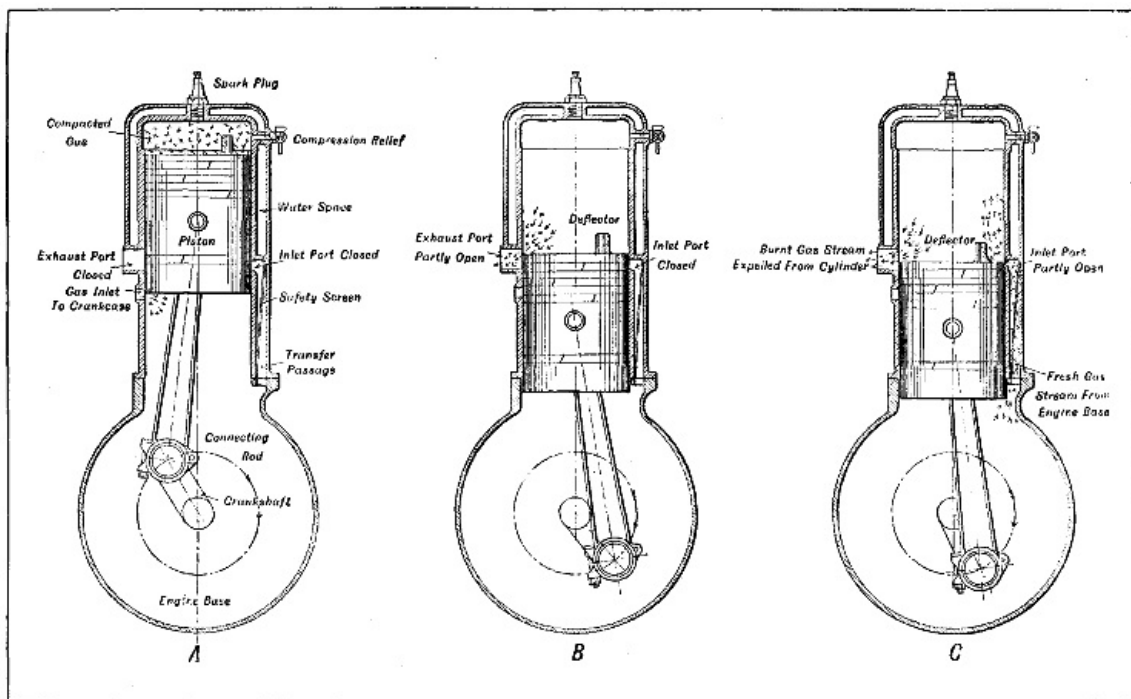
Fig. 9.—Defining Three-port, Two-cycle Engine Action.
