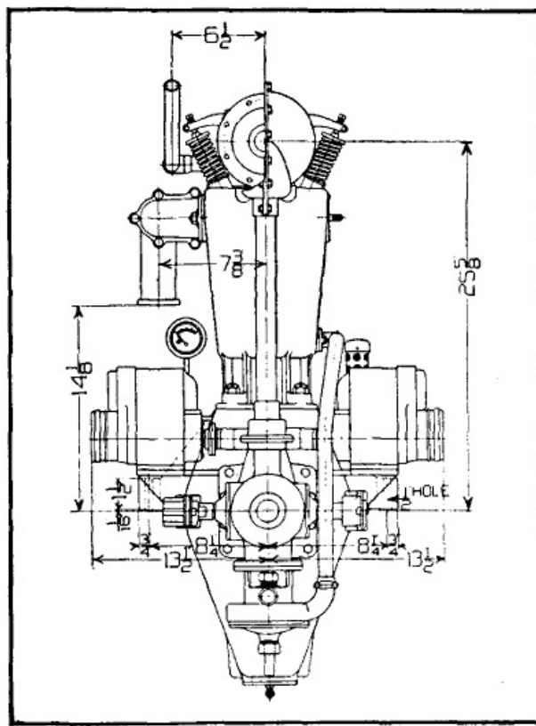
Fig. 238.—Dimensioned End Elevation of Wisconsin Six Motor.
