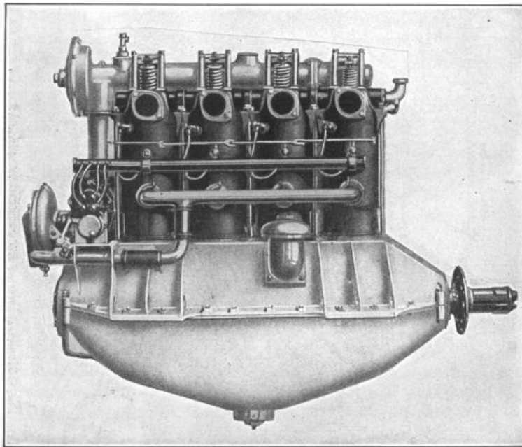
Fig. 33.—The Hall-Scott Four-Cylinder 100 Horse-Power Aviation Motor.
