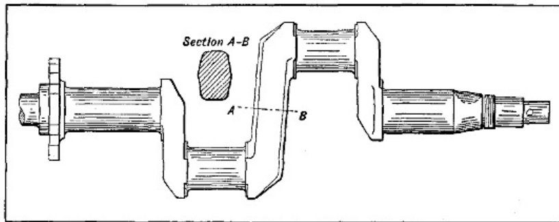
Fig. 136.—Showing Form of Crank-Shaft for Twin-Cylinder Opposed Power Plant.
