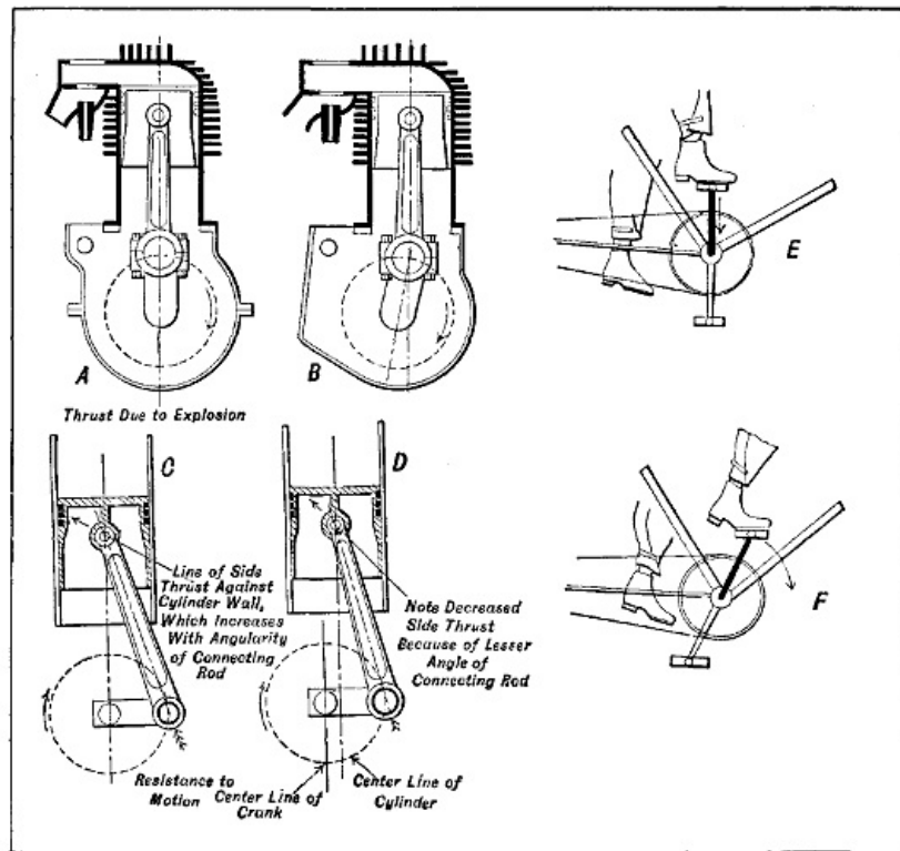
Fig. 91.—Diagrams Demonstrating Advantages of Offset Crank-Shaft Construction.
