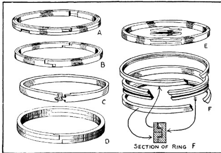
Fig. 125.—Leak-Proof and Other Compound Piston Rings.
