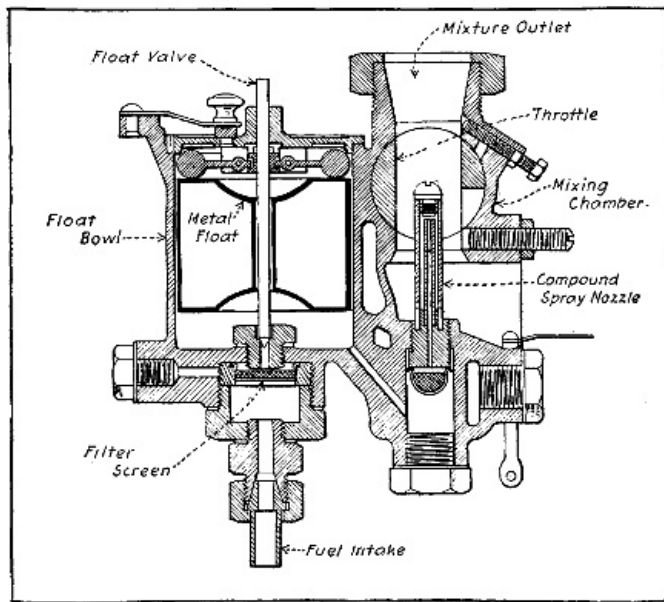
Fig. 46.—The Claudel Carburetor.
