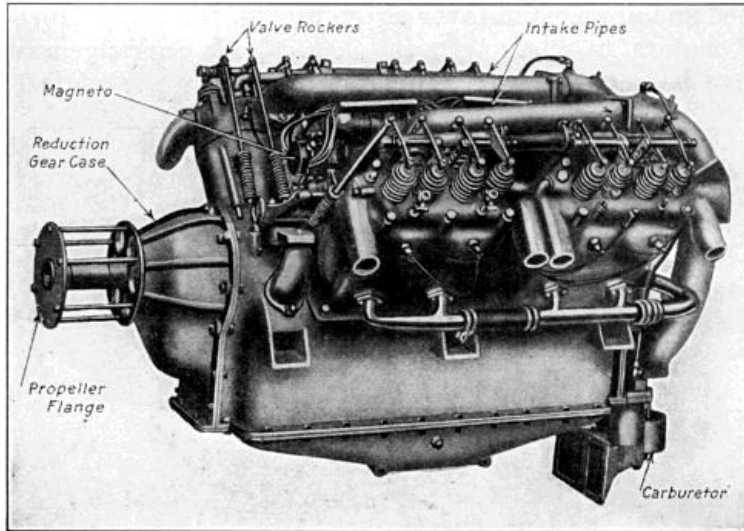
Fig. 37.—The Sturtevant Eight-Cylinder, High Speed Aviation Motor.
