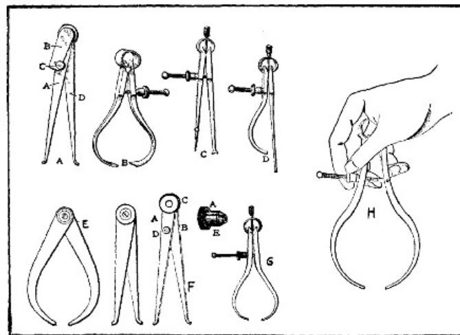
Fig. 174.—Common Forms of Inside and Outside Calipers.
