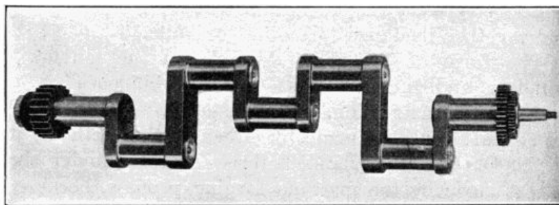
Fig. 137.—Crank-Shaft of Thomas-Morse Eight-Cylinder Vee Engine.
