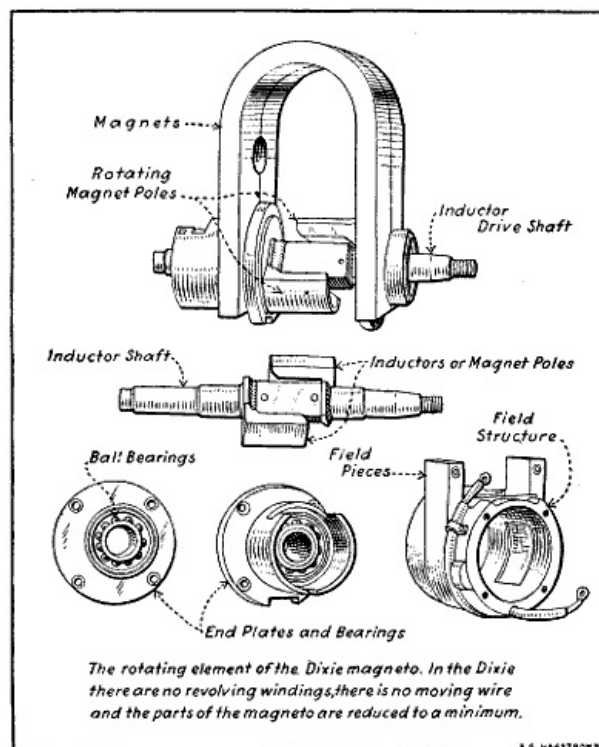
Fig. 68.—The Rotating Elements of the Dixie Magneto.
