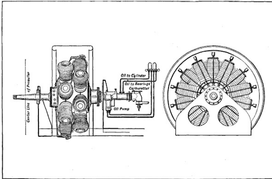
Fig. 203.—The Gnome Fourteen-Cylinder 100 Horse-Power Aviation Engine.
