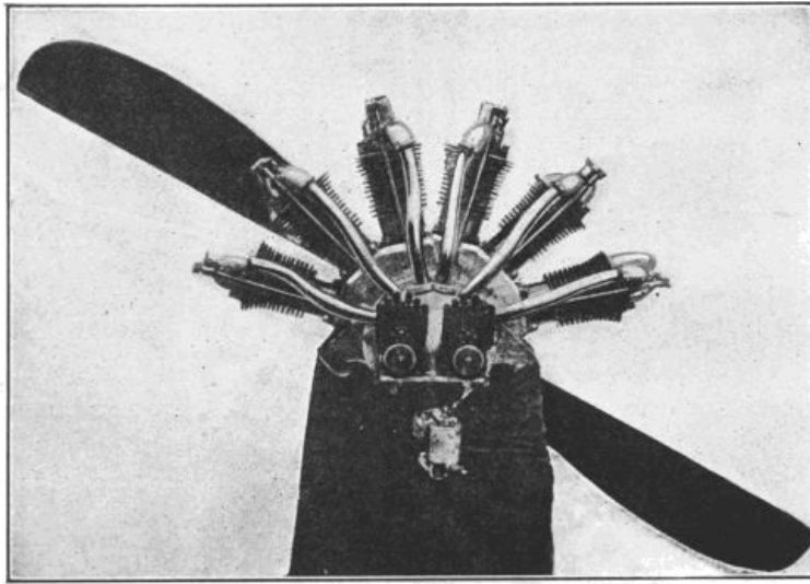
Fig. 39.—Unconventional Six-Cylinder Aircraft Motor of Masson Design.
