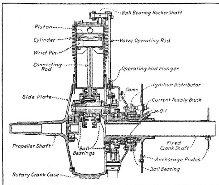
Fig. 216.—Part Sectional Views of Le Rhone Rotary Cylinder Engine, Showing Method of Cylinder Retention, Valve Operation and Novel Crank Disc Assembly.
