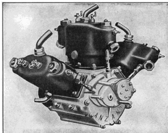
Fig. 191.—The Anzani Six-Cylinder Water-Cooled Aviation Engine.
