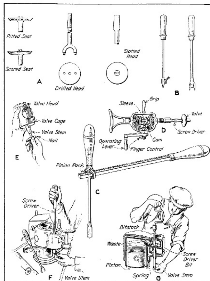
Fig. 184.—Tools and Processes Utilized in Valve Grinding.
