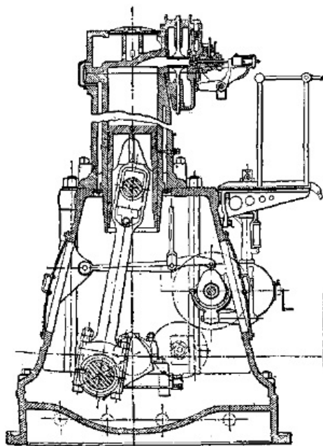
Stationary Diesel Engine 450 to 500 Pounds per Horsepower
