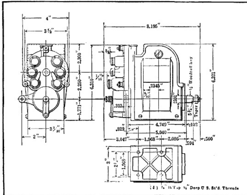
Fig. 67.—Installation Dimensions of Dixie Model 60 Magneto.
