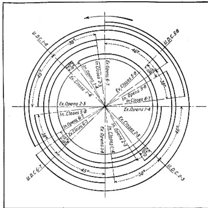
Fig. 110.—Timing Diagram of Typical Eight-Cylinder V Engine.
