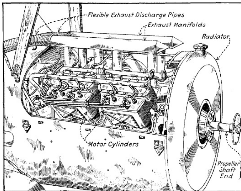
Fig. 147.—Front View of L. W. F. Tractor Biplane Fuselage, Showing Method of Installing Thomas Aeromotor and Method of Disposing of Exhaust Gases.
