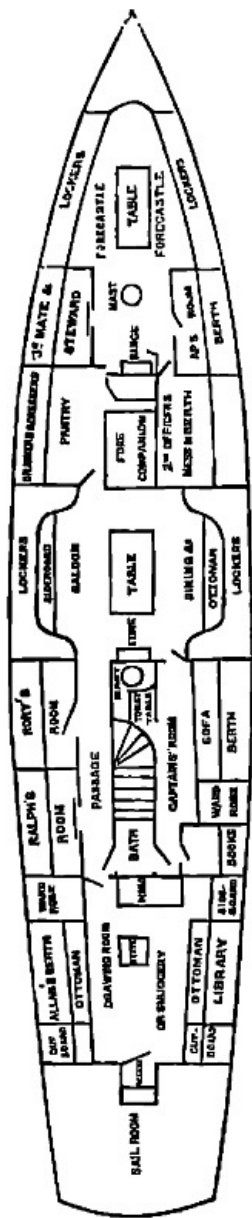
PLAN OF THE "SNOWBIRD."
