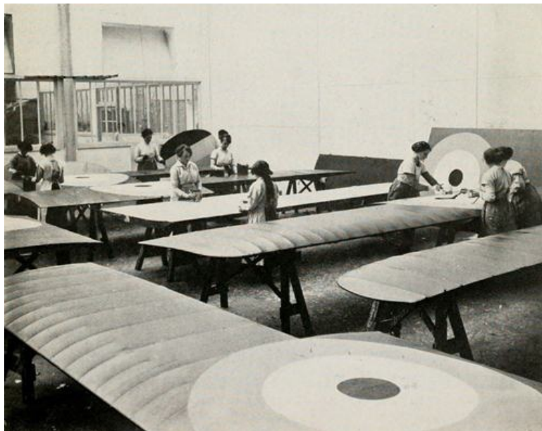
COLOURING AEROPLANE PLANES
