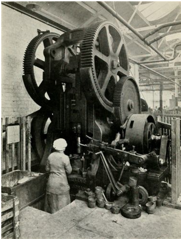
THE MANUFACTURE OF 4.5-INCH CARTRIDGE CASES: OPERATING THE DRAWING PRESS
