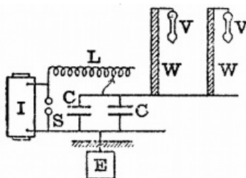
FIG. 22.—SEIBT'S APPARATUS FOR EXHIBITING ELECTRIC RESONANCE. I, induction coil; S, spark gap; CC, condensers; L, variable inductance; E, earth plate; WW, wire spirals; VV, vacuum tubes.
