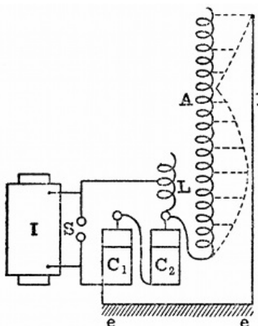
FIG. 11.—HARMONIC OSCILLATIONS IN LONG SOLENOID SHOWN WITH SEIBT'S APPARATUS.
