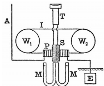
FIG. 18.—MARCONI MAGNETIC
