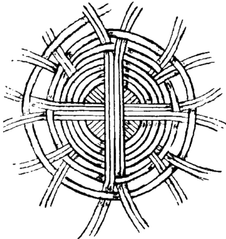
DIAGRAM NO. 11.—SIXTEEN-SPOKE CENTER
