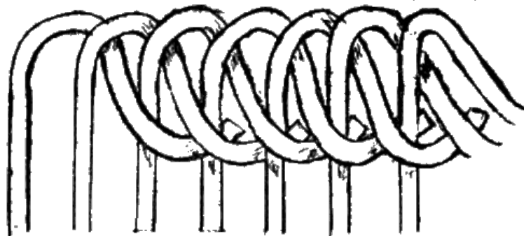
DIAGRAM NO. 17.—CLOSED BORDER NO. 1 (PART 2)
