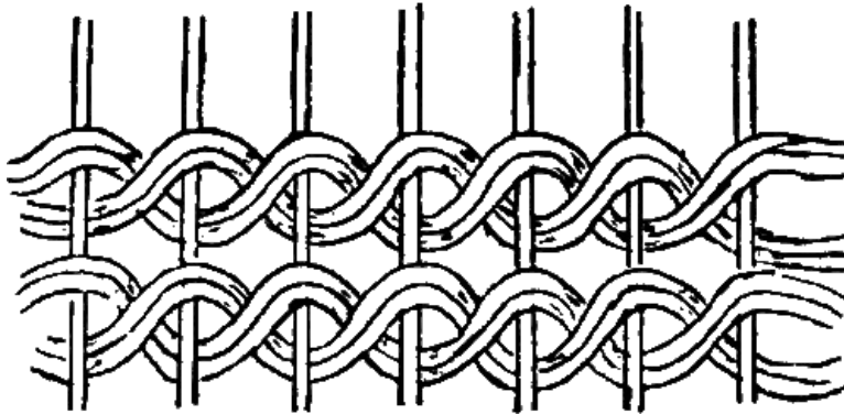
DIAGRAM NO. 4.—DOUBLE PAIRING
