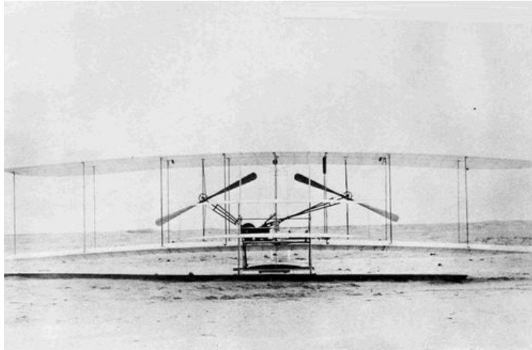
Kitty Hawk Flyer with original Wright engine poised on launching rail at Kill Devil Hill, near Kitty Hawk, North Carolina, 24 November 1903, the month before the Wrights achieved man's first powered and controlled flight in a heavier-than-air craft.
