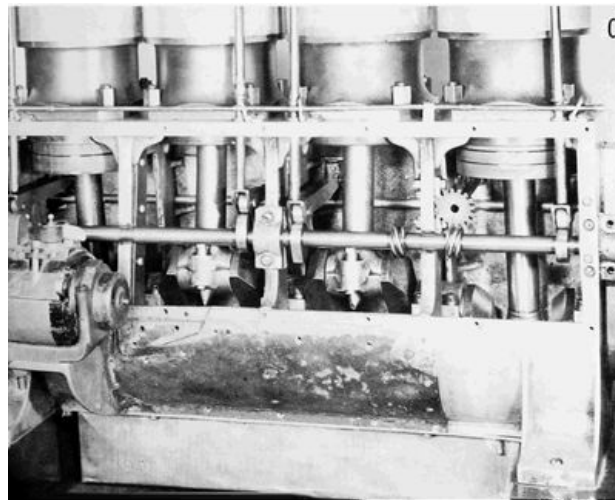
Figure 9. —4-Cylinder vertical engine: a, magneto side; b, valve port side with intake manifold removed; c, flywheel end of engine at Carillon Park Museum, Dayton, Ohio; d, magneto side with crankcase cover removed. (Photos: a, Smithsonian A-3773; b, d, Pratt & Whitney D-15003, 15007; c, by A. L. Rockwell.)
