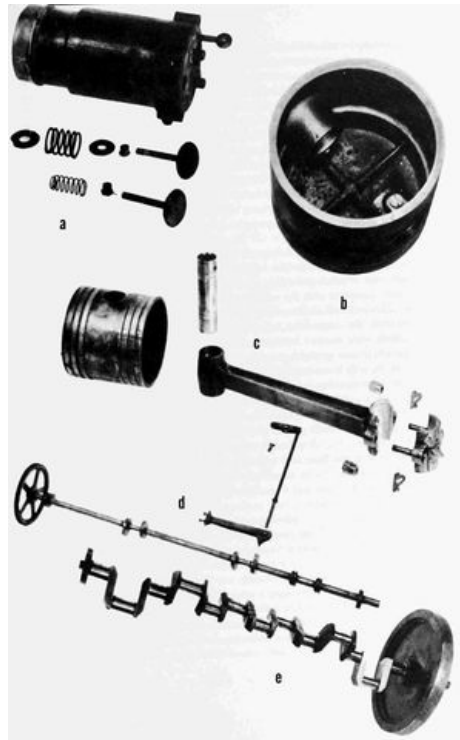
Figure 13.—Original 6-cylinder engine: a, cylinder assembly and valve parts; b, bottom side of piston; c, piston, piston pin and connecting rod; d, valve mechanism; e, crankshaft and flywheel. (Pratt & Whitney photos D-15012, 15017, 15013, 15018, respectively.)
