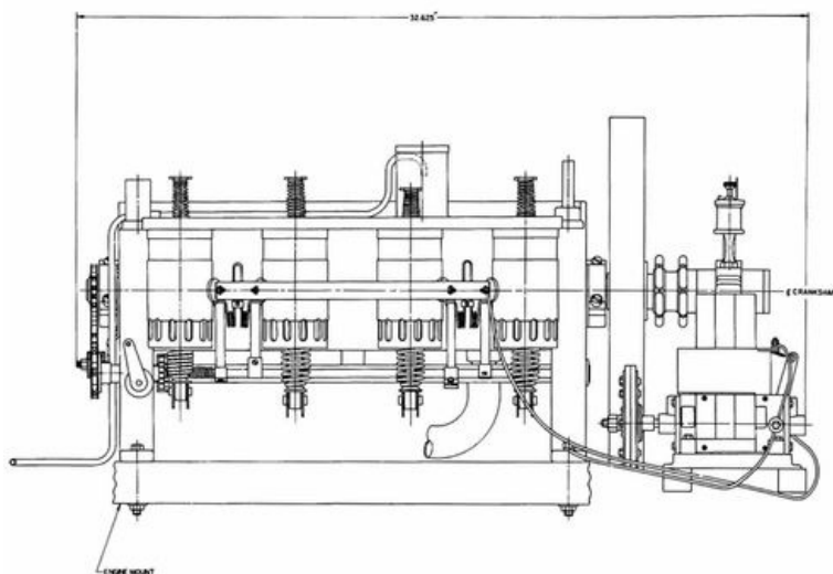
Figure 4.—First flight engine, 1903, left side and rear views, with dimensions. (Drawing courtesy Howell Cheney Technical School.)
