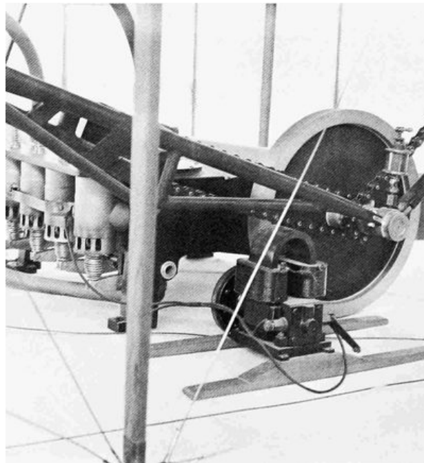
Reproduction of the first engine, built by Pratt & Whitney, as displayed in Wright Brothers National Memorial at Kitty Hawk. Engine is mounted in a reproduction of the Wrights' Flyer built by the National Capital Section of the Institute of the Aeronautical Sciences (now the American Institute of Aeronautics and Astronautics). Engine and plane were donated in 1963 to the National Park Service Cape Hatteras National Seashore.
