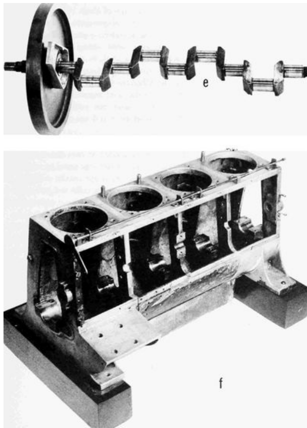
Figure 10. —4-Cylinder vertical engine: a, cylinder assembly with valve mechanism parts; b, cylinder disassembled, and parts; c, pistons and connecting rods; d, bottom side of piston; e, crankshaft, flywheel and crankcase end closure; f, crankcase, with compression release parts. (Pratt & Whitney photos D-14996, 15001, 14998, 14994, 14999, 14989, respectively.)
