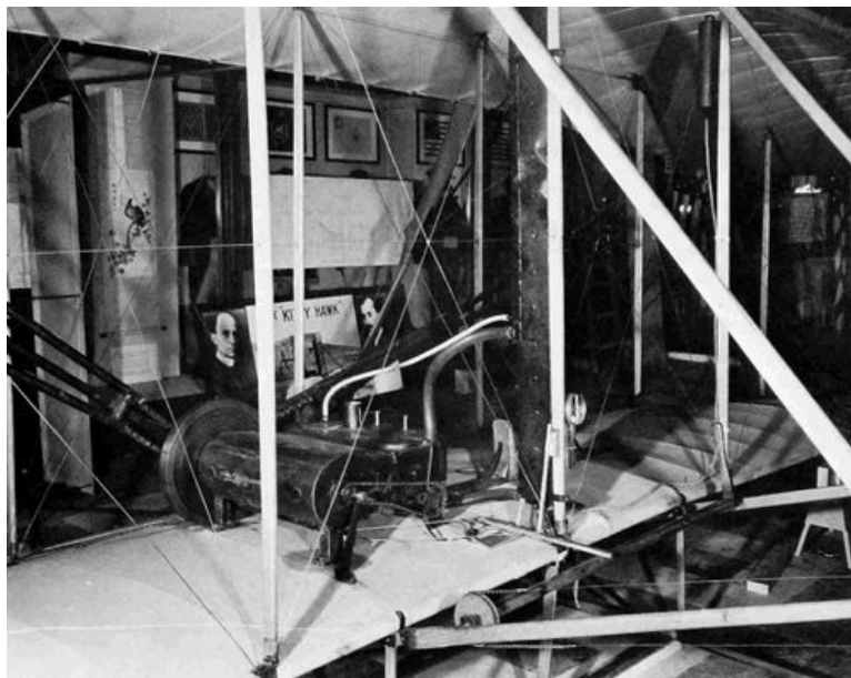
Figure 3. —First flight engine, 1903, installed in the Kitty Hawk airplane, as exhibited in the Science Museum. (Photo courtesy the Science Museum, London.)
