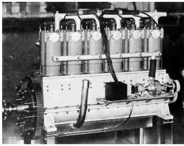
Figure 15.—6-Cylinder 6-70 engine, incorporating flexible flywheel drive, exhaust side. (Smithsonian photo A-54381.)
