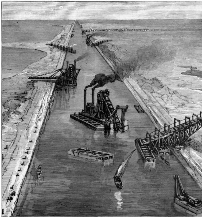
THE SUEZ CANAL: DREDGES AT WORK.
