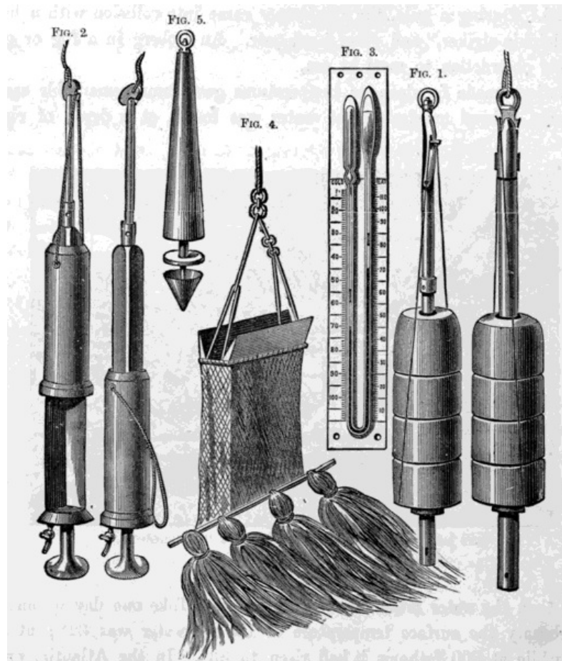
DREDGING IMPLEMENTS USED BY THE "CHALLENGER."
