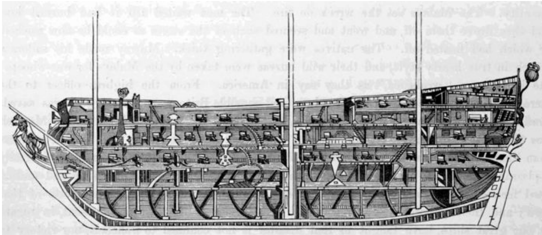
SECTION OF A FIRST-CLASS MAN-OF-WAR.
