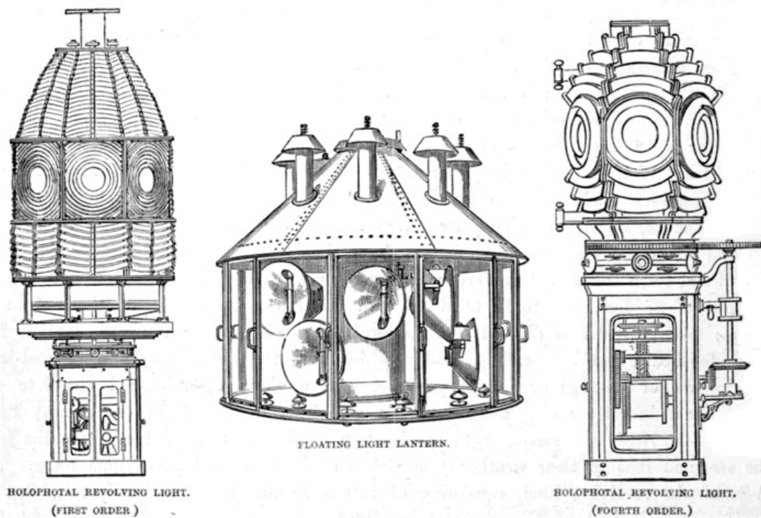
REVOLVING LIGHT APPARATUS. (From Drawings supplied by Messrs. W. Wilkins & Co.)
