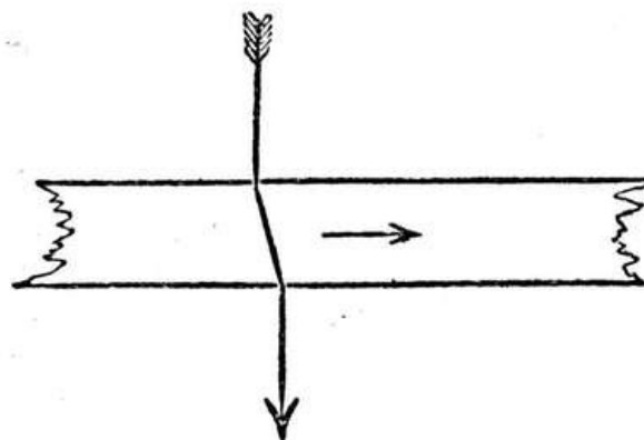
Fig. 4. Ray through a Moving Stratum.
