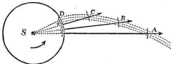
Fig. 3. Beam from a Revolving Lighthouse.
