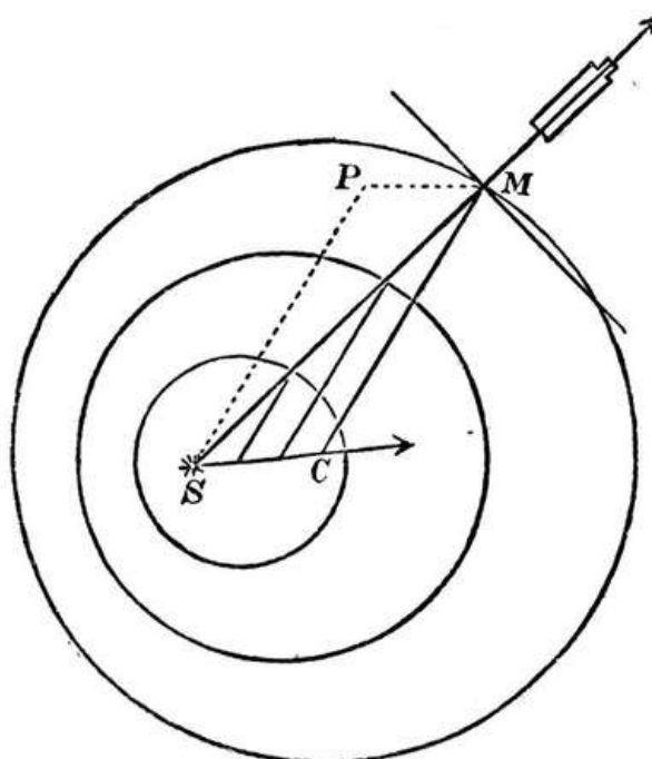
Fig. 5. Successive Wave Fronts in a Moving Medium.
