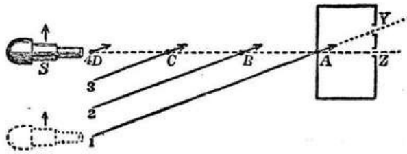
Fig. 1. Shots or Disturbances with Momentum from a Moving Gun.
