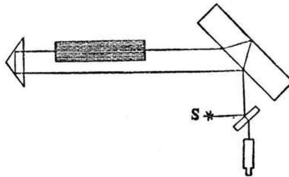
Fig. 9. Arrangement of Mascart and Jamin.
