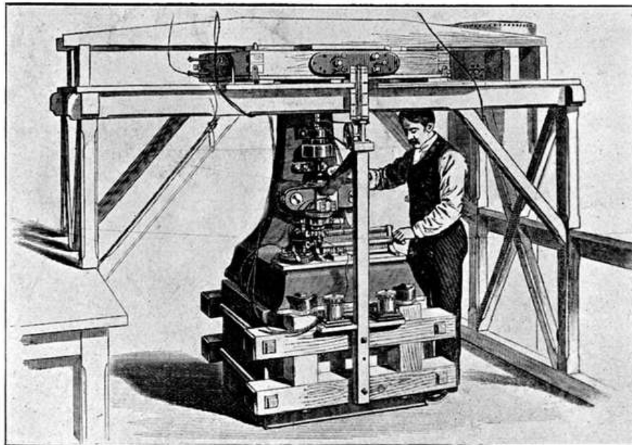
Fig. 15. View of Ether machine complete and in action.
