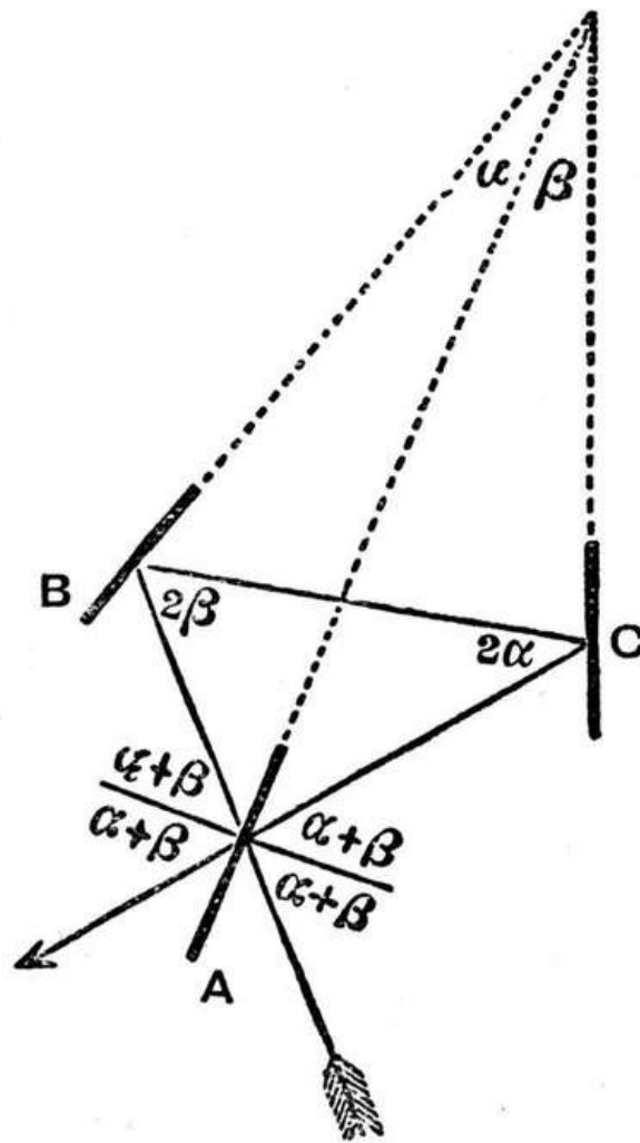
Fig. 7. Plan of Interference Kaleidoscope with three mirrors.
