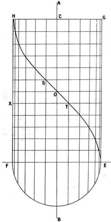
FIG. 30.—PROPELLER DESIGN. One quarter scale. Diameter 14 in. Pitch 52 in. Angle at tip 44^\circ .
