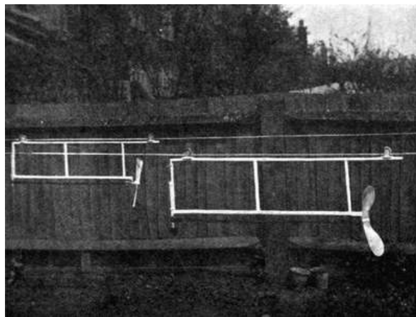
FIG. 34.—THE AUTHOR'S PROPELLER TESTING APPARATUS.
