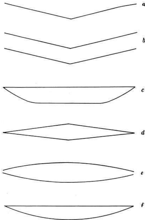
FIG. 12.—VARIOUS FORMS OF DIHEDRALS.
