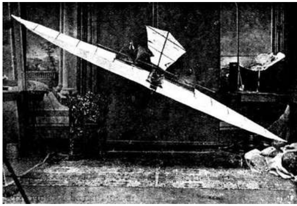
FIG. 5.—THE STRINGFELLOW MODEL MONOPLANE OF 1848.
