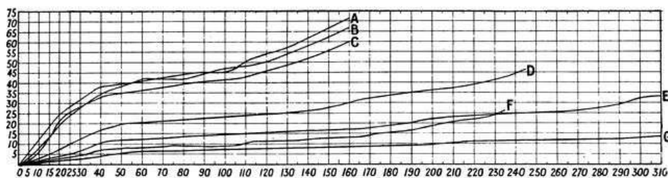
FIG. 16.—TORQUE GRAPHS OF RUBBER MOTORS.
