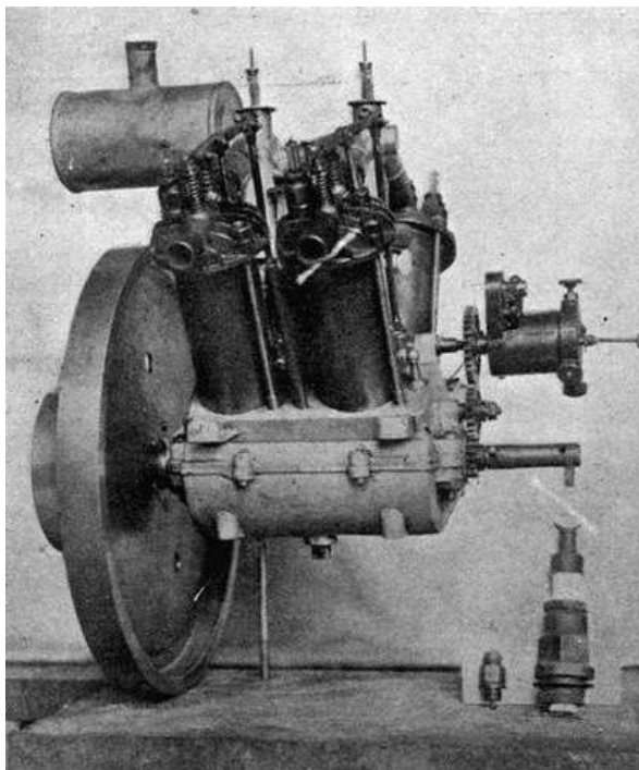
FIG. 20.—MR. STANGER'S MODEL PETROL ENGINE.
