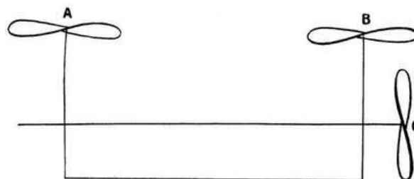
FIG. 51.—INCORRECT WAY OF ARRANGING SCREWS.
