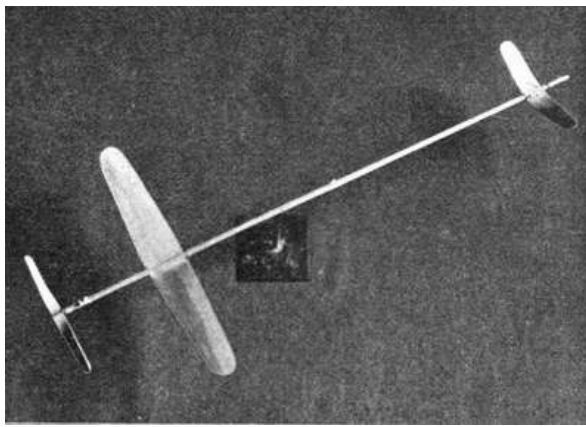
FIG. 49B.—MR. T.W.K. CLARKE'S 1 OZ. MODEL. Showing the position of C. of G., or point of support.
