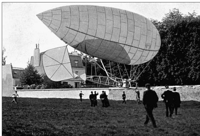
"No. 9" JUMPING MY WALL
