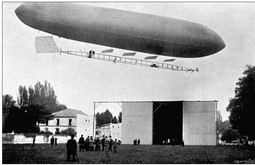
"No. 10" WITHOUT PASSENGER KEEL
