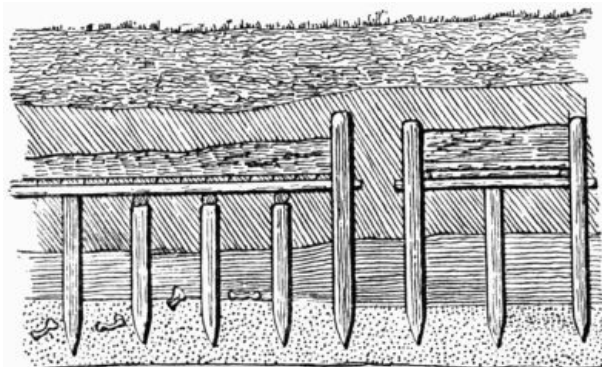
Fig. 151.—Vertical Section of the Marniera of Castione.
