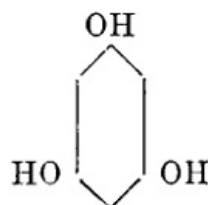
Phloroglucin.
