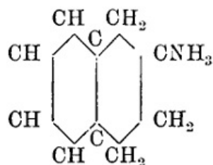
Acyclic tetrahydro- \alpha -Naphthylamine.
