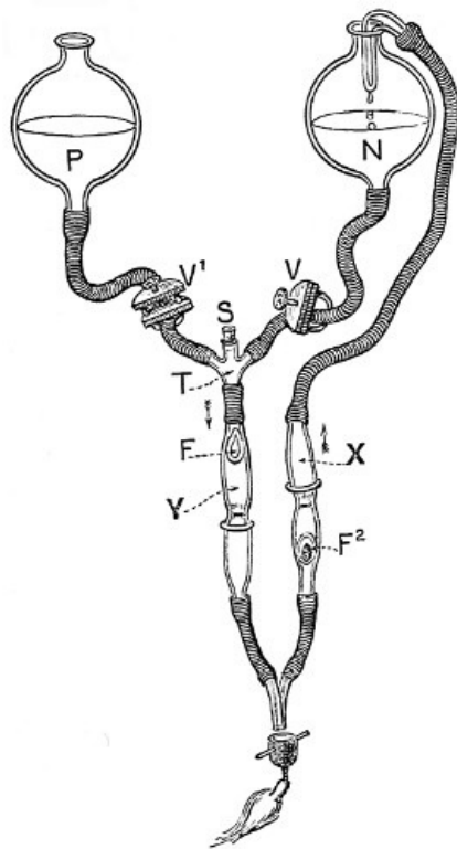
Williams' Apparatus.
