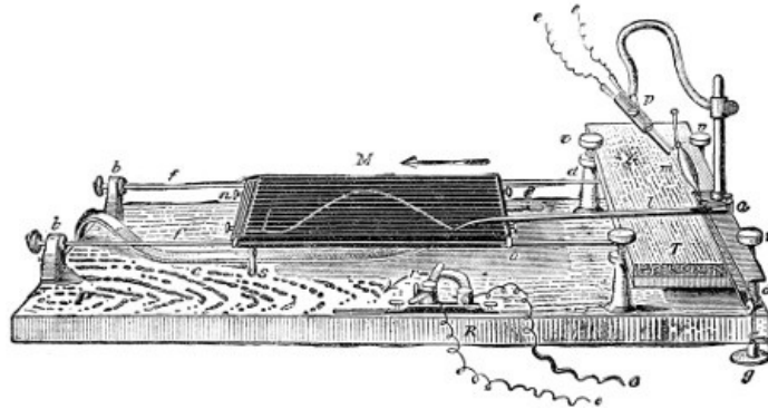
Fig. 118.—Horizontal Myograph of Frédéricq. M , Glass plate, moving on the guides f, f, l , Lever; m , Muscle; p, e, e , Electrodes; T , Cork plate; a , Counterpoise to lever; R , Key in primary circuit.
