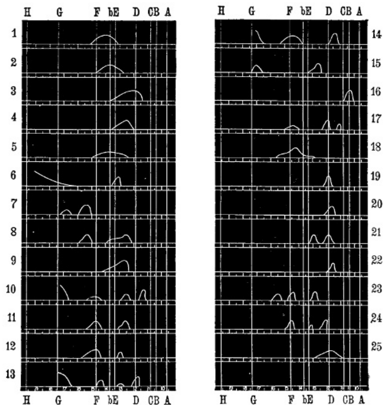
NOTES TO CURVES INDICATING ABSORPTION BANDS.
