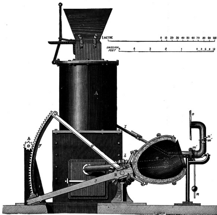
APPARATUS FOR MECHANICAL PUDDLING.
