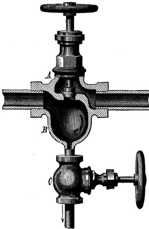
SAUNDERS' STEAM VALVE.
