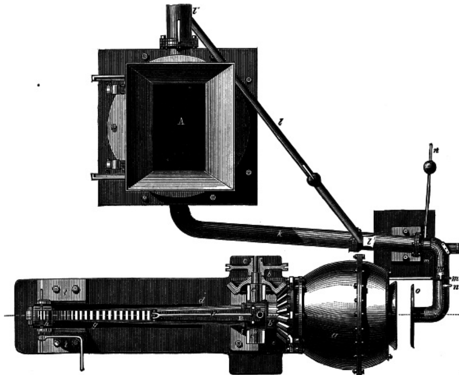
APPARATUS FOR MECHANICAL PUDDLING.
