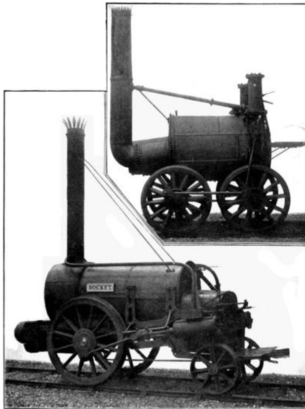
THE FAMOUS LOCOMOTIVES "ROCKET" AND "SANS PAREIL."
