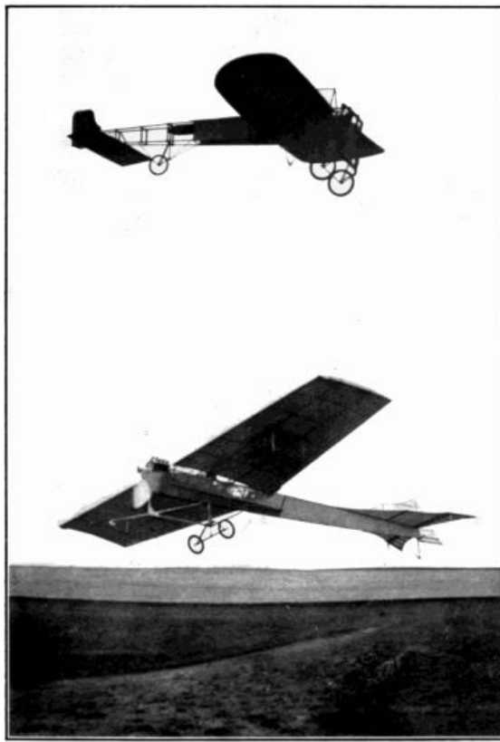
THE MONOPLANES OF BLÉRIOT AND LATHAM.
