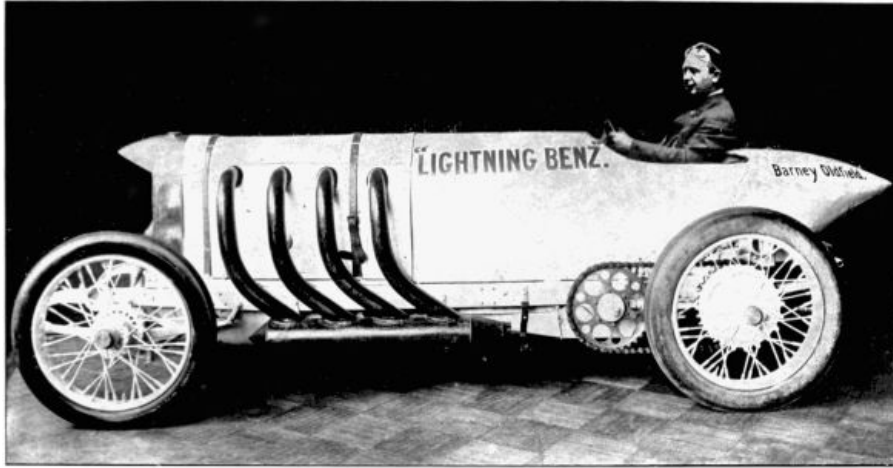
A RACING AUTOMOBILE.
