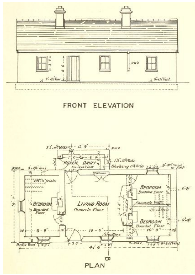
INTERIOR AND EXTERIOR OF ONE STORY COTTAGES ERECTED BY THE CONGESTED DISTRICTS BOARD
