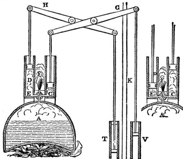
Leupold's Engine
