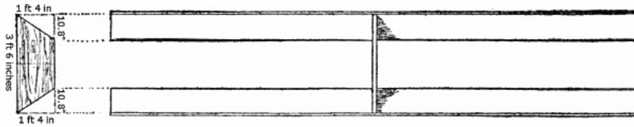
Fig. 111.—Parts of dory.
