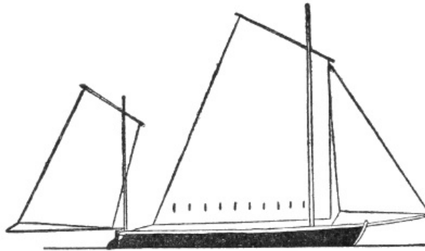
Fig. 171.—Lug rig with jigger and jib.
