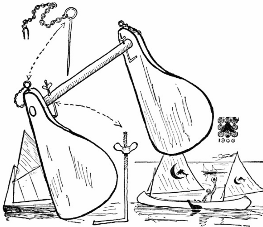
Fig. 140.—Lee-board. Fig. 140a.—Bolt and thumb-screw.
