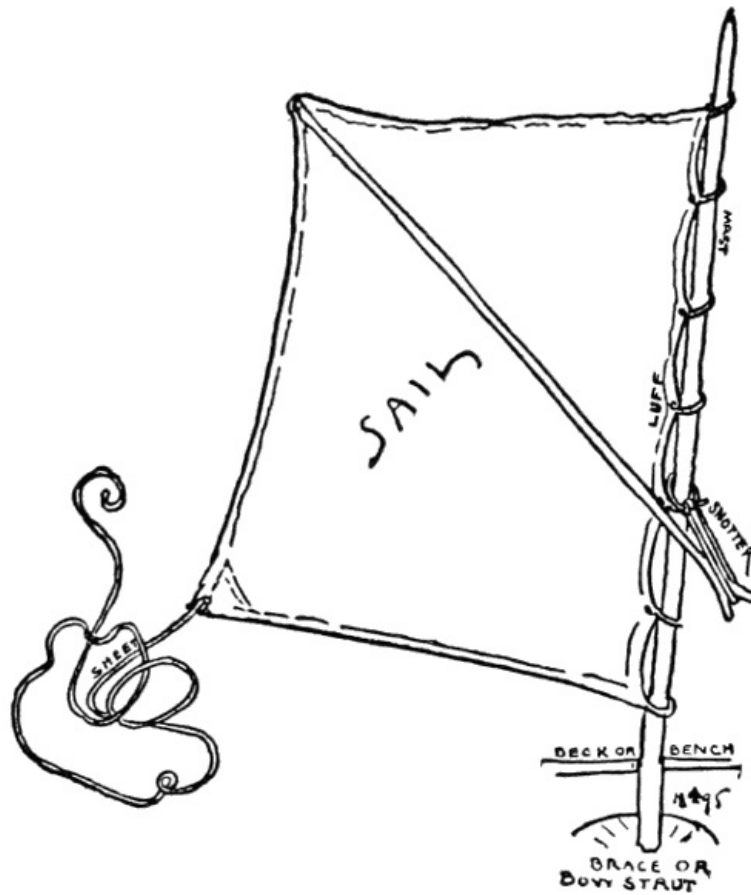
Fig. 126.—Sail and sheet.
