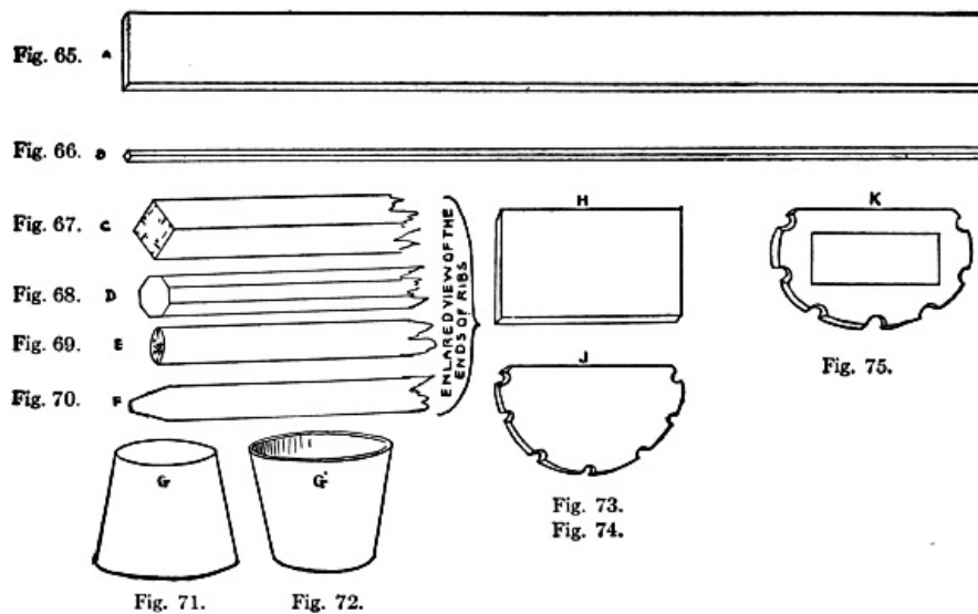
PARTS OF THE UMBRELLA CANOE.
