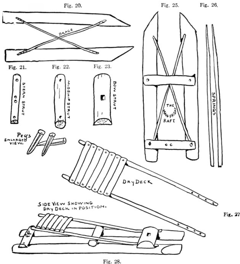
20.—Logs in place with braces. Figs. 21, 22, and 23.—Struts. Fig. 24.—Pegs. Fig. 25.—Raft with middle and stern strut in place. Fig. 26.—Springs for dry deck. Fig. 27.—Dry deck. Fig. 28.—Dry deck in place
