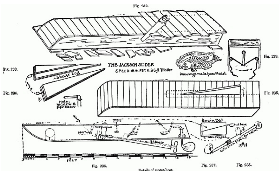
Details of motor-boat.
