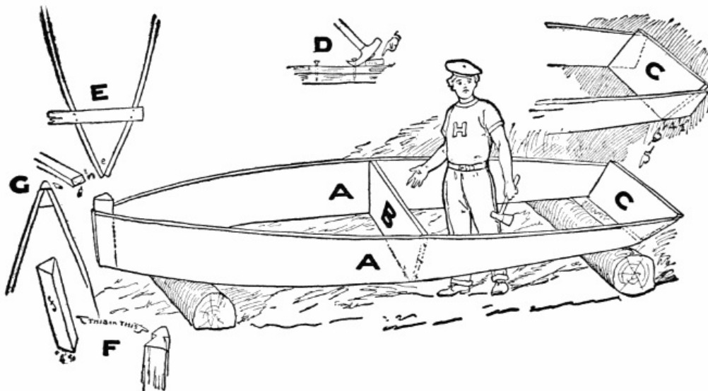
Fig. 195.—Details of the boat.
