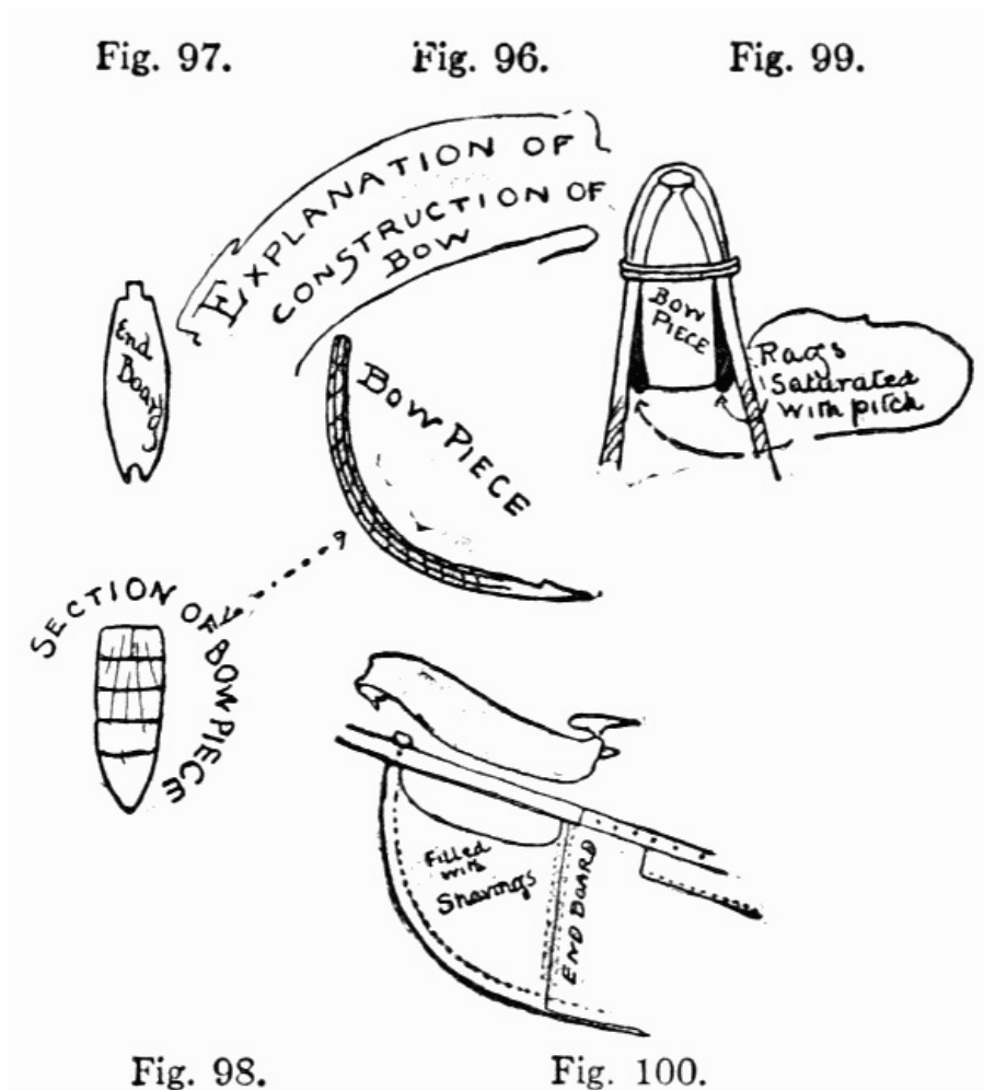
Figs. 97-100.—Show details of canoe bow.
