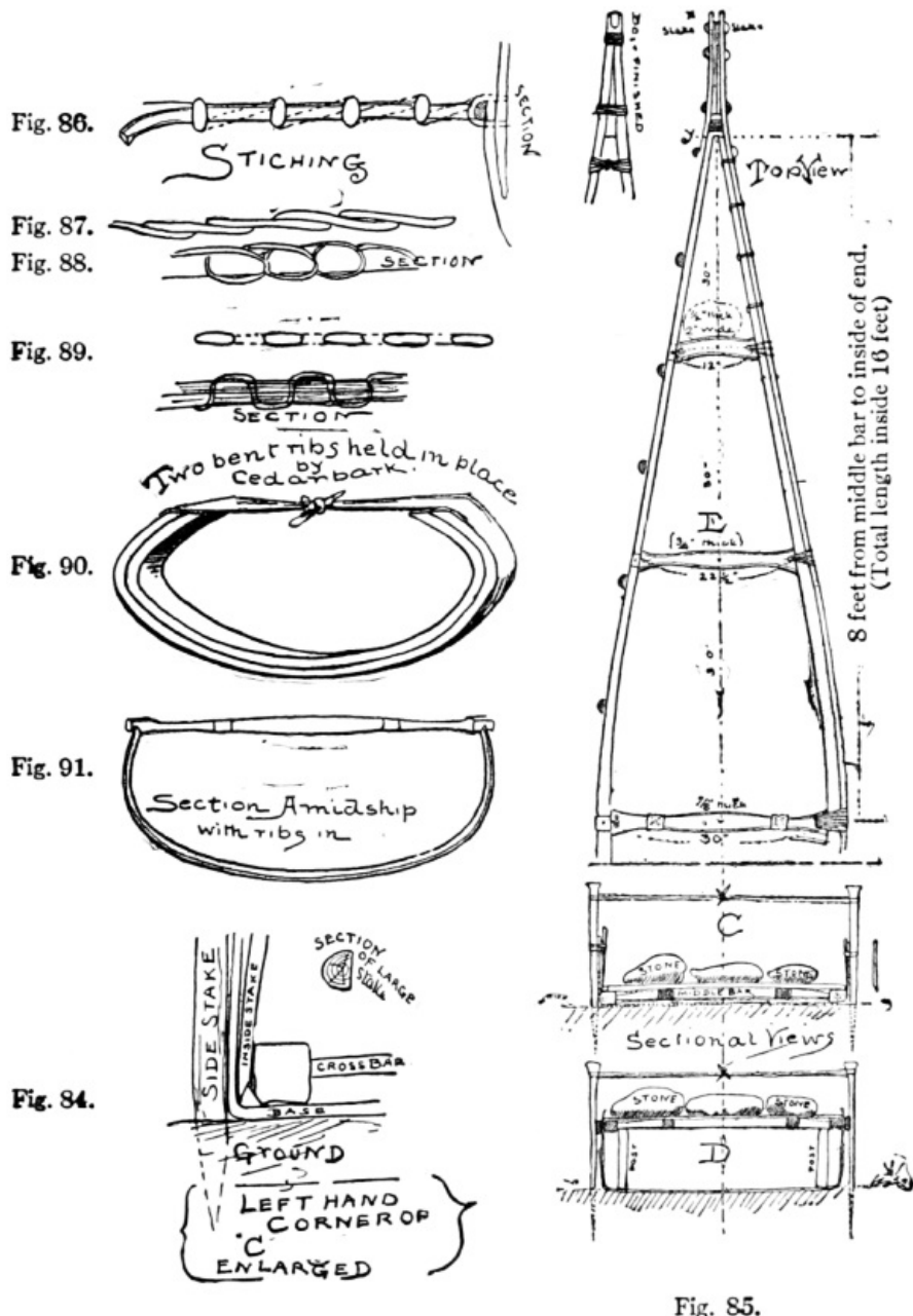
Details of sticking and framework of canoe.
