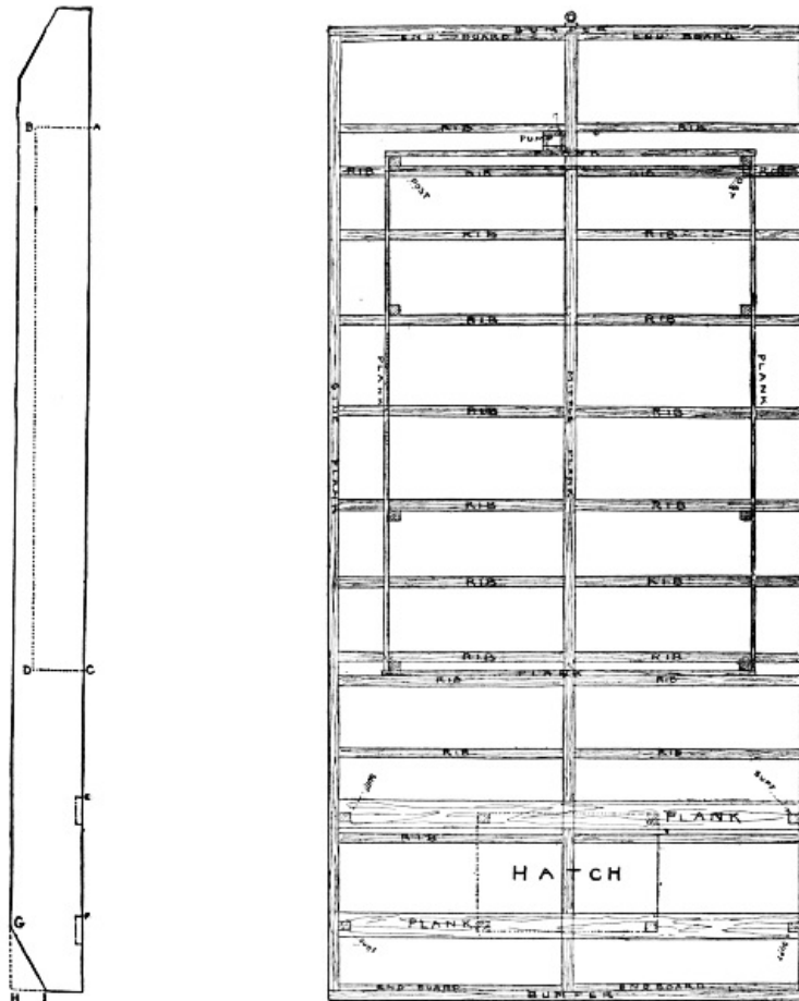
Fig. 220.—Center board of house boat. Fig. 221.—Plan of house boat.
