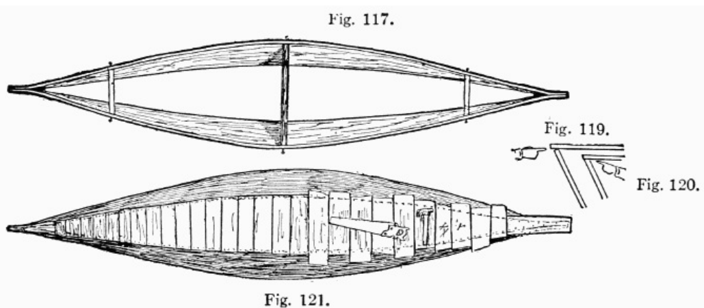
Top view with sides in place, also reversed view showing how bottom boards are laid.
