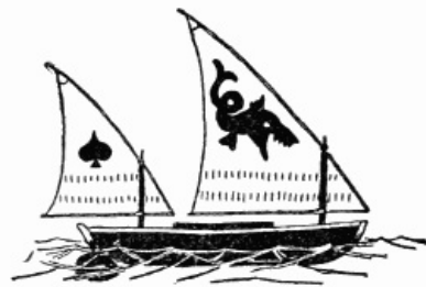
Fig. 175.—The lateen rig with dandy.
