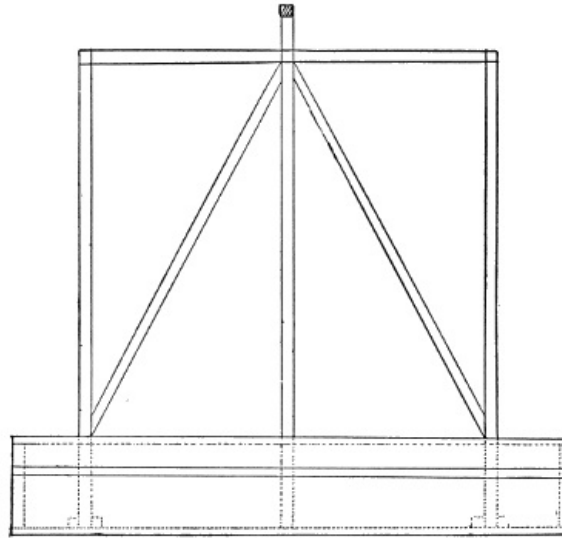
Fig. 223.—End view.
