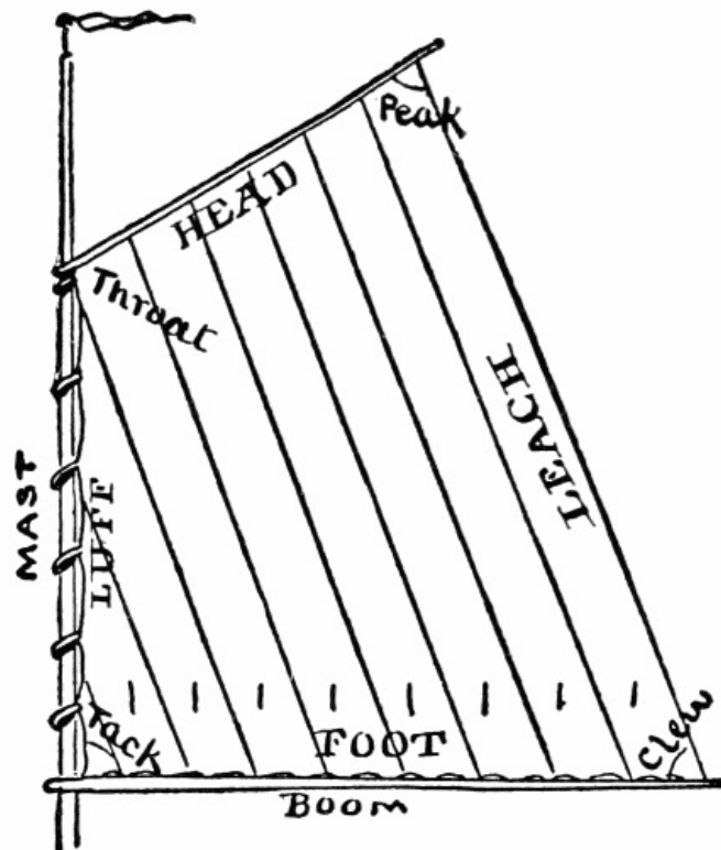
Fig. 127.—Parts of sail.
