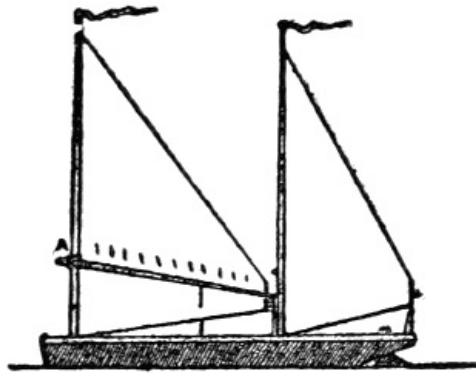
Fig. 164.—Sharpie with sprit and club leg-of-mutton sails.
