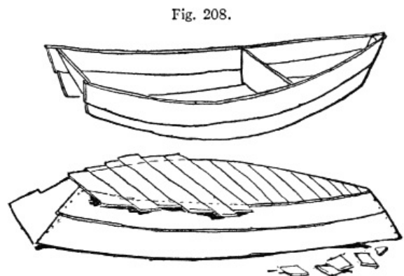
Diagrams showing the construction of the rough-and-ready.
