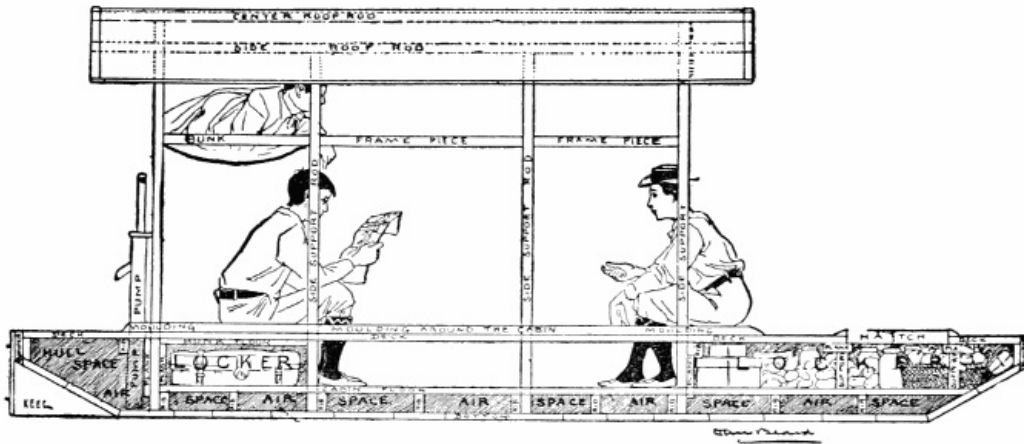
Fig. 222.—Cross-section of boat
