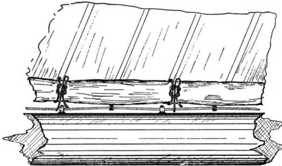
THE PROPER WAY TO TIE REEF-POINTS
