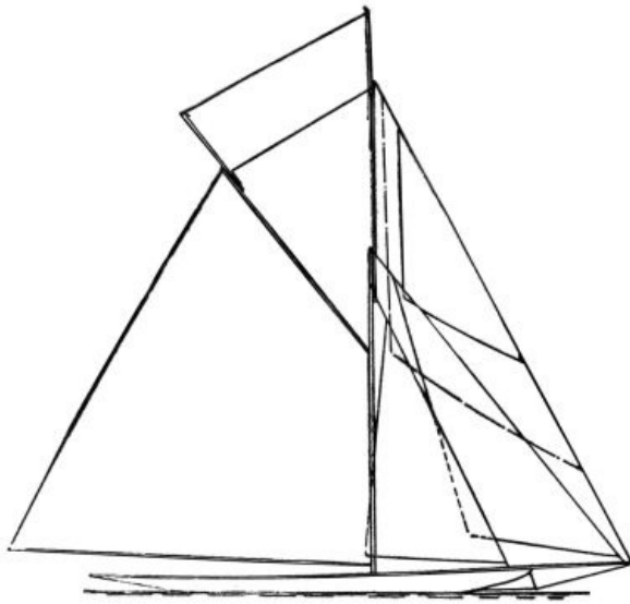
CUTTER RIG
