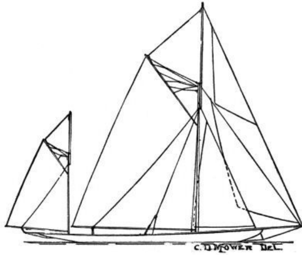
YAWL RIGS
