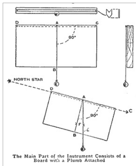
The Main Part of the Instrument Consists of a Board with a Plumb Attached
