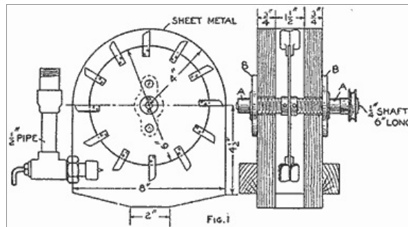
Details of the Water Wheel (Fig. 1)
