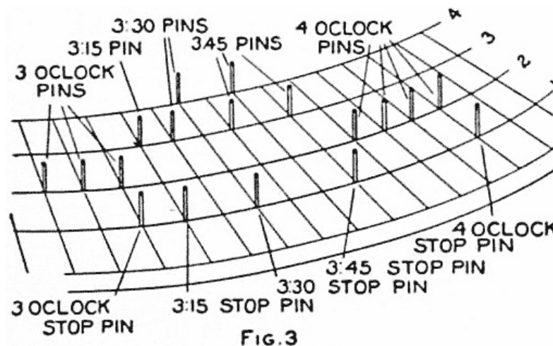
The Pins are Accurately Set in Four Circular Lines and on Radial Lines (Fig. 3)
