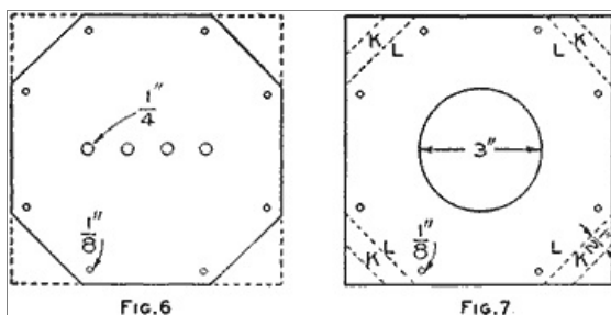
Detail of the Upper and Lower End Plates That are Used in Making a Rheostat (Fig. 6, Fig. 7)
