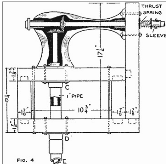
The Supporting Standard Holds the Machine Head with the Wheel and the Vane on an Axis (Fig. 4)
