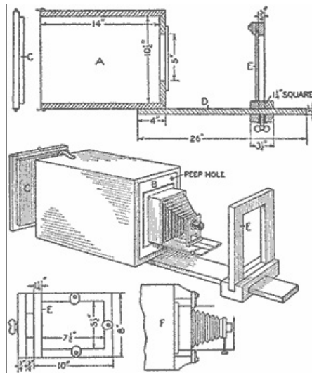
Details of Construction and Camera Complete
