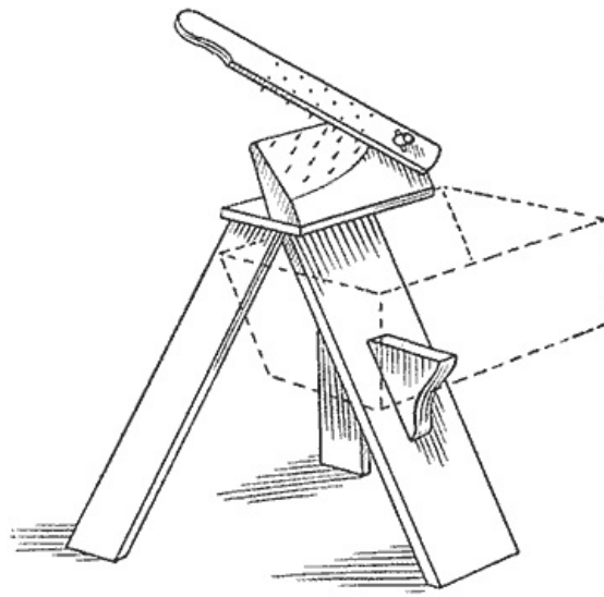
The Projecting Nail Heads in the Block and Lever, as They Pass, Shell the Corn
