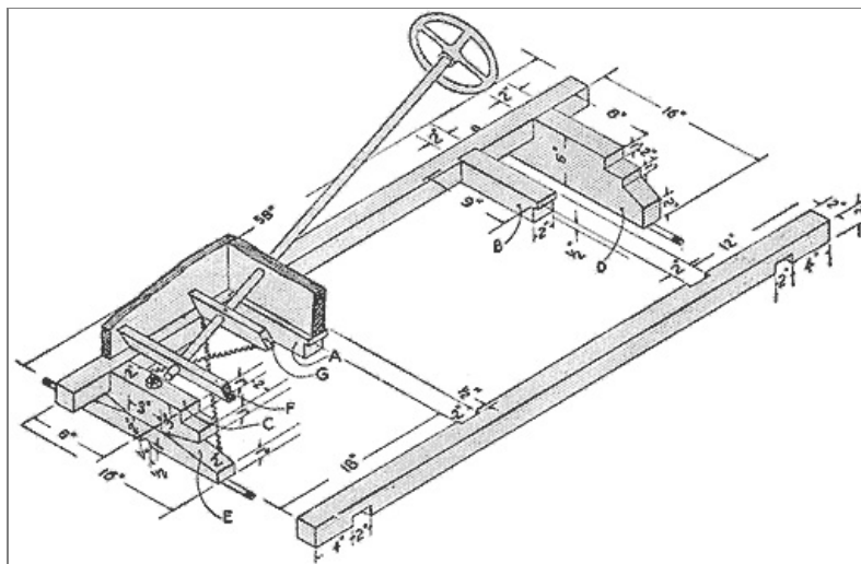
The Entire Chassis was Made of Cypress Wood, All Cars of the Same Length and Width, the Hoods and Seats Being the Only Parts Optional in Size and Shape for the Builder
