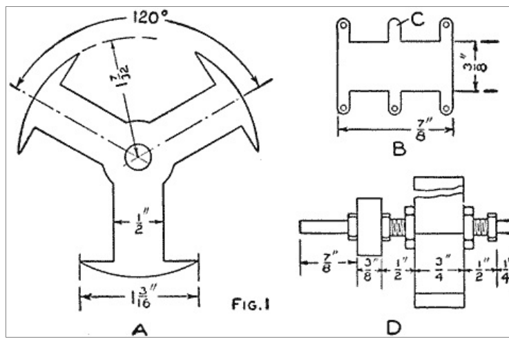
Details of the Armature Laminations and the Commutator Segments, and the Method of Mounting Armature Core and Commutator (Fig. 1)
