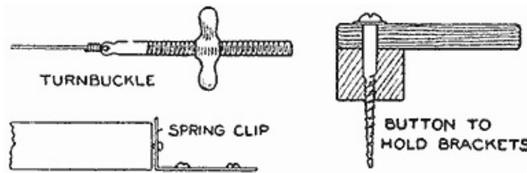
Detail of the Turnbuckle, Button to Hold the Brackets, and the Spring Clip for Holding the Legs on the Side of the Box
