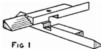
The Hub Consists of Two Parts, Each Having Four Arms for Holding the Blades (Fig. 1)
