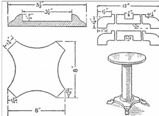
The Pedestal can be Made of a Wood Suitable for Finishing to Match Other Furniture
