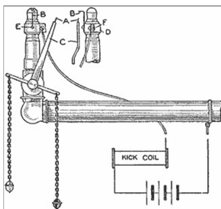
The Igniting Points as They are Attached to a Gas Burner to Work Automatically
