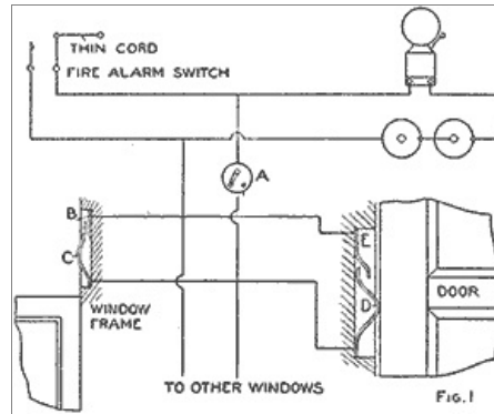
Connections and Wiring Diagram Showing an Open-Circuit Fire and Burglar Alarm (Fig. 1)
