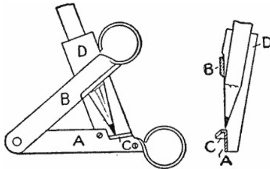
A Pencil Sharpener That will Make a Point without Breaking the Lead
