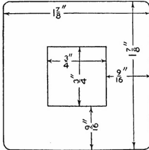
Fig. 14—Insulating Washer
