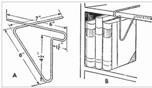
The Shape of the Wire Makes It Easily Applicable to Any Open Bookshelf
