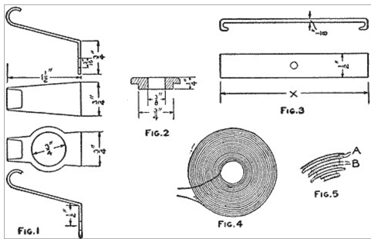
Detail of the Parts for the Construction of an Electric Shaving Mug. The Heating of Sufficient Water for a Shave can be Accomplished at a Nominal Cost (Fig. 1, Fig. 2, Fig. 3, Fig. 4, Fig. 5)
