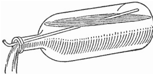
The Vacuum Caused by the Flow of Heavy Liquids is Easily Overcome by the Air Tube
