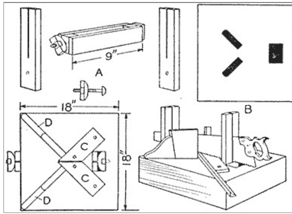
Homemade Miter Box for Sawing Frame Molding and to Hold the Parts for Fastening Together
