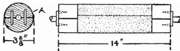
A Wood Mandrel for Attaching Regular Sheets of Sandpaper to Make a Lathe Sander
