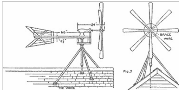
the Manner of Building the Tower on Which the Supporting Standard Revolves (Fig. 7)
