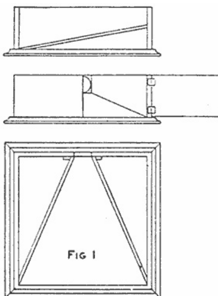
The Horn or Sounding Box Is Constructed in the Auxiliary Base... (Fig. 1)
