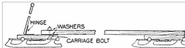
Homemade Pushmobile, Constructed the Same as the Wheeled Kind, with Runners for Snow and Ice
