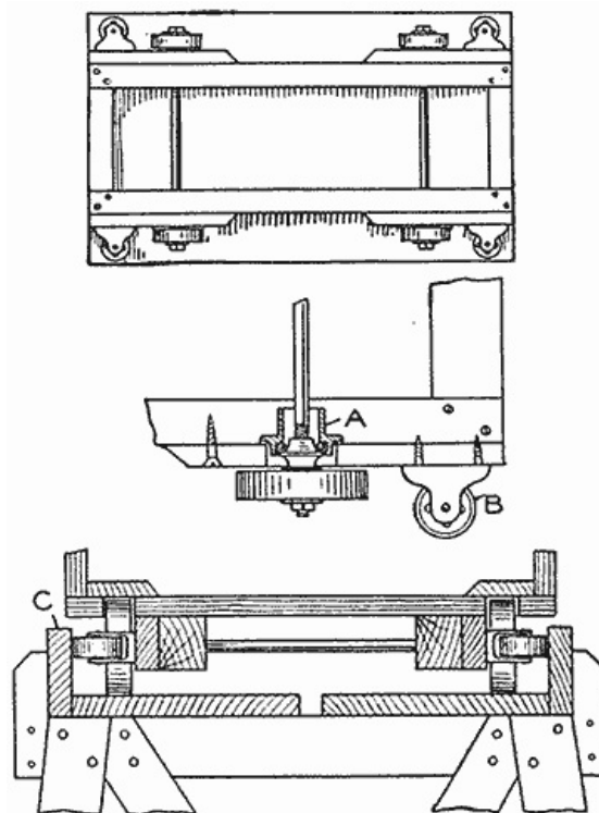
Detail of the Car, Wheels and the Trestle, Which is Attached to a Tie
