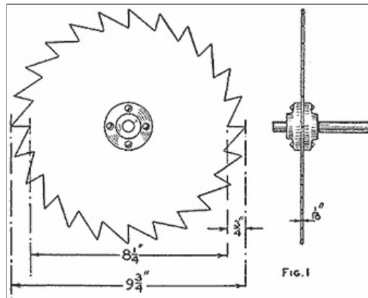
Metal Disk with a Saw-Tooth Circumference That Constitutes the Main Body of the Wheel (Fig. 1)
