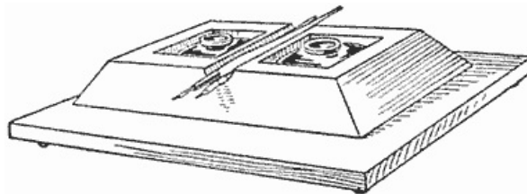
Two Pieces of Pine Shaped to Receive the Inkwells and Finished in Mission Style
