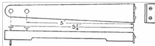
FIG. 6 Construction of the Saw for Making the Groove to Receive the Metal Strip in the Sides (Fig. 6)
