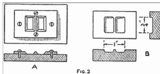
Two Ways of Making the Dies to Shape the Sheet-Metal Water Cups (Fig. 2)
