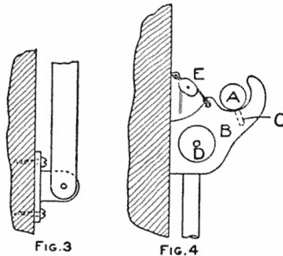
The Attachments, Supports and Brackets for Holding both Curtain Pole and Shade Roller (Fig. 3, Fig. 4)
