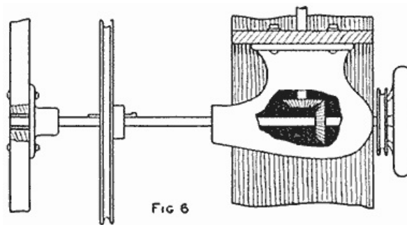
The Lower End of the Shaft has a Horizontal Shaft Geared to It for the Drive Pulleys (Fig. 6)
