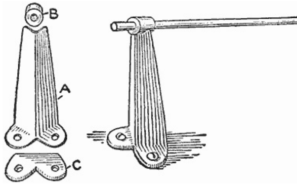
Sheet-Copper Support with a Base and a Shaft Bearing Soldered to the Ends
