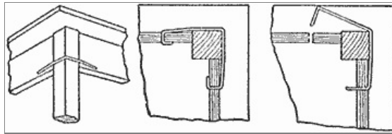
A Piece of Wire Bent around the Leg of a Table will Make It Rigid
