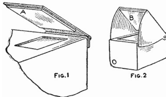
Two Types of Ordinary View Finders and Methods of Converting Them into Direct-View Finders
