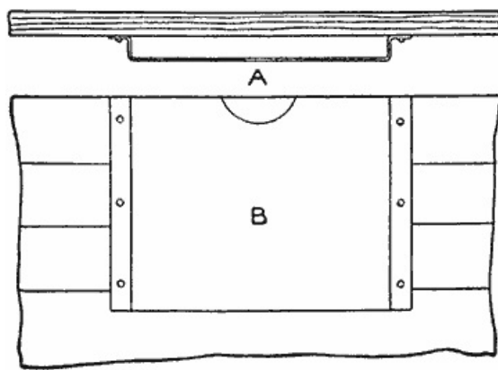
A Receptacle for Emery Cloth Made of Sheet Metal or Tin and Fastened to a Bench
