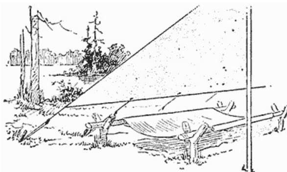
Canvas Bed Made on Two Poles Laid in the Crotches of Forked Stakes
