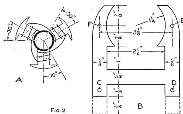
Diagram of the Winding on the Armature and Detail of the Field Laminations (Fig. 2)
