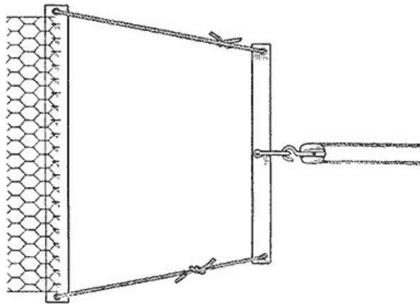
Board Fitted with Screw Hooks and a Pulling Device for Stretching Poultry Fencing on Posts
