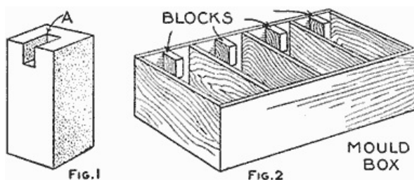
Ar. Anchor Post of Cement and a Mold Box for Shaping Four Posts at a Time (Fig. 1, Fig. 2)
