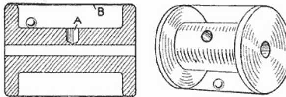
The Steel Ball is Not So Easily Run Into the Hole as It Appears
