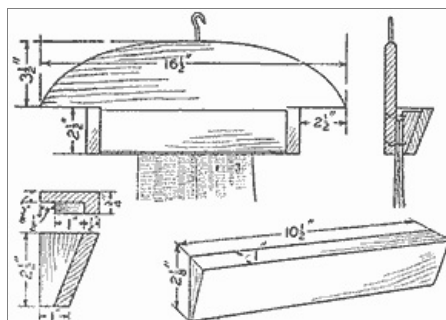
Details of Hangers
