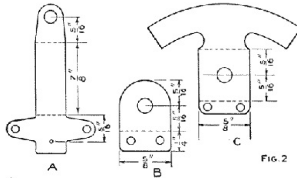
Details of the Supports for the Coil and for the Needle, or Pointer, Shaft (Fig. 2)
