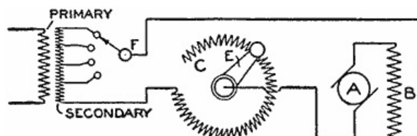
Diagram of a Small Motor Where a Rheostat and Switch Are in the Line (Fig. 2)
