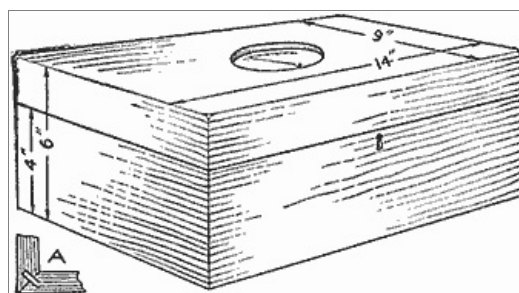
The Amount of Moisture within the Box is Shown on the Dial in the Cover
