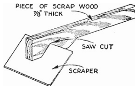
An Ordinary Piece of Board Shaped for a Handle and Notched for the Scraper Blade
