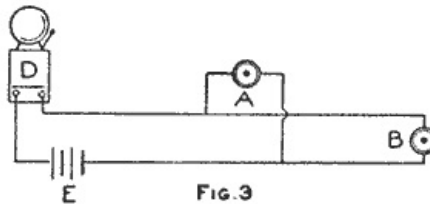
Wiring Diagrams for a Single Bell (Fig. 1, Fig. 2, Fig. 3)
