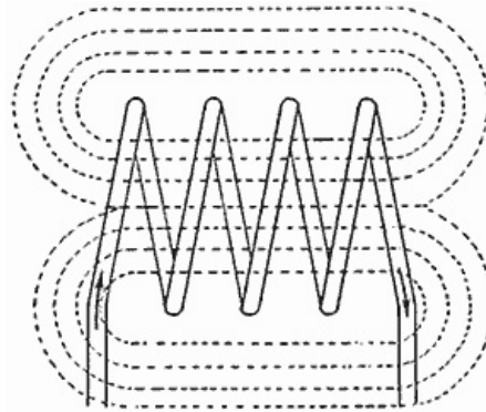
Fig. 6—A Coil about a Magnetic Circuit through Iron and Air
