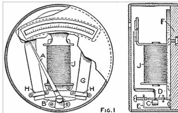
The Parts as They are Assembled to Make a Pocket Voltmeter for Direct Currents (Fig. 1)
