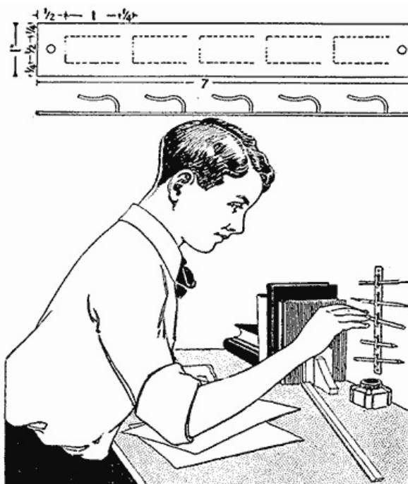
A Strip of Sheet Metal Cut and Clips Formed to Make a Pencil Rack
