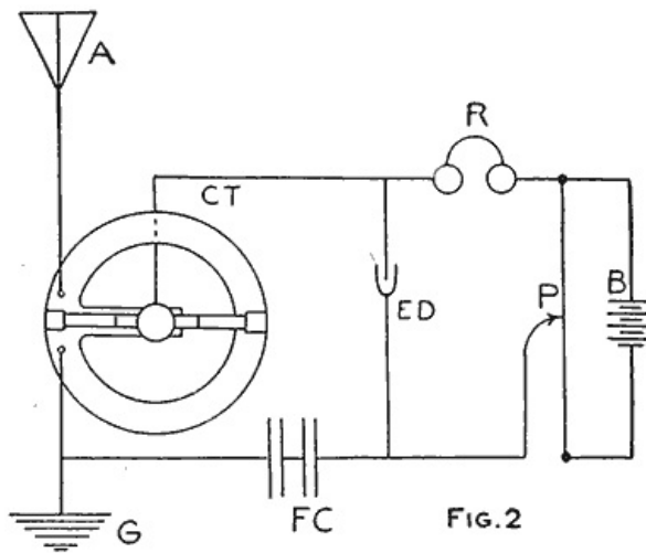
...and Wiring Diagram (Fig. 2)
