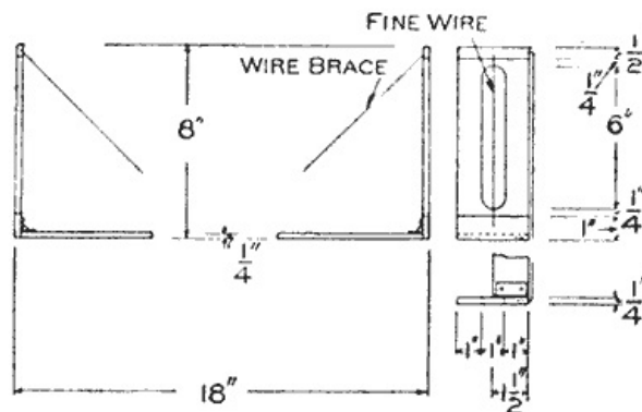
An Alidade, Consisting of Two Sights and a Straightedge, Takes the Place of the Two Needles
