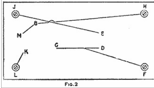
The Base upon Which the Buzzer and Rheostat are Fastened, and the Electrical Connections (Fig. 1, Fig. 2)
