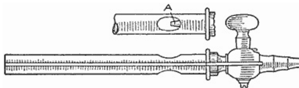
Bunsen-Burner Attachment for Use with Illuminating Gas Taken from the House Mains
