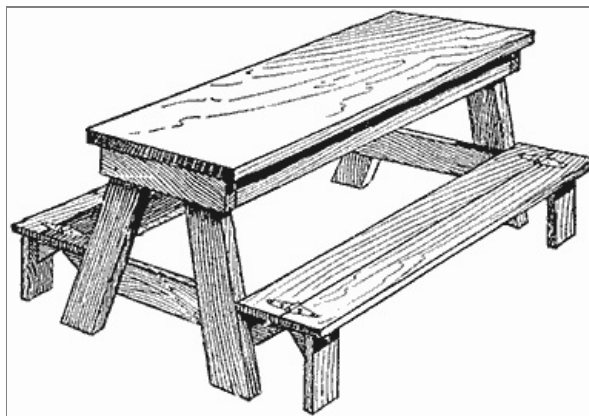
Bench, or Table, with a Seat on Each Side That can be Folded for Carrying Purposes
