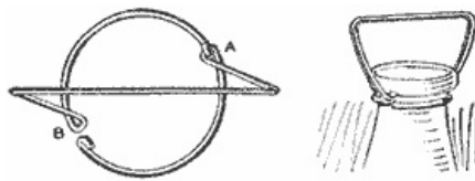
A Carrier Made of Wire to Quickly Attach on a Milk-Bottle Neck
