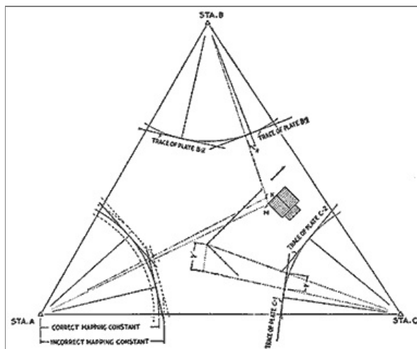
In Plotting a Camera Survey the Base Triangle is First Carefully Laid Out on the Paper to Such a Scale That the Map will be of Desirable Size
