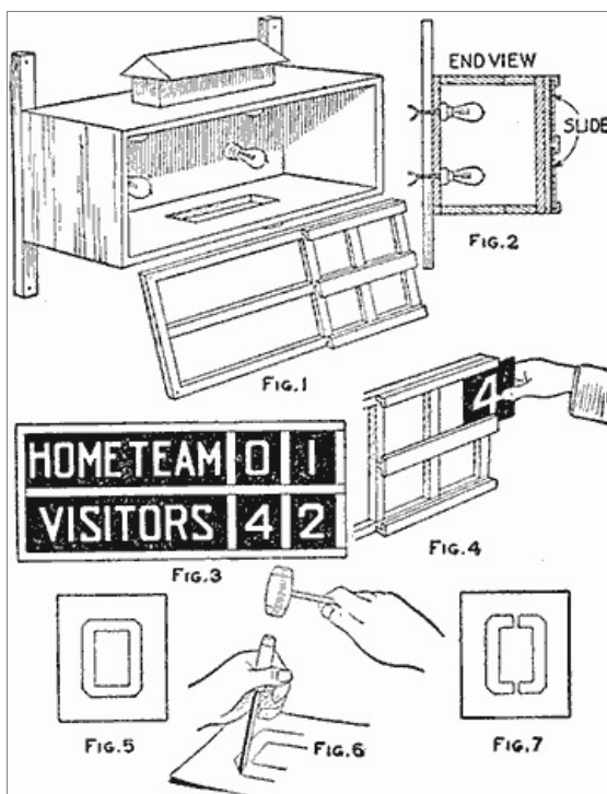
Electric Indoor Score Board, Showing Its Construction and Manner of Cutting Out the Letters and Numbers (Fig. 1, Fig. 2, Fig. 3, Fig. 4, Fig. 5, Fig. 6, Fig. 7)
