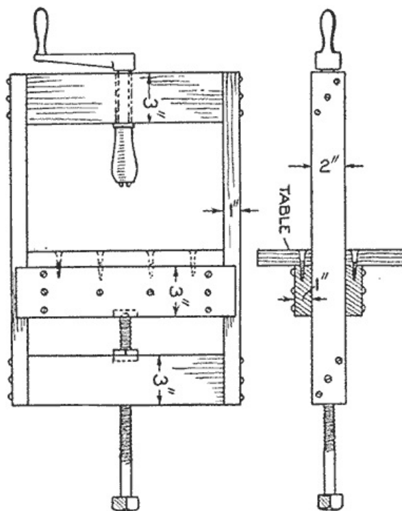
A Very Inexpensive Drill Press Frame Which Answers the Purpose Admirably
