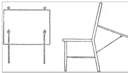
The Writing Board is Easily Attached to, or Detached from, an Ordinary Chair Back
