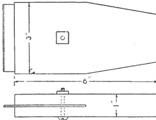
A Handle Attached to a Plain Scraper Blade Makes the Work Much Easier
