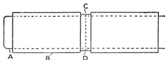
A Wood Mandrel Used to Face the Ends and Turn Flanges on Tubing for Cylinders
