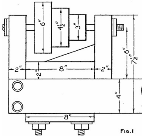
Detail of Wood Lathe (Fig. 1)
