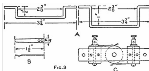
Detail of the Armature Supports and the Brushes, and the Manner of Mounting the Brushes (Fig. 3)
