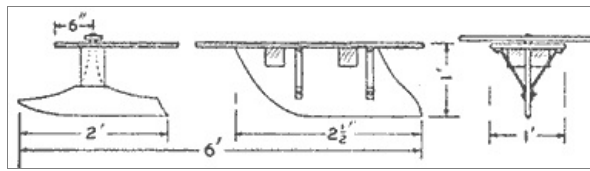
The Construction is Much More Simple Than Making a Double-Runner Bobsled
