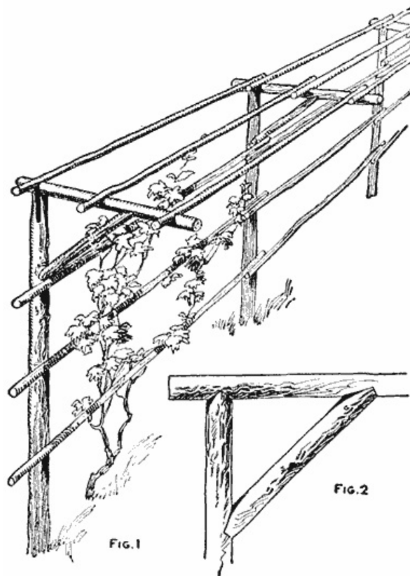
Arbor Made of Poles Which are Supported by One Row of Uprights (Fig. 1, Fig. 2)
