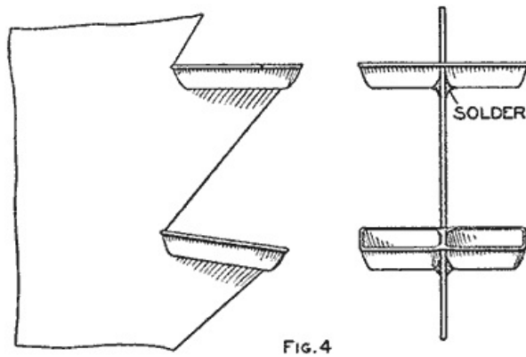
FIG. 4 The Water Cups are Fastened to the Teeth on the Metal Disk with Solder (Fig. 4)
