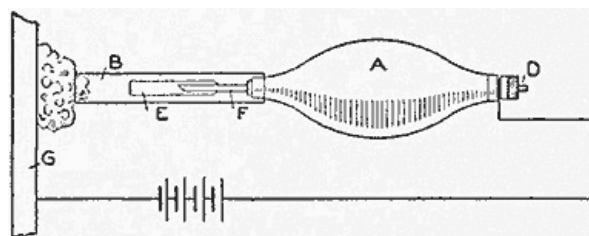
A Hand Tool for Applying a Plate Electrically to the Surface of Metal
