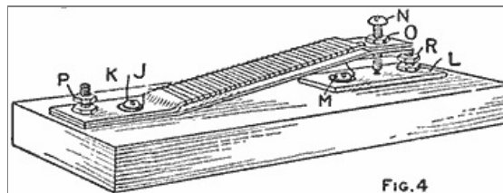
The Assembled Parts Showing the Complete Flasher and Electric Connections with Adjusting Screw (Fig. 4)
