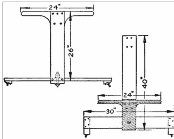
Detail of the Parts for the Construction of the Ice Glider, or Pushmobile
