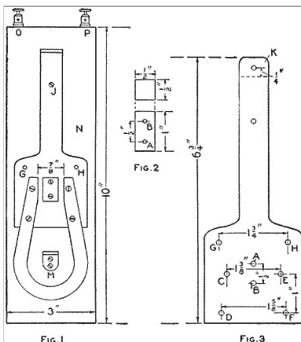
The Permanent Magnet and Its Brass Support, and Their Position on the Base (Fig. 1, Fig. 2, Fig. 3)
