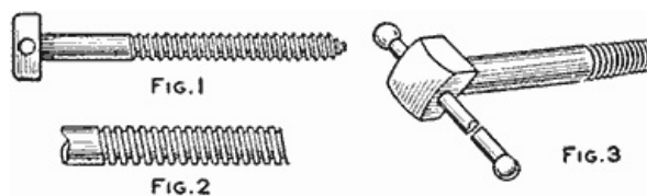
A Vise Screw Formed of an Ordinary Lag Screw, the Threads being Made Square and a Handle Attached (Fig. 1, Fig. 2, Fig. 3)
