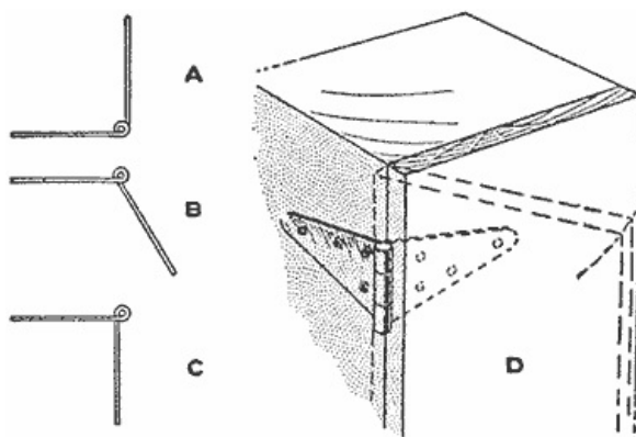
Reversing a Strap Hinge So That When It is Applied Only One Wing will Show
