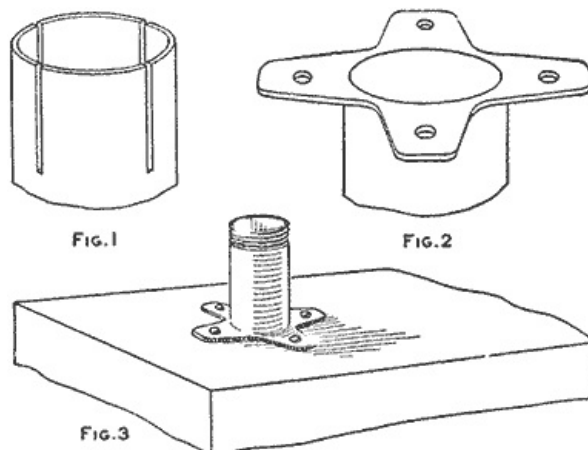
The End of the Pipe as It is Prepared to be Riveted on the Sheet Metal (Fig. 1, Fig. 2, Fig. 3)
