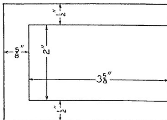
Fig. 12—Outer Portion of the Magnetic Circuit
