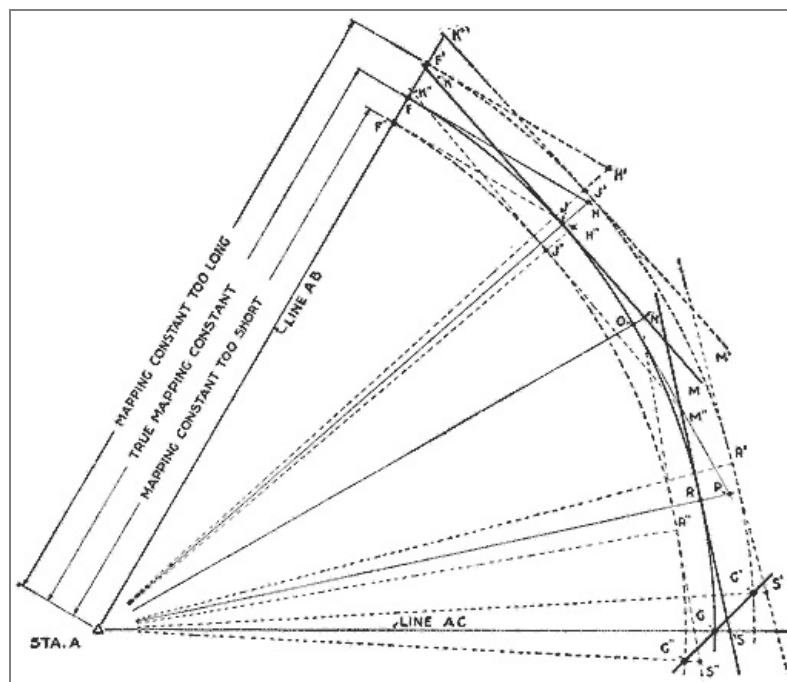
From Each Station the Mapping Constant is Laid Out by the Focal Distance of the Camera or Distance of the Plate from the Lens, and the Location of Traces of the Plates Determined
