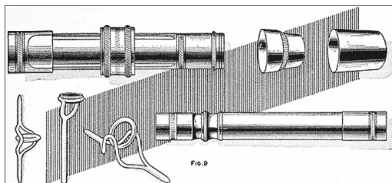
The Mountings Used on a Bait-Casting Rod Consist of a Reel Seat, Butt Cap, Taper Sleeve, Narrow Agate Guide, Agate Offset Top, One Ring Guide, and a Welted, Shouldered Ferrule (Fig. 9)
