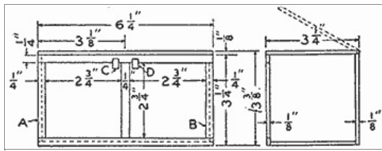
The Box with Doors on One Side and the Top, (Fig. 1)
