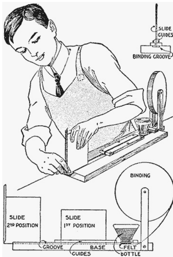
A Machine That will Help to Bind Lantern Slides Quickly and Neatly
