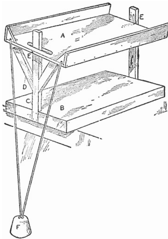
Tray Rocked Automatically by a Weight
