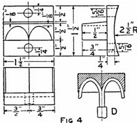
FIG 4 The Best Shape of the Buckets to Take Up the Force of the Water (Fig. 4)
