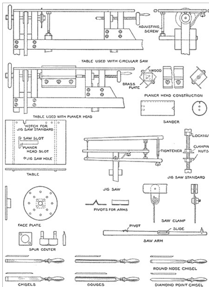
Detail of the Various Attachments for Use in Connection with the Lathe for Sawing, Planing and Sanding, and the Shape of the Tools Used in Turning, Together with the Faceplate and Spur Construction
