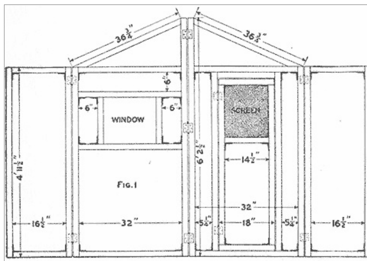
The Entire Framework is Held Together with Brackets, and is Hinged at the Joints, so That It can be Folded Up and Put into a Small Space, the Sections being Covered with Colored Burlap to Make Them Appear Solid... (Fig. 1)
