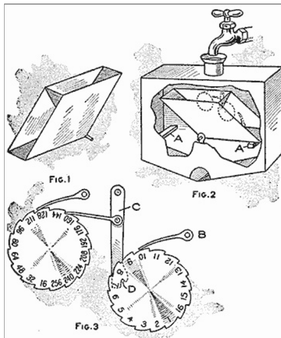
When a Bucket is Filled to the Proper Amount It is Turned Out by the Weight (Fig. 1, Fig. 2, Fig. 3)
