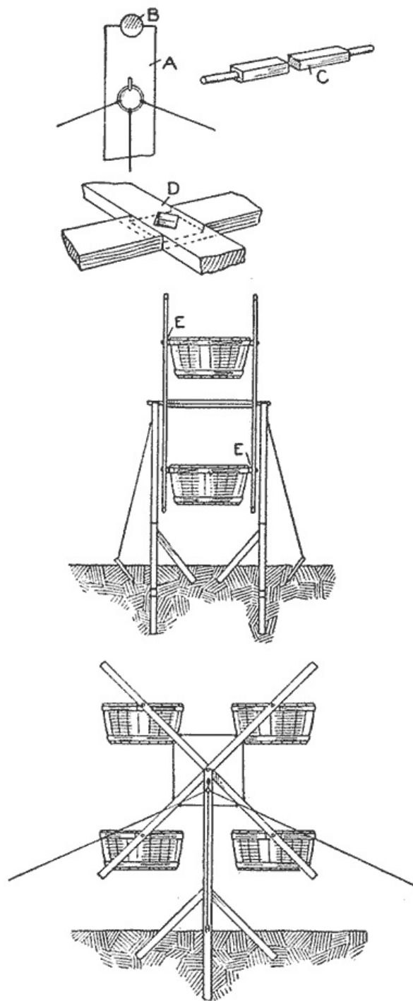
Detail of the Uprights, Axle and Spokes, and the End and Side Elevations of the Completed Wheel, Showing Braces and Cars Attached
