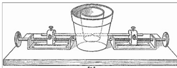
The Furnace Consists of a Flowerpot in Which a Crucible is Set, and on Either Side the Carbon Holders are
