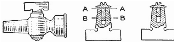
Removing a Portion of the Plug and Shortening the Screw Allows the Parts to be Drawn Tightly Together
