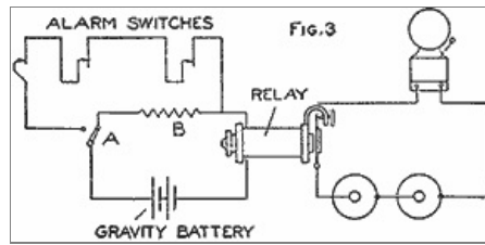
Wiring Diagram Showing Connections for a Closed-Circuit Burglar and Fire Alarm (Fig. 3)
