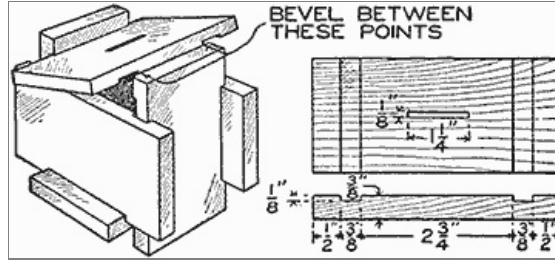
Six Pieces of Wood as They are Put Together to Form a Toy Bank
