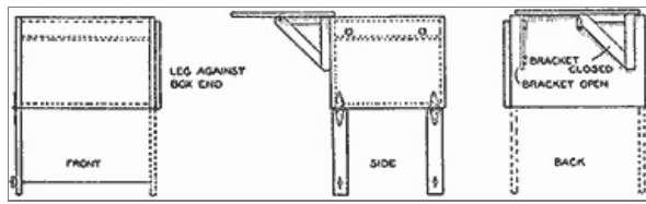
The Brackets for the Cover as Well as Each of the Four Legs Fold Against the Sides of the Box in Such a Manner as to be Out of the Way, Making the Box Easy to Carry and Store Away in a Small Space
