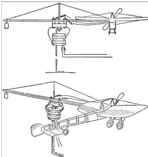
Detail of Parts Showing Wire Connections and Model in Flight around the Central Axis
