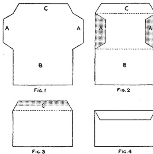
Various Stages in the Forming of an Envelope to Make Any Size for Special Papers (Fig. 1, Fig. 2, Fig. 3, Fig. 4)
