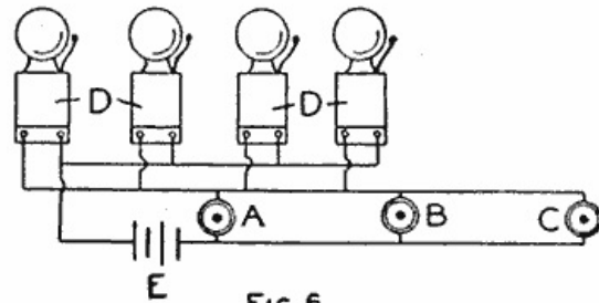
Wiring Diagram for Two or More Bells (Fig. 4, Fig. 5, Fig. 6)
