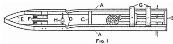
Detail of the Parts for Constructing an Automobile-Type Foot-Power Car (Fig. 1)
