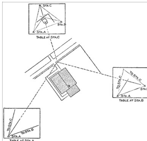
Three Stations are Used for Setting the Plane Table in Succession to Locate the Various Objects TABLE AT STA. A - TABLE AT STA. B - TABLE AT STA. C
