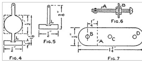
Upper and Lower Connections to the Coil and Supports, and the Supports for Suspension (Fig. 4, Fig. 5, Fig. 6, Fig. 7)
