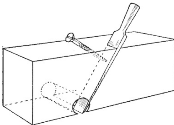
A Plane Made of a Piece of 2 by 4-In. Pine, a Chisel and a Large Wood Screw
