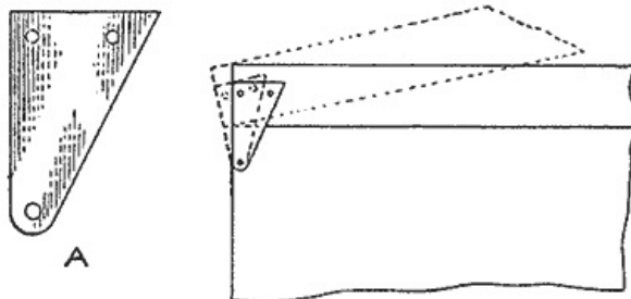
Hinge Parts Made of Sheet Metal and Their Use on a Box Cover
