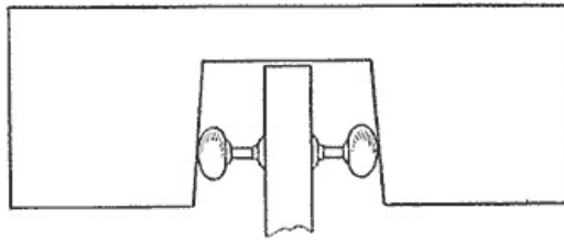
The Sloping Edges in the Notch Forces the Knobs Together and Holds Them While Inserting the Screws
