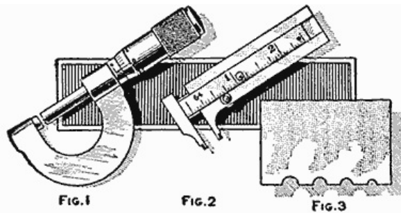
Two Tools for Gauging the Diameter of the Rods, and a Homemade Scraper (Fig. 1, Fig. 2, Fig. 3)
