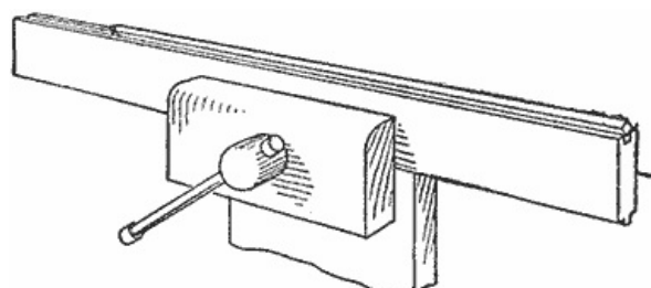
Planing the Corners from Square Stock by Placing Them in the Groove of a Flooring Board
