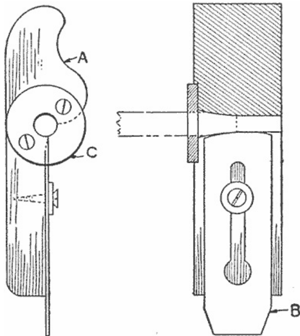
The Tool is Very Similar to a Plane and is Used with a Lathe for Turning Dowels
