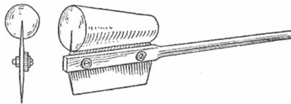
The Wafer Blade Attached to the Handle, the Top Edge being Protected with a Cork
