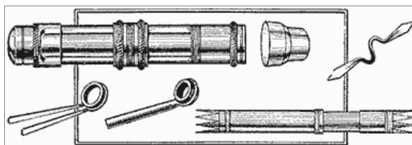
The Mountings for a Fly Rod Consist of a Reel Seat with a Straight Hood, a Taper, Snake Guide, Agate Angle Top, and Serrated Ferrule. The Toothed Ends are Wound with Silk to Afford Additional Strength
