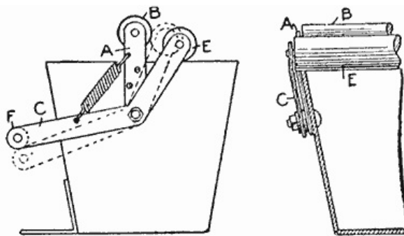
The Parts may be Either Attached to a Metal or Wood Pail with Bolts or Screws
