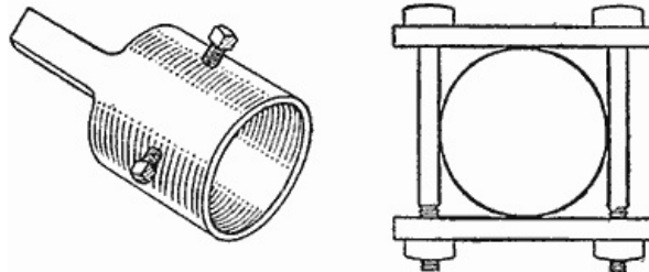
Two Forms of Lathe Dogs That are Quickly and Cheaply Constructed
