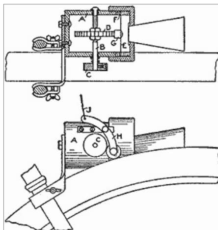
The Horn is Sounded by Making Connections with the Moving Surface of the Tire
