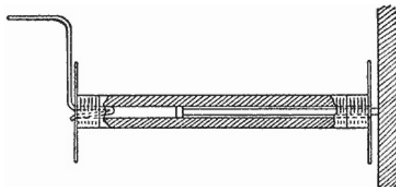
The Film Spool as It is Attached to a Wall, and the Crank for Turning It
