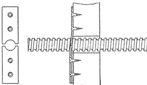
Two Pieces of Strap Iron Shaped to Fit the Square Thread Make a Good Substitute Nut
