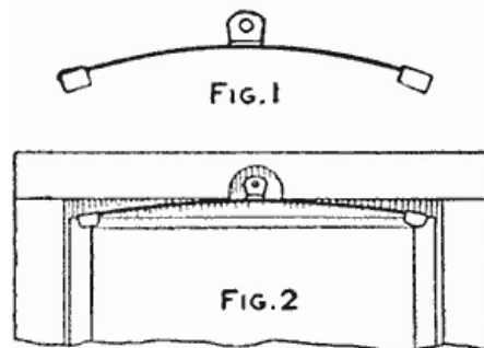
The Spring with Its Clips and Manner of Holding a Negative in a Printing Frame (Fig. 1, Fig. 2)
