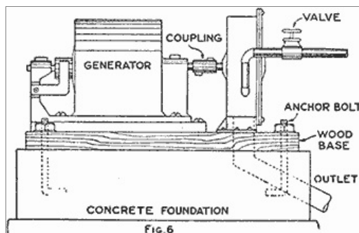
The Motor as It is Coupled to Drive the Dynamo, and the Water Connections (Fig. 6)
