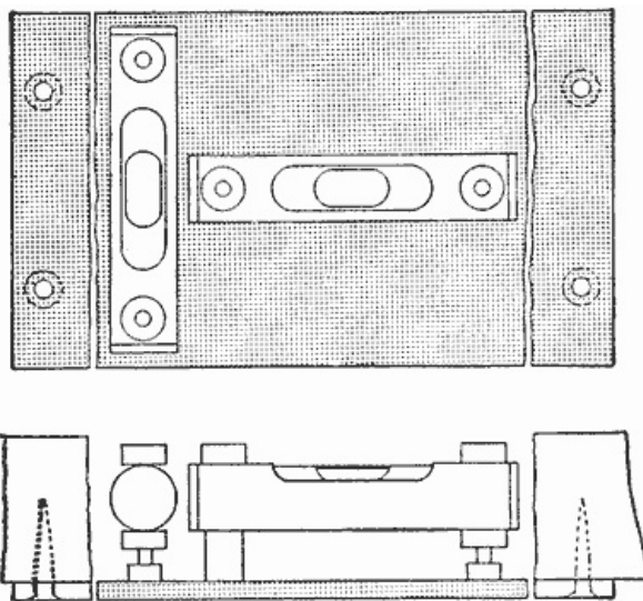
A T-Shaped Level with Adjusting Nuts is Located on the Camera Box, or on the Bed of the Folding Camera
