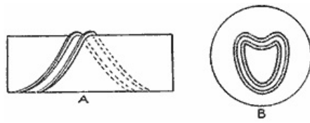
Channels of the Cams Formed with Strips of Brass Soldered to the Drum or Disk
