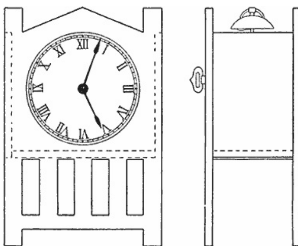
An Alarm Clock with a Wood Covering Ornamented and Finished in Mission Style
