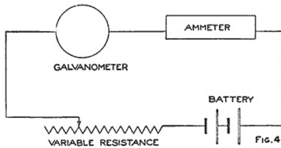
The Electric Circuit, Showing Connections for Finding the Value of a Current in Calibrating (Fig. 4)
