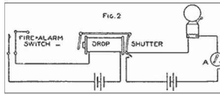
Circuit Equipped with Drop to Ring the Bell in Case the Switch is Destroyed (Fig. 2)
