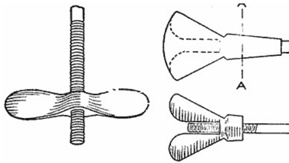
Wing Nuts Made of Discarded Parts Taken from a Faucet or a Gas Bracket
