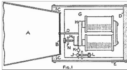
An Electric Horn Operated in a Manner Similar to an Electric Bell on a Battery Circuit (Fig. 1)
