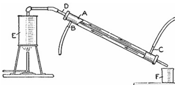
Homemade Still for Removing the Impurities in Water That is Used in Mixing Chemicals
