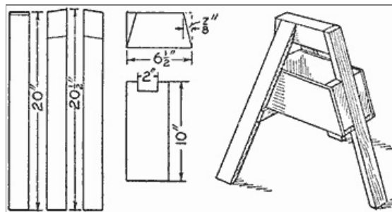
Dimensioned Parts and Completed Stand Which has a Box to Hold the Shining Outfit
