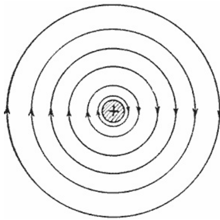
Fig. 4—Magnetic Field Surrounding a Conductor
