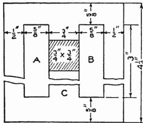
Fig. 11—Complete Magnetic Circuit
