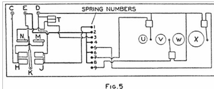
The Wiring Diagram for the Location of the Wires on the Under Side of the Base (Fig. 5)
