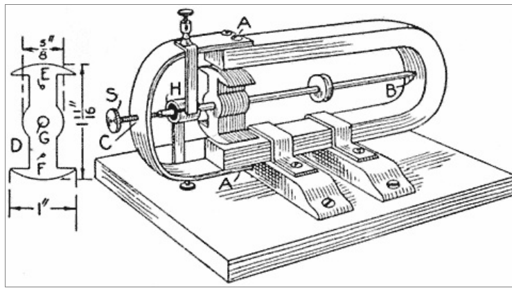
Detail of Armature Laminations, and Completed Parts Assembled, but without Armature Windings
