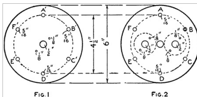
Detail of the Two Ends on the Heater Giving Dimensions and the Location of Parts (Fig. 1, Fig. 2)
