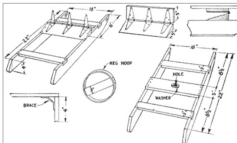
Details Showing the Method of Rear-Sled Oscillation, the Bracing, and the Steering Wheel
