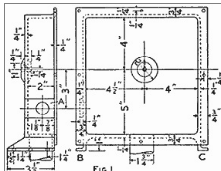
Layout for the Casing, Cover and Wheel for the Construction of a Hydraulic Motor That will Drive a Small Dynamo, to Produce Current for Experimental Purposes, to Charge Storage Cells or to Run Electric Toys (Fig. 1)
