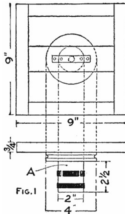
Details of the Different Parts to Construct the Electric Fountain (Fig. 1)
