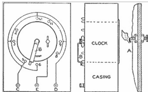
The Alarm Clock in Its Case and the Location of the Contact Pins and Contact Lever (Fig. 1)
