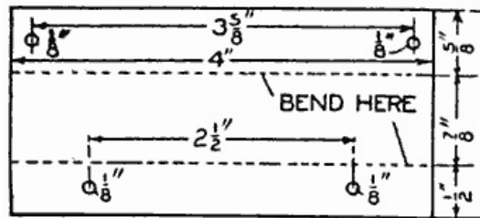
Fig. 17—Lower Clamping Pieces and Mounting Supports
