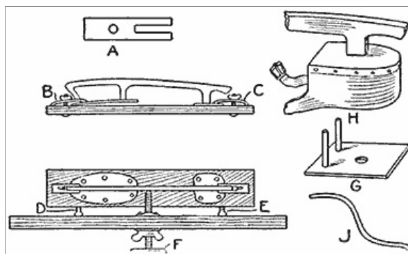
The Holder Provides a Way to Grind a Slight Curve in the Edge of a Skate Blade
