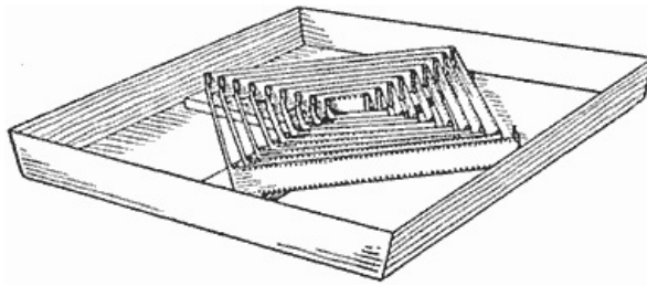
Fig. 4—Cross Arms with Pins
