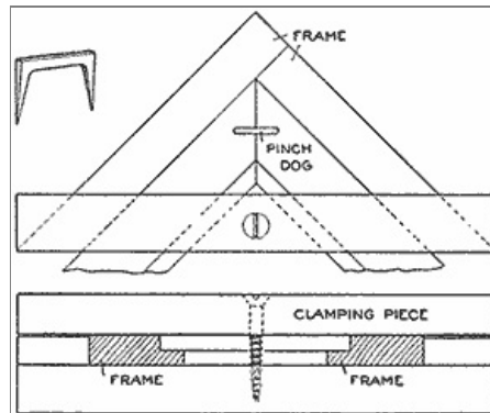
Clamp for Holding the Corner of a Frame While Gluing and Fastening the Mitered Joint
