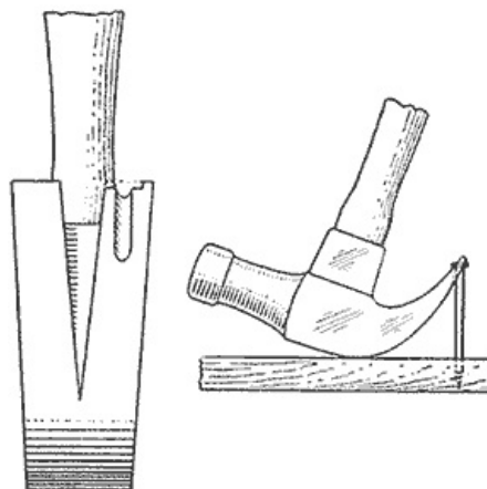
The Small Notch on the End of the Claw Makes It Easy to Pull a Nail Straight
