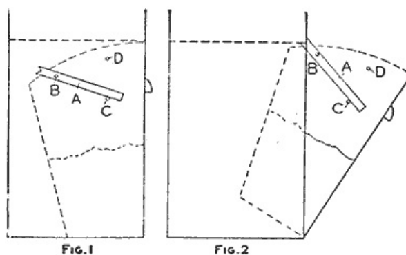
Automatically Operated Catch to Hold a Flour Bin Out While Taking Flour from It (Fig. 1, Fig. 2)
