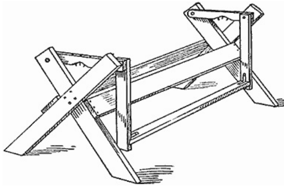
The Holding Attachment Easily Adjusts Itself to the Stick of Wood Placed in the Crotch
