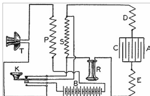
Fig. 7—Sending and Receiving Equipment
