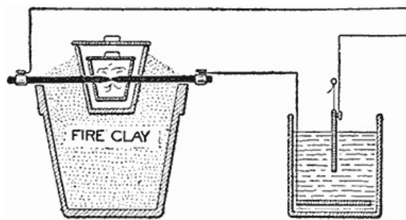
Electric Connections to Furnace
