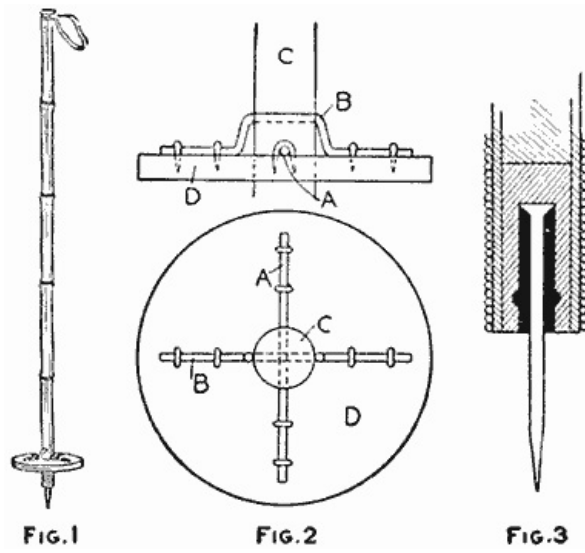
The Staff, being Made of a Bamboo Pole, is Strong as Well as Light (Fig. 1, Fig. 2, Fig. 3)
