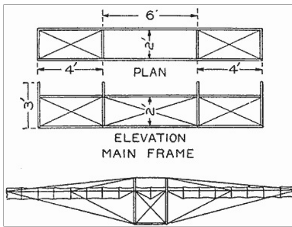
Details of Tandem Monoplane Glider, Showing the Main Frame and Wing Construction, and the Manner of Placing the Crossed Bracing Wires Between the Parts and to the Wing Ends
