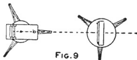
...and Diagram Showing the Location of the Tripods to Direct the Light through the Shutter (Fig. 9)
