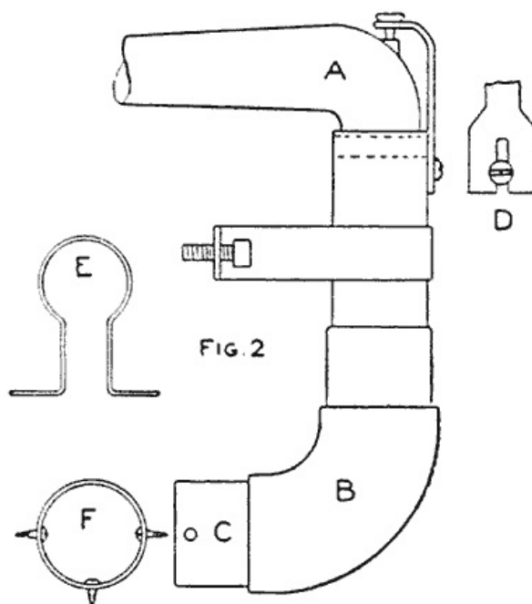
...and the Part for Connecting the Sounding Tube to the Box Consists of Ordinary Gas Pipe Fastened with a Clip at the Back (Fig. 2)
