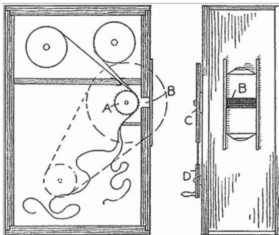
Fig. 7—Printing Machine
