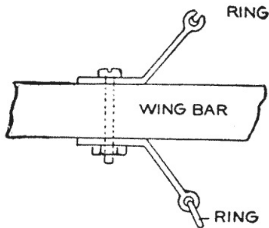
Wing Bar
