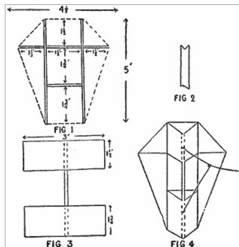
The Sticks are Fastened Solidly with Brads, and the Cloth Sewed to the String around Their Ends (Fig. 1, Fig. 2, Fig. 3, Fig. 4)
