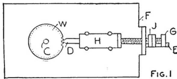
Details of Gear-Cutting Machine (Fig. 1)
