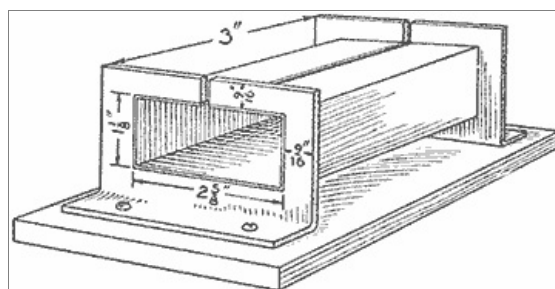
Dimensioned Parts for the Construction of the Core over Which the Insulated Wire is Wound
