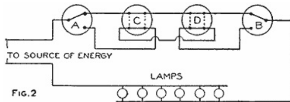
FIG. 2 Lamps Controlled by Any Number of Switches (Fig. 2)
