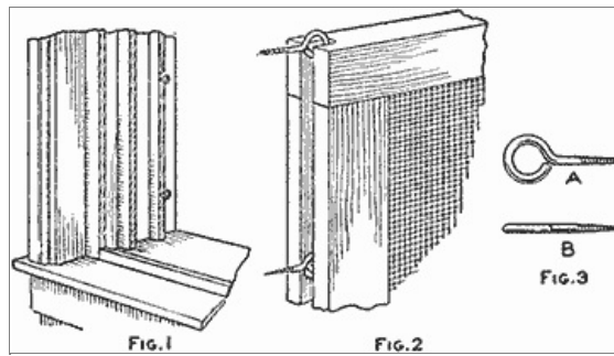
The Heads of the Screweyes in the Window-Frame Stop Slide in a Groove Cut in the Screen Frame (Fig. 1, Fig. 2, Fig. 3)
