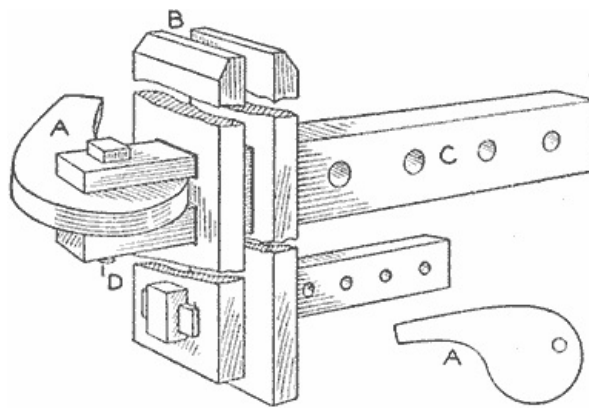
A Vise That can be Quickly Constructed Where No Bench Vise is at Hand
