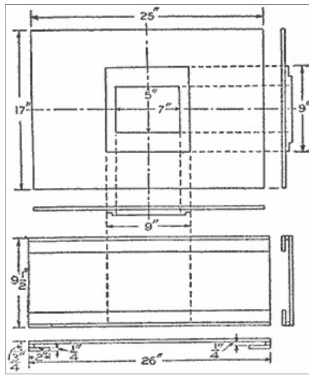
Manner of Laying Out the Pattern for the Back and Locating the Exact Center
