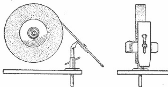
The Plane-Iron Cap Turned at Right Angles, Provides a Guide to Grind the Edge Straight
