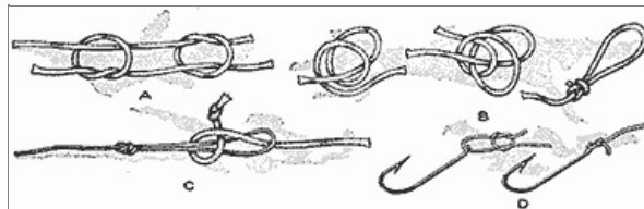
(A) The Single Water Knot Used in Tying Leaders; (B) a Good Knot for Making the Loop at the End of the Leaders; (C) an Angler's Knot Used for Attaching the Line to the Leader, and (D) a Jam Knot for Attaching Eyed Flies, or Hooks, to the Leader or Snell
