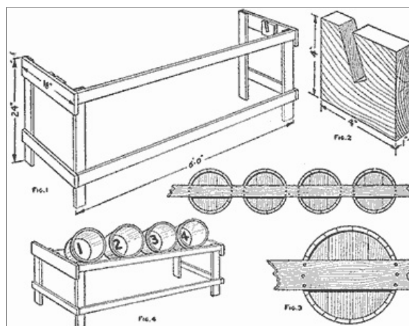
The Frame is Made Up without a Back, to Hold the Buckets at an Angle That Makes It Difficult to Toss the Ball So That It Will Stay in Any One of Them (Fig. 1, Fig. 2, Fig. 3, Fig. 4)
