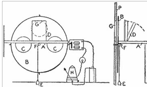
Details of Timing Apparatus
