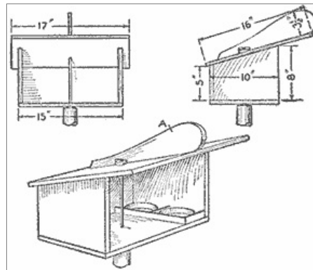
A Feeding Table for Birds That will Keep Its Open Side Protected from the Storms
