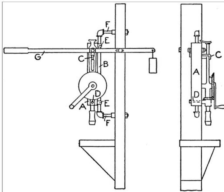
The Breast Drill as It is Attached to an Upright, to Make a Drill Press
