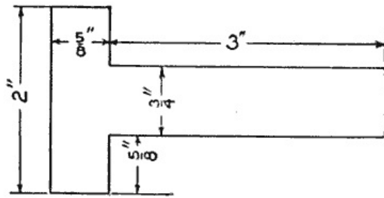
Fig. 13—Inner Portion of the Magnetic Circuit
