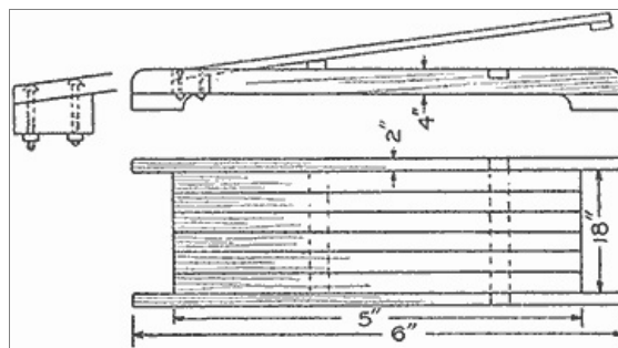
A Springboard for Use in Connection with a Vaulting Pole or for Turning Acts
