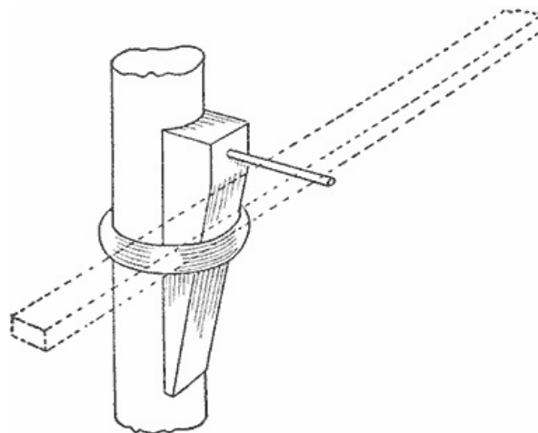
The Ring on the Upright, Held in Position by the Wedge, Which in Turn Carries the Pole on the Pin
