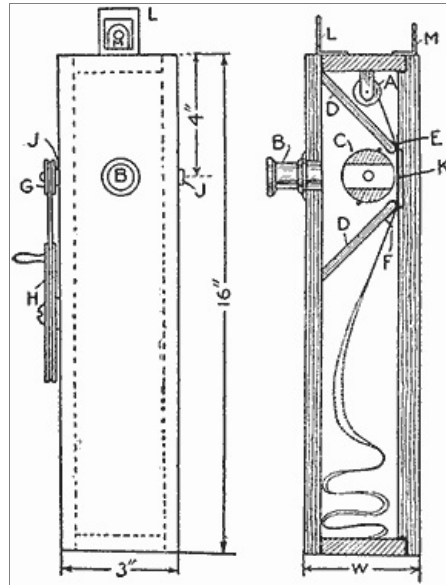
Fig. 2—Details of Camera
