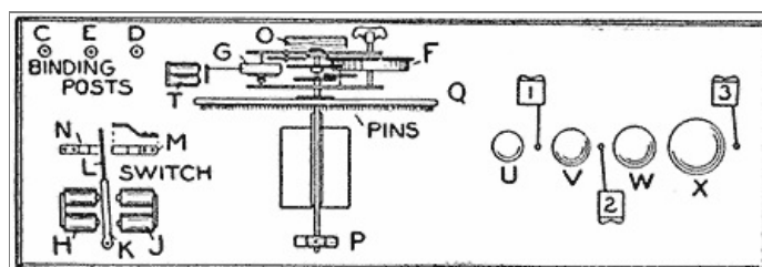
Location of the Clock Works, Magnets, Binding Posts, Gongs and Strikers on the Baseboard (Fig. 2)
