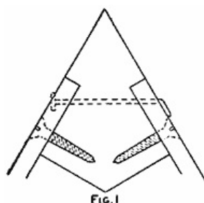
The Skiff is Especially Constructed for Use in Shallow Water and Marshes by Duck Hunters, but with the Addition of a Keel It Makes a Good Craft for Almost Any Water as a Rowboat (Fig. 1)
