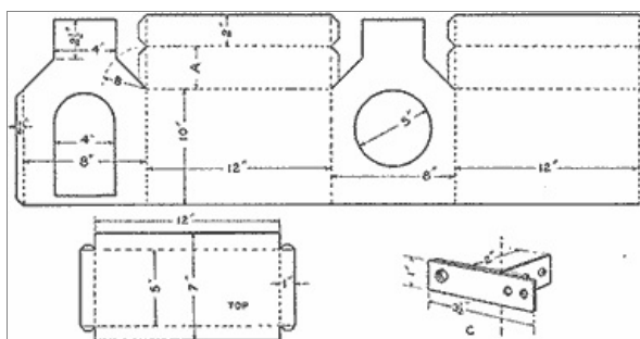
Pattern for Cutting the Metal to Form the Entire Lantern, or Lamp House, Also the Pattern for the Top and the Metal Bracket That Makes a Bearing for the Revolving Wheel, Having Openings Covered with Tinted Celluloid
