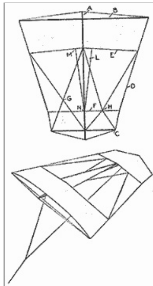
General Plan and Outline of the Kite, Which may be Built in Any Size, If the Proportions are Kept, and Its Appearance in the Air on a Steady Breeze
