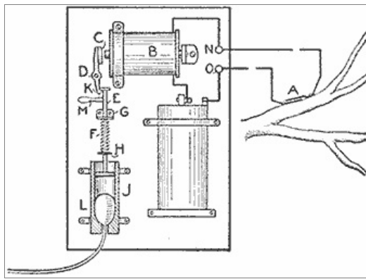
The Electromagnet Trips a Spring Plunger That Forces a Piston on the Camera Air Bulb
