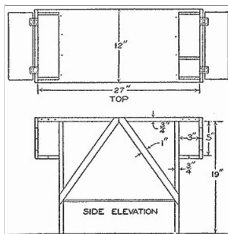
The Bench Provides a Seat for the Worker in Doing Operations on a Small Foot Lathe
