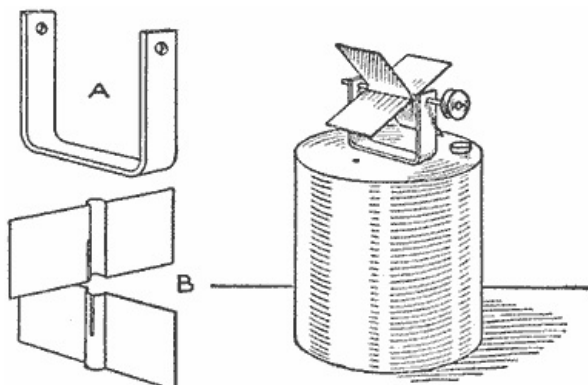
The Boiler is Made of a Fruit or Vegetable Can and the Turbine of Thin Metal Strips
