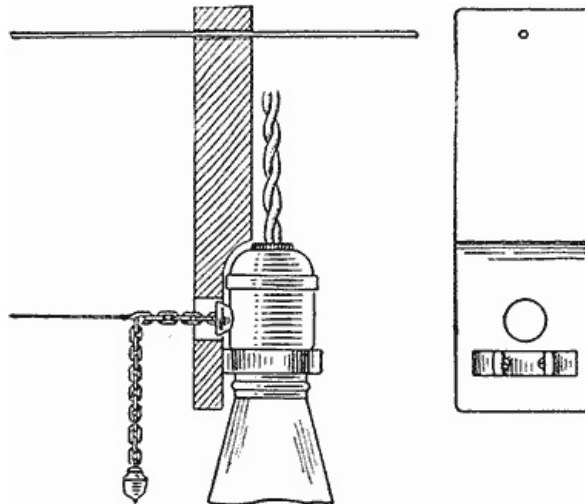
Socket Attachment to Turn a Basement Light On or Off from a Distance
