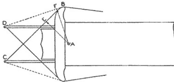
The Most Efficient Way of Attaching Ropes to the Guiding Runners of a Bobsled
