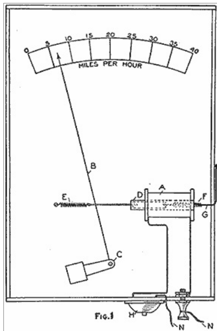
The Indicator Box with Coil, Needle and Scale, as It is Used in Connection with the Anemometer (Fig. 1)
