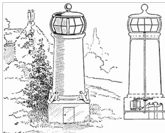
The Flasher as It Appears on the Stand and the Details of Its Construction
