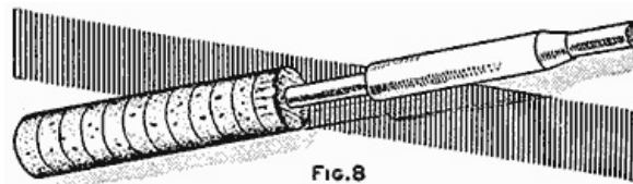
The Corks Glued in Place on the Butt and the Wood Sleeve, or Reel-Seat Core, Ready to Slide Down and Glue in Position (Fig. 8)
