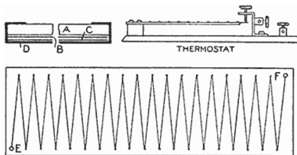
Fig. 2—Heater Details
