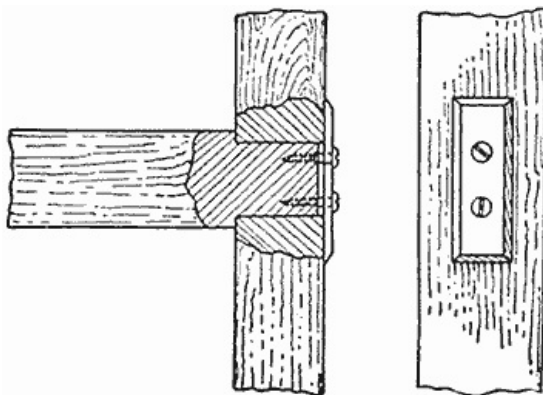
Metal Covering and Holder for a Tenon and Mortise Joint on Mission Furniture
