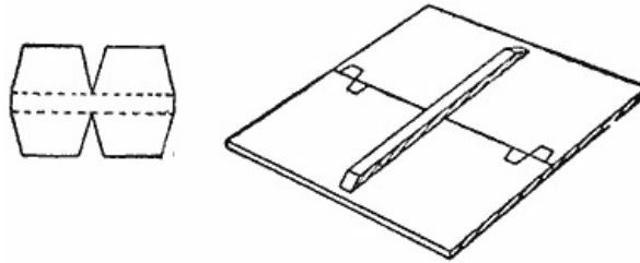
The Metal Clips Hold the Edges of the Boards Together Closely and Quite Rigidly
