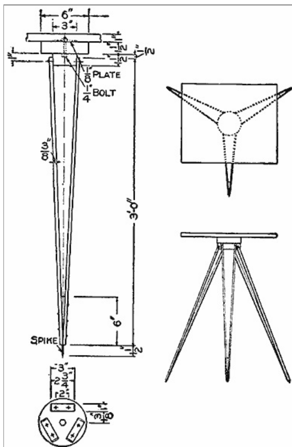
A Rigid Tripod is Made of Strips for Legs, Which are Fastened to a Large Top
