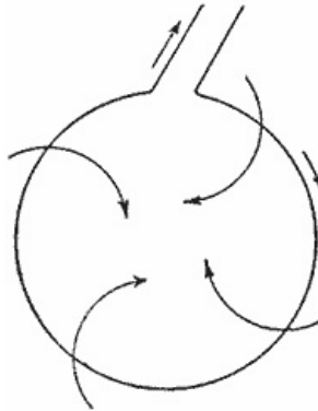
Fig. 5—Magnetic Field about a Coil
