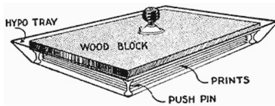
Push Pins on the Under Side of the Board Raise It and Provide a Space for the Prints in the Liquid
