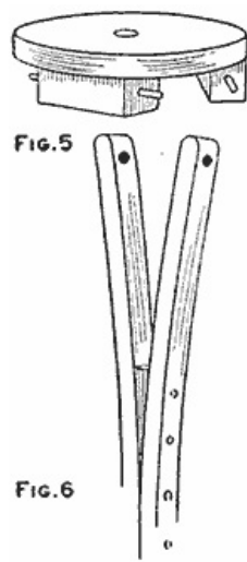
The Parts in Detail for Making the Tripods... (Fig. 5, Fig. 6)
