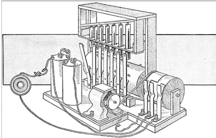
Detail of the Parts for the Construction of a Musical Doorbell That will Play the Music on Brass Tubes with One Touch of a Push Button
