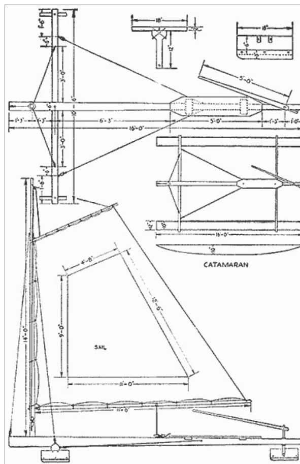
The Ice-Boat Details, Showing Construction with Straight Poles Having Detachable Runners So the Boats can be Supplied in Their Stead to Make a Sailing Catamaran for Use in Summer
