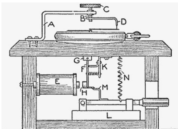
Time Switch for Operating an Electric Light in Printing Photographic Developing Papers
