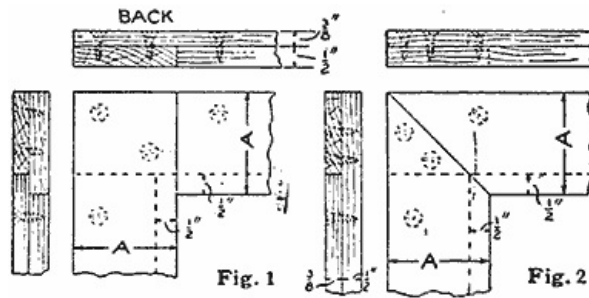
Square and Mitered Lap Joints for Making Rigid Picture Frames in Natural or Stained Woods (Fig. 1, Fig. 2)
