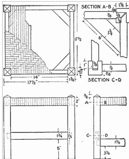
Construction of the Frame and Manner of Laying the Weavers for the Top
