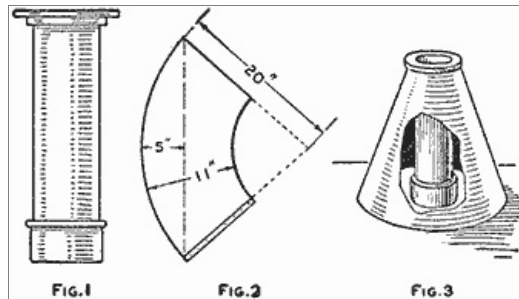
The Parts to Make the Crucible Consist of Pipe and Fittings and a Piece of Sheet Metal (Fig. 1, Fig. 2, Fig. 3)
