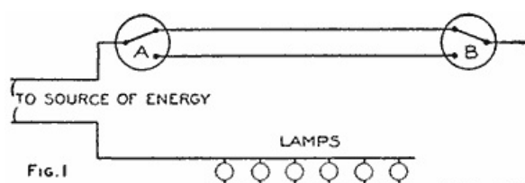
Lamps Controlled from Two Switches (Fig. 1)
