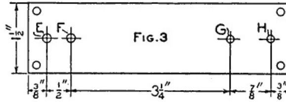
Dimensions of the Brass Strip and Mounting Base, Showing the Location of the Holes and the Shape of the Brass Strip to Receive the Coil of Wire (Fig. 1, Fig. 2, Fig. 3)
