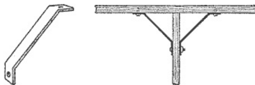
The Braces are Cut from Stake Iron or Sheet Metal According to the Size Machine being Built
