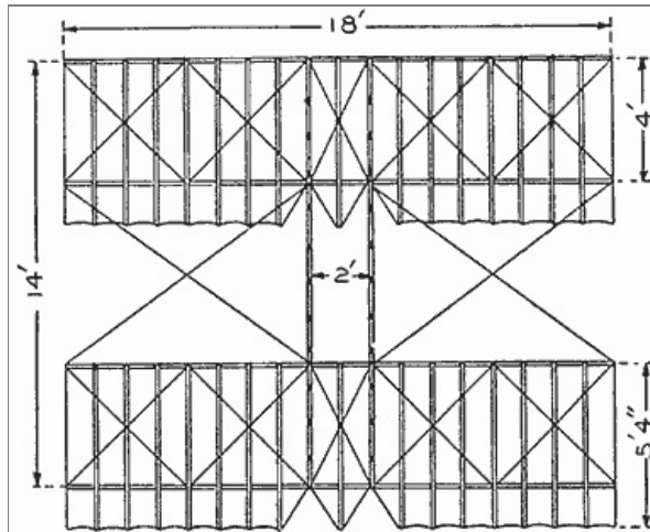
Details of Tandem Monoplane Glider, Showing the Main Frame and Wing Construction, and the Manner of Placing the Crossed Bracing Wires Between the Parts and to the Wing Ends
