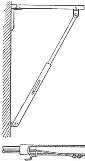
When the Shelf is Lowered the Support Telescopes and is Out of the Way
