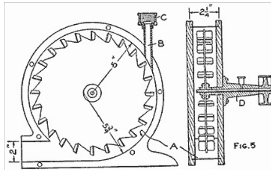
FIG. 5 The Housing for the Wheel with a Connection to Attach the Motor on an Ordinary Faucet (Fig. 5)
