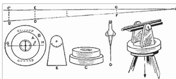
Detail of Parts for the Construction of a Transit Which can be Used, with Fairly Accurate Results, in Doing Amateur Surveying for Railroad Work, Town Sites and the Laying Out of Maps
