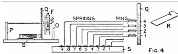
The Contact Springs are Operated by the Pins on the Disk Wheel (Fig. 4)
