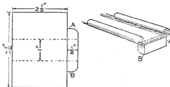
Gauge Made of Sheet Metal Which will Easily Snap on a Carpenter's Rule
