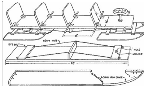
The Top Board is Well Braced on the Under Side and Fitted with Four Backs on Top to Make It a Luxurious Riding Sled, and the Runners are Provided with Metal Shoes for Speed
