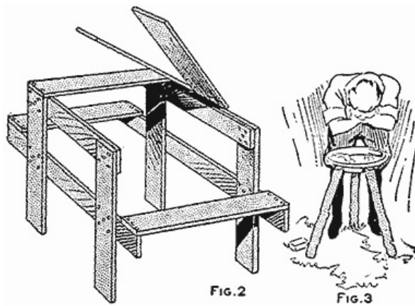
A Table Made of Packing-Box Material and a Wash Basin Stand of Three Stakes (Fig. 2, Fig. 3)
