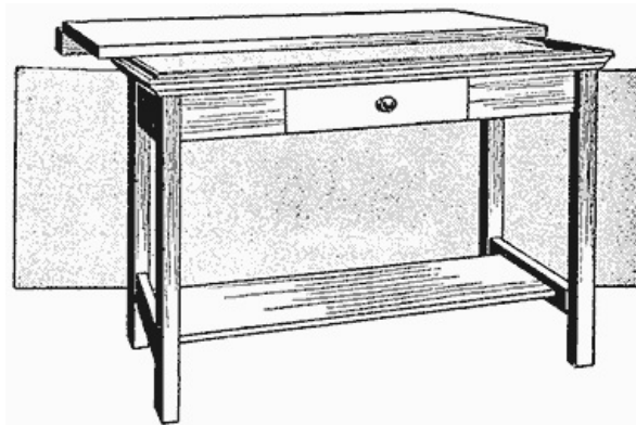
The Table When Drawn Out Uncovers the Zinc Tray, Fastened on Top
