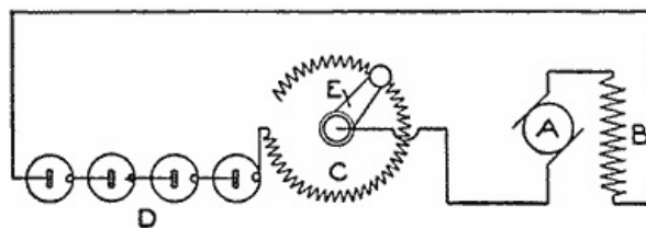
Diagram Showing the Connections for a Small Motor Where a Rheostat Is in the Line (Fig. 1)
