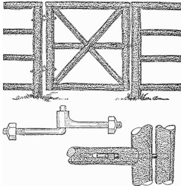
Gate Openings were Made in the Fence Where Necessary, and Gates of Poles Hung in the Ordinary Manner
