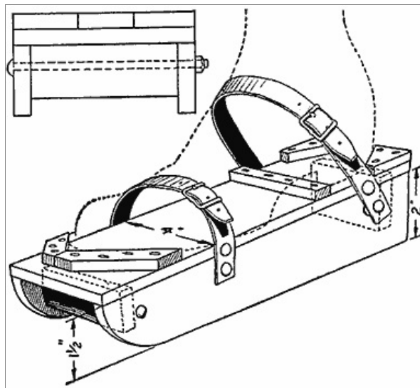
Skates Made of Wood to Take the Place of the Steel-Runner Kind and Prevent Sprained Ankles
