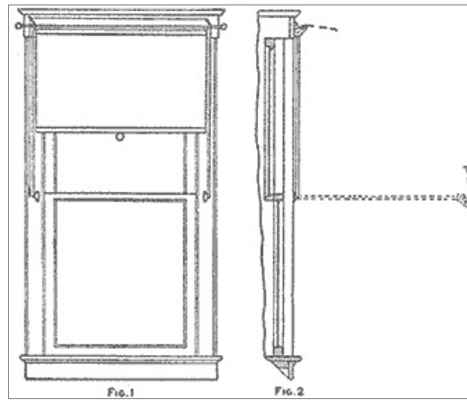
The Brackets as They are Attached to a Window Casing for Lowering the Curtain Pole (Fig. 1, Fig. 2)
