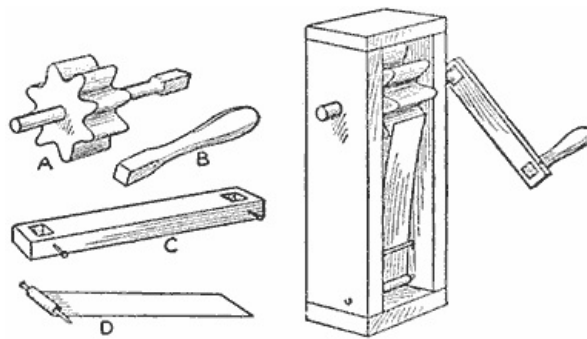
Detail of the Parts and How They are Assembled to Make the Clapper
