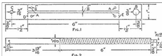
Details of the Base, Rod and Handle for Each Carbon Feed, Which is Attached to the Large Base on One Side of the Furnace (Fig. 1, Fig. 2)
