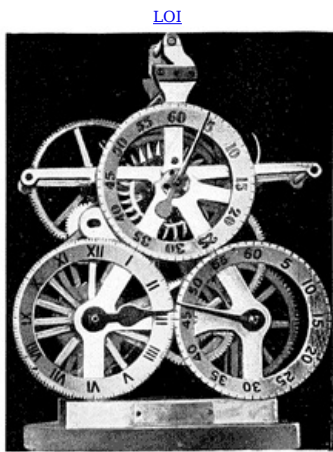
Fig. 30—Remontoir Clock Movement
