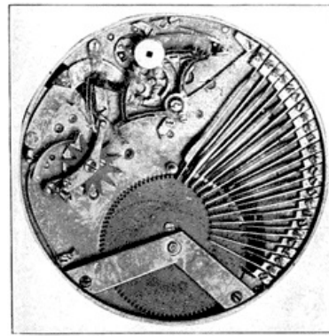
Fig. 41—Musical Watch, Repeating Hours and Quarters
