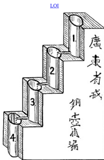
Fig. 8—“Hon-woo-et-low” or “Copper Jars Dropping Water”—Canton, China
