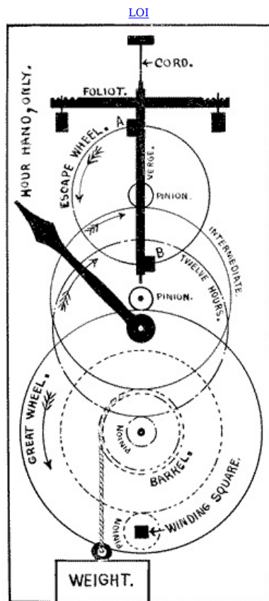
Fig. 26—De Vick's Clock of 1364
