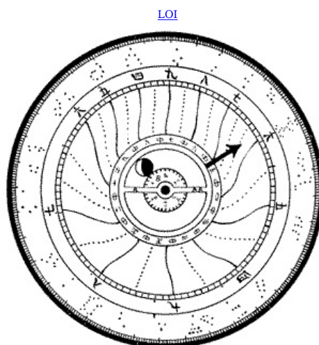
Fig. 22—Dial of Japanese Astronomical Clock
