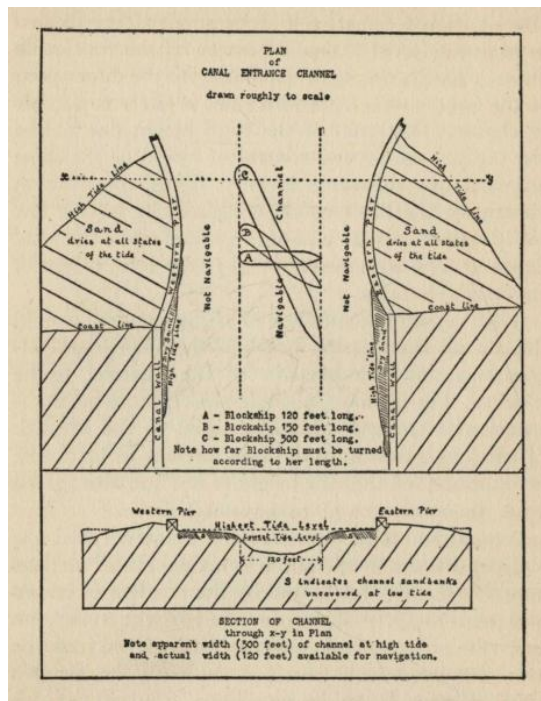
Plan of CANAL ENTRANCE CHANNEL
