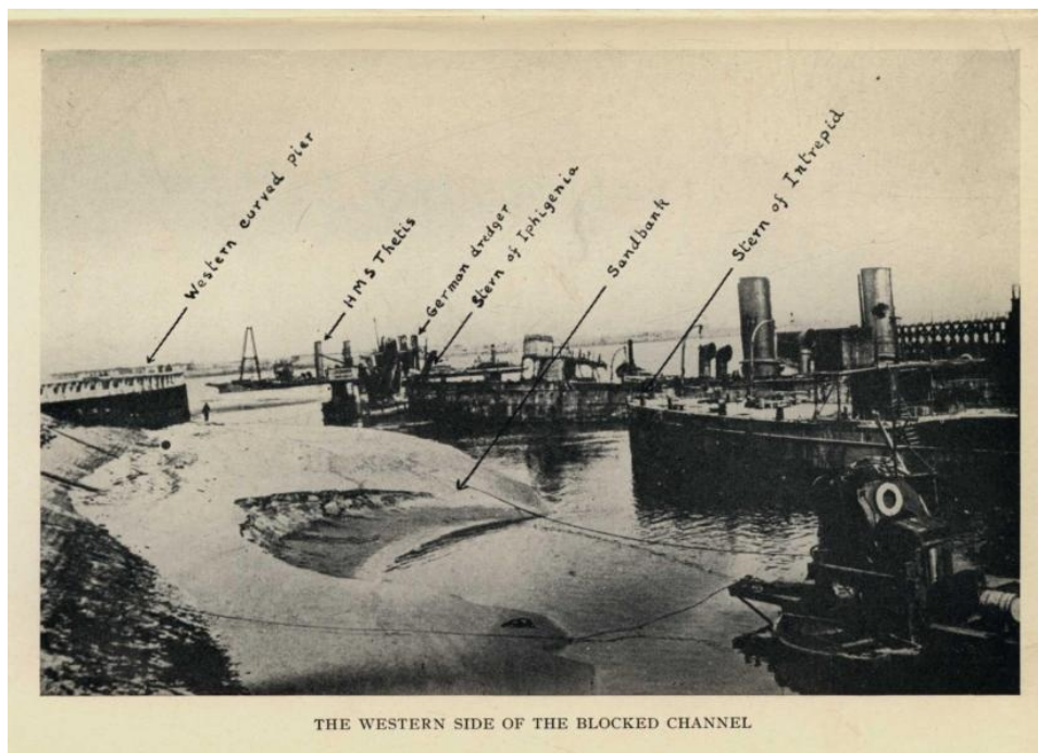
THE WESTERN SIDE OF THE BLOCKED CHANNEL
