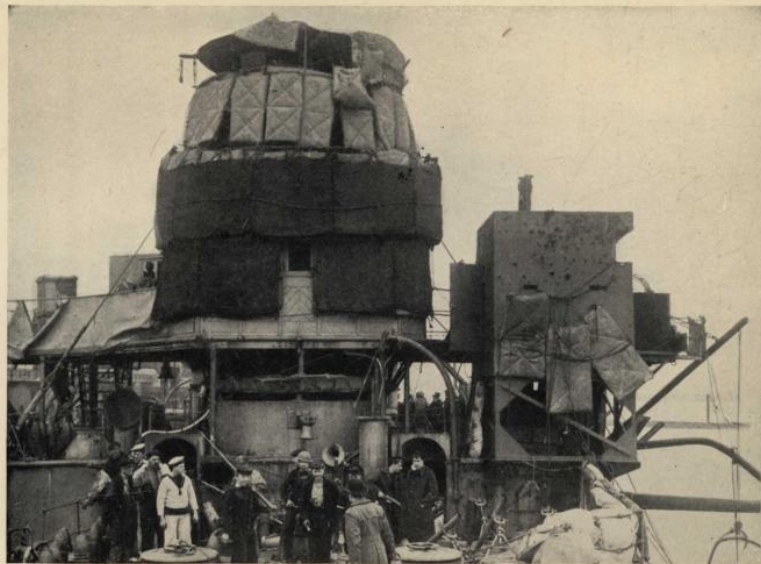
H.M.S. VINDICTIVE'S BRIDGE AND FLAME-THROWER HUT (RIGHT) The fighting top is shown above, and from behind, the bridge. The conning tower is below the bridge. A large shell passed through the hole to the right of the man in white uniform
