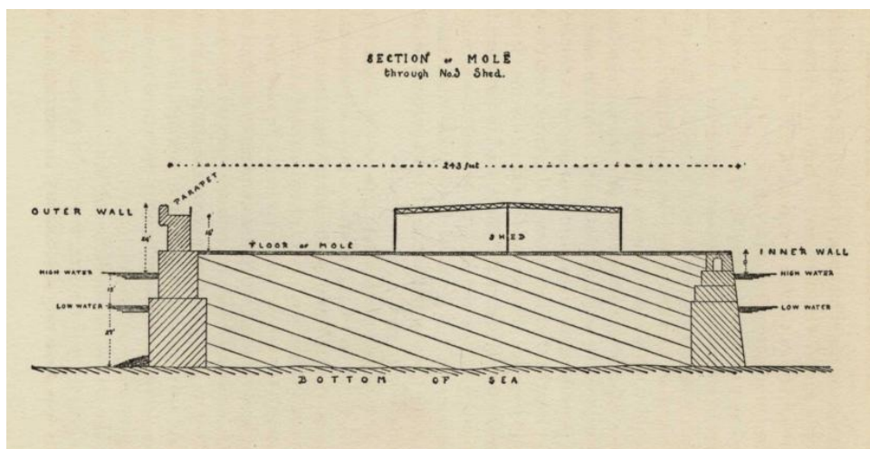
SECTION of MOLE through No. 3 Shed
