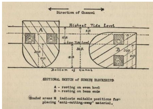
SECTIONAL SKETCH of SUNKEN BLOCKSHIPS
