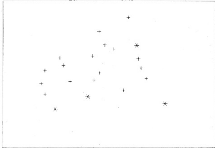
Star-cluster in Orion's Head
