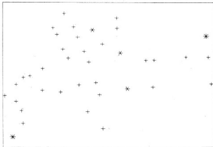
Star-cluster of Praesepe in Cancer
