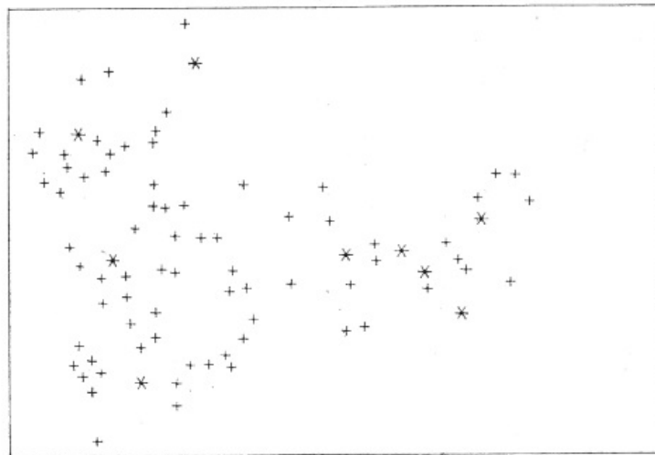
Orion's Belt and Sword; 83 Stars
