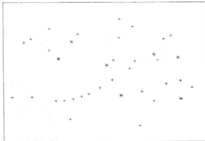
Pleiades; 36 Stars
