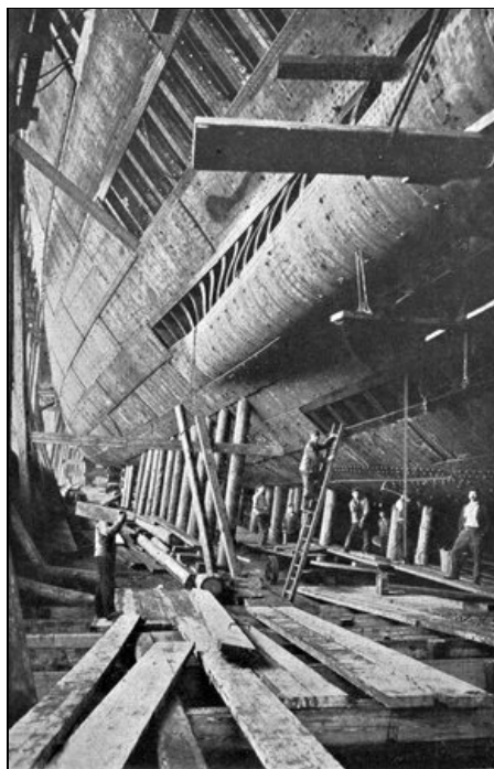
RIVETTING THE OUTER SKIN ON THE FRAMES OF A 65,000-TON OCEAN LINER
