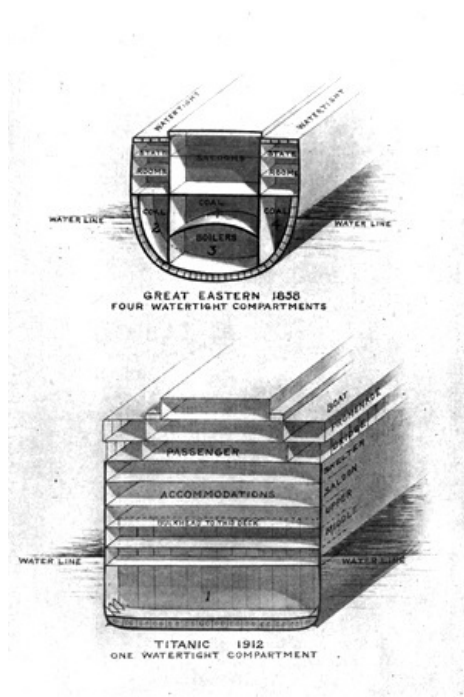
GREAT EASTERN 1858 FOUR WATERTIGHT COMPARTMENTS
