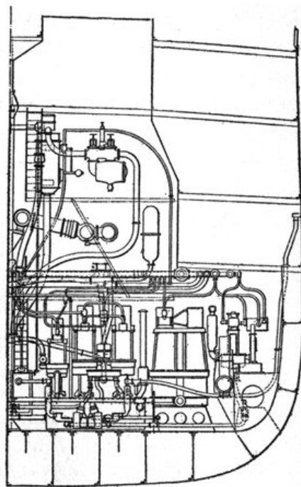
SECTION THROUGH ENGINE-ROOM OF THE KAISER WILHELM II, SHOWING INNER BOTTOM CARRIED UP SIDES OF SHIP, TO FORM DOUBLE SKIN
