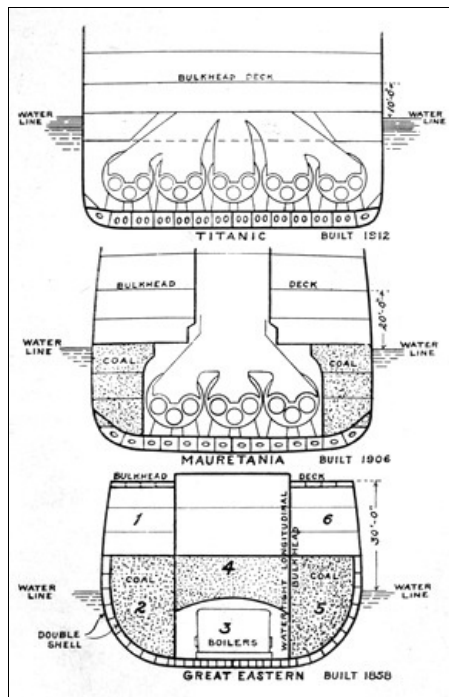
TITANIC BUILT 1912 MAURETANIA BUILT 1906 GREAT EASTERN BUILT 1858
