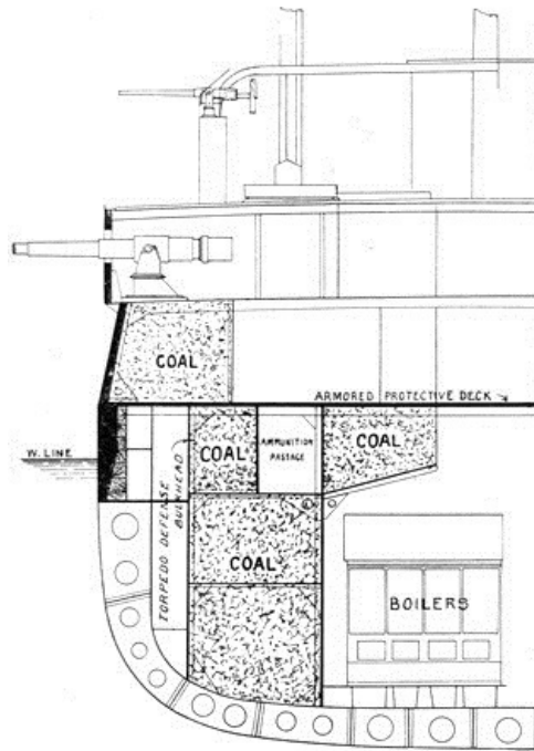
Between the boiler rooms and the sea are four, separate, watertight walls of steel. The whole is covered in by a 3-inch watertight steel deck.
