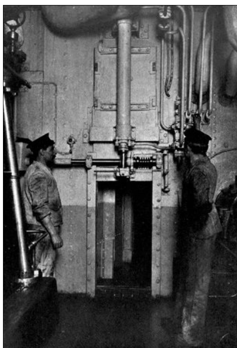
HYDRAULICALLY-OPERATED, WATERTIGHT DOOR IN AN ENGINE-ROOM BULKHEAD
