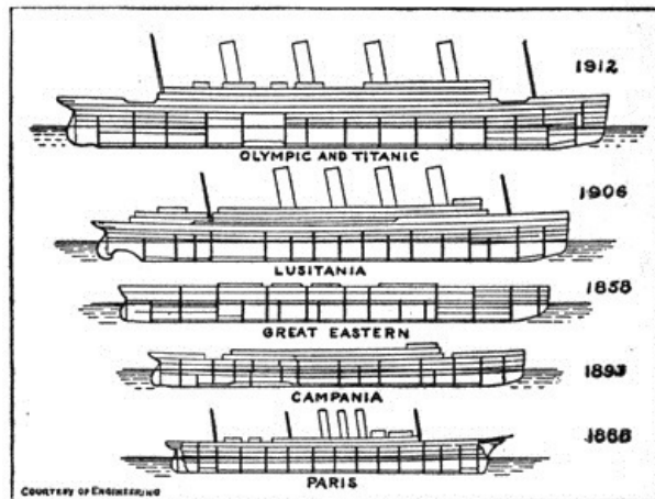
COURTESY OF ENGINEERING OLYMPIC AND TITANIC 1912 LUSITANIA 1906 GREAT EASTERN 1858 CAMPANIA 1893 PARIS 1868
