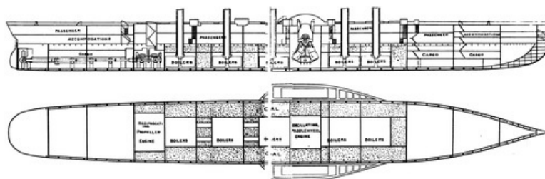
Length, 692 feet; beam, 83 feet; depth, 58 feet. Subdivision: Double hull; nine main bulkheads, 53 feet high, extending to upper deck, and six sub-bulkheads 35 feet high, extending to lower deck. Two longitudinal bulkheads through machinery spaces.
