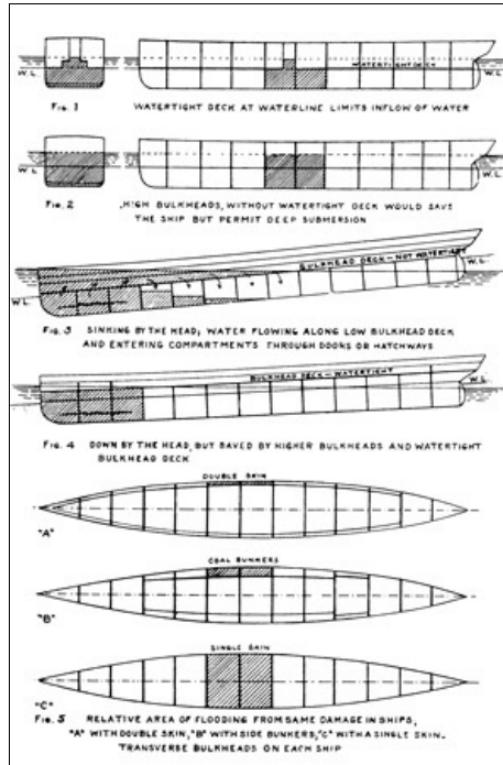
FIG. 1 WATERTIGHT DECK AT WATERLINE LIMITS INFLOW OF WATER FIG. 2 HIGH BULKHEADS, WITHOUT WATERTIGHT DECK WOULD SAVE THE SHIP BUT PERMIT DEEP SUBMERSION FIG. 3 SINKING BY THE HEAD; WATER FLOWING ALONG LOW BULKHEAD DECK AND ENTERING COMPARTMENTS THROUGH DOORS OR HATCHWAYS FIG. 4 DOWN BY THE HEAD, BUT SAVED BY HIGHER BULKHEADS AND WATERTIGHT BULKHEAD DECK FIG. 5 RELATIVE AREA OF FLOODING FROM SAME DAMAGE IN SHIPS, "A" WITH DOUBLE SKIN, "B" WITH SIDE BUNKERS, "C" WITH A SINGLE SKIN. TRANSVERSE BULKHEADS ON EACH SHIP DIAGRAMS SHOWING PROTECTIVE VALUE OF TRANSVERSE AND LONGITUDINAL BULKHEADS, WATERTIGHT DECKS, AND INNER SKIN
