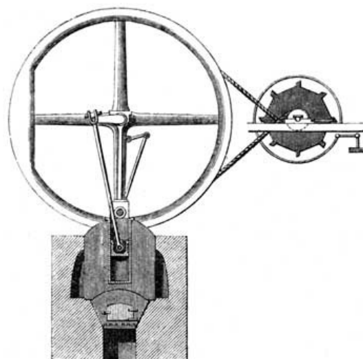
TREVITHICK'S HIGH-PRESSURE STEAM-PUFFER THRASHING ENGINE, 1812.
