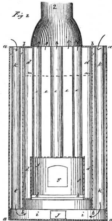
FIG. 2.—ELEVATION SECTION. [174]
