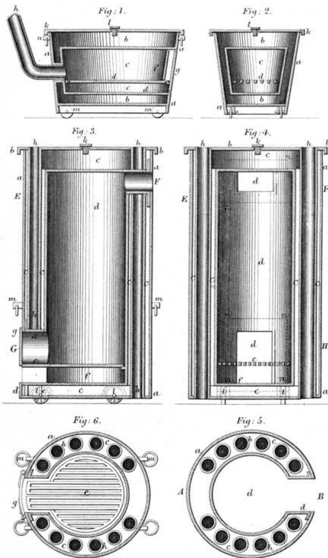
PLATE 16. HEATING APPARATUS.
