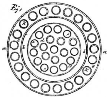
FIG. 1.—PLAN SECTION.
