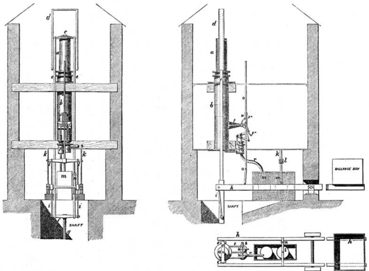
WHEAL PROSPER HIGH-PRESSURE EXPANSIVE STEAM-CONDENSING POLE-ENGINE, 1811.
