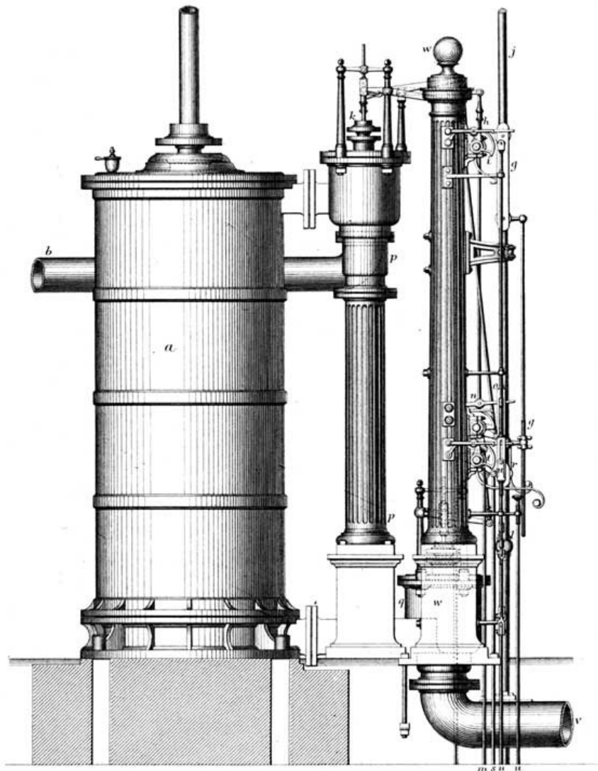
PLATE 13. LA BELLE MACHINE. HIGH PRESSURE STEAM EXPANSION PUMPING ENGINE.—1836.
