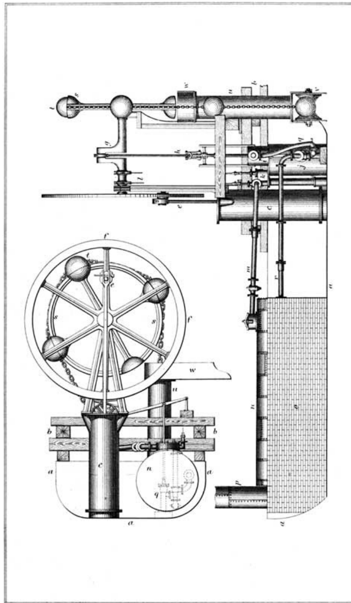
PLATE 15 TREVITHICK'S CHAIN AND BALL PUMP.
