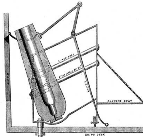
TREVITHICK'S GUN-CARRIAGE AND FRICTION SLIDES, 1827.
