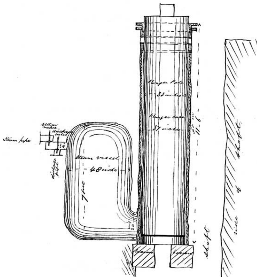
POLE-ENGINE.
