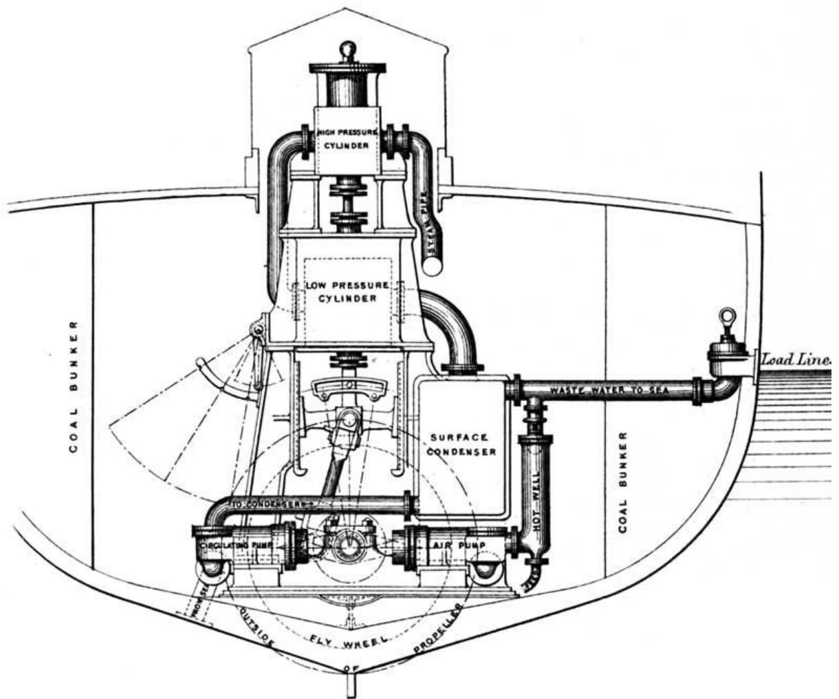
PLATE 18. COMPOUND MARINE ENGINE, 1871.
