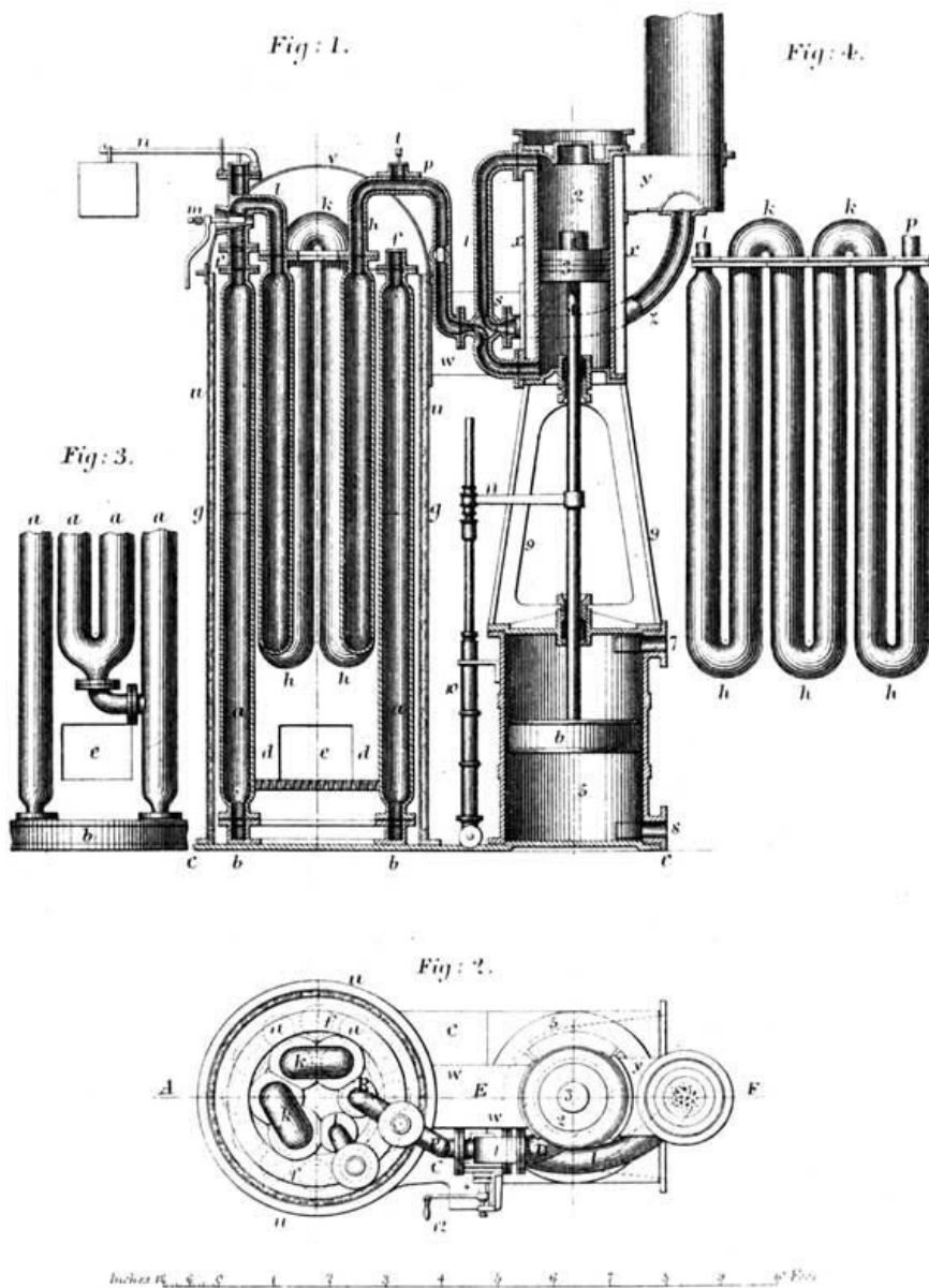
PLATE 17. TREVITHICK'S PATENT BOILER AND ENGINE, 1832.
