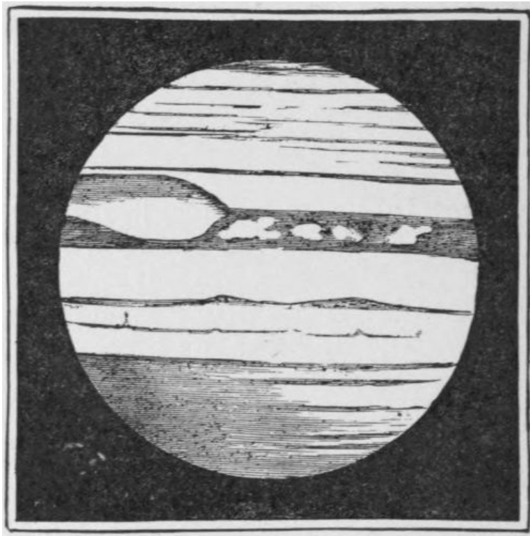
FIG. 14.—Jupiter, November 27, 1857 (Dawes).
