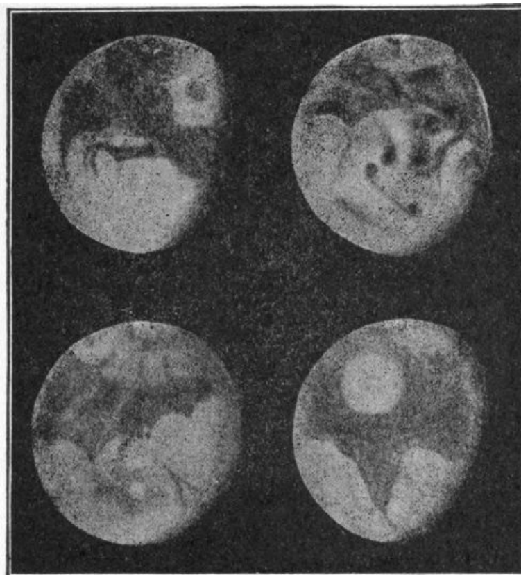
FIG. 12.—Four views of Mars differing 90° in longitude (Barnard).
