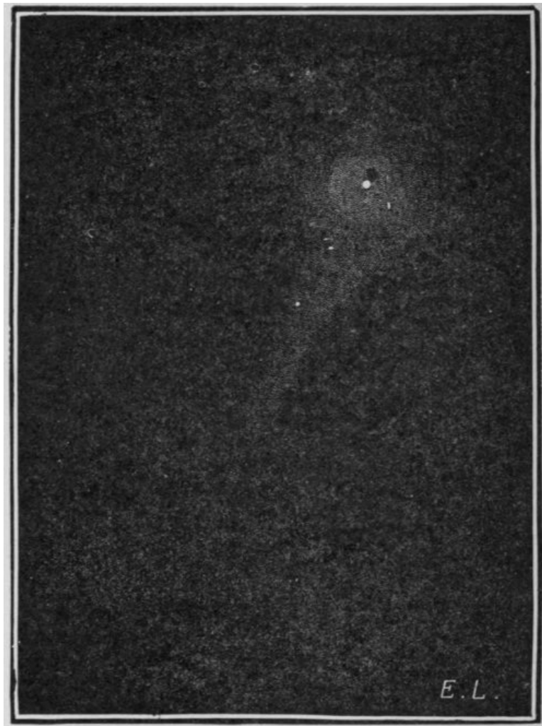
FIG. 21.—Quenisset's Comet, July 9, 1893 (Quenisset).
