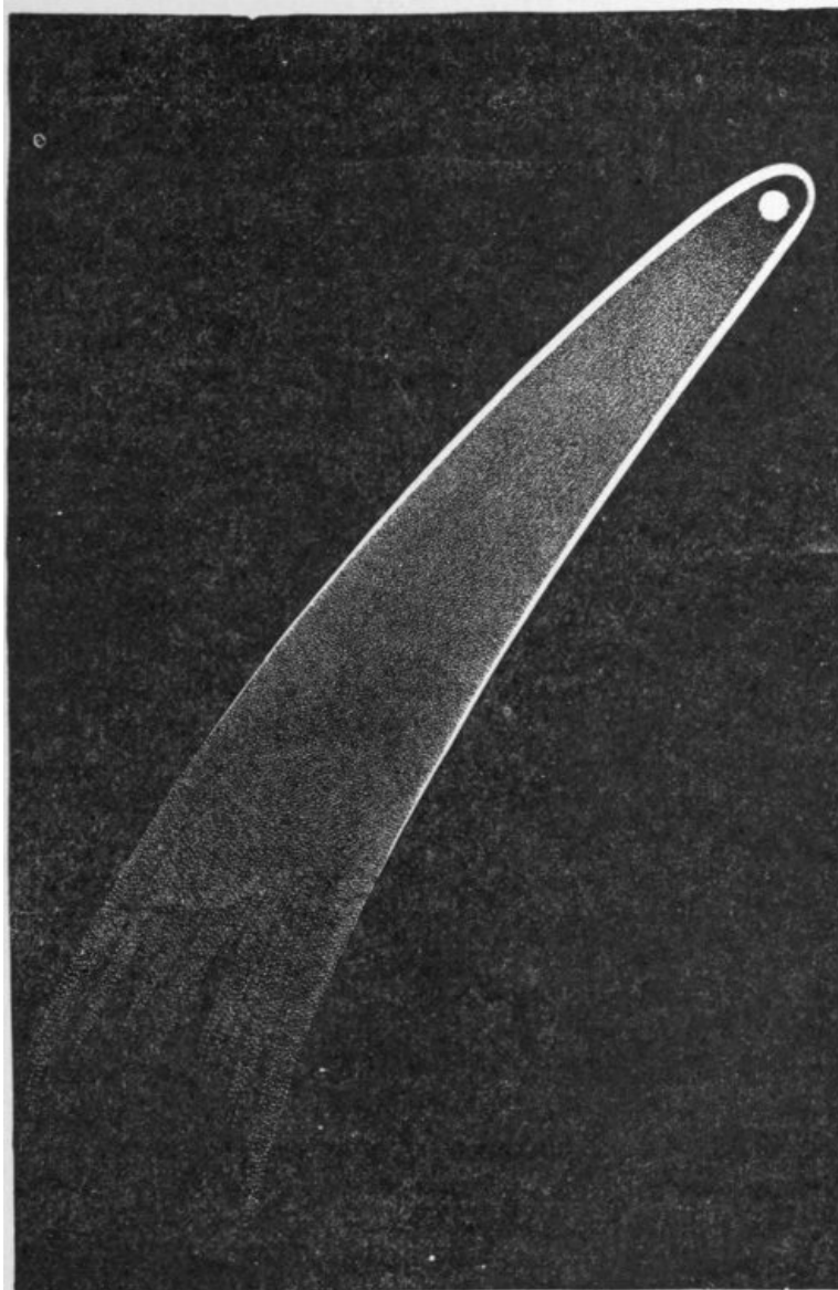
FIG. 27.—The Great Comet of 1811.
