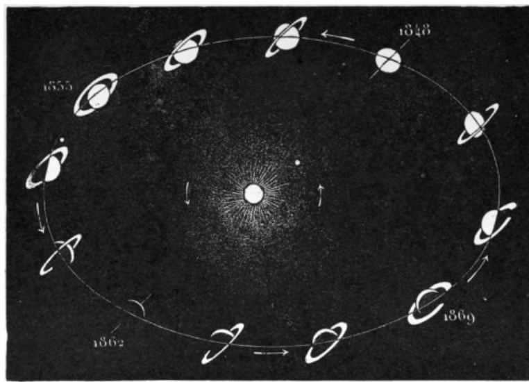
FIG. 17.—Phases of Saturn's Rings at specified dates.
