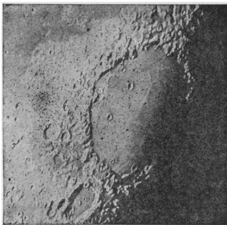
FIG. 11.—Mare Crisium. (Lick Observatory photographs.)
