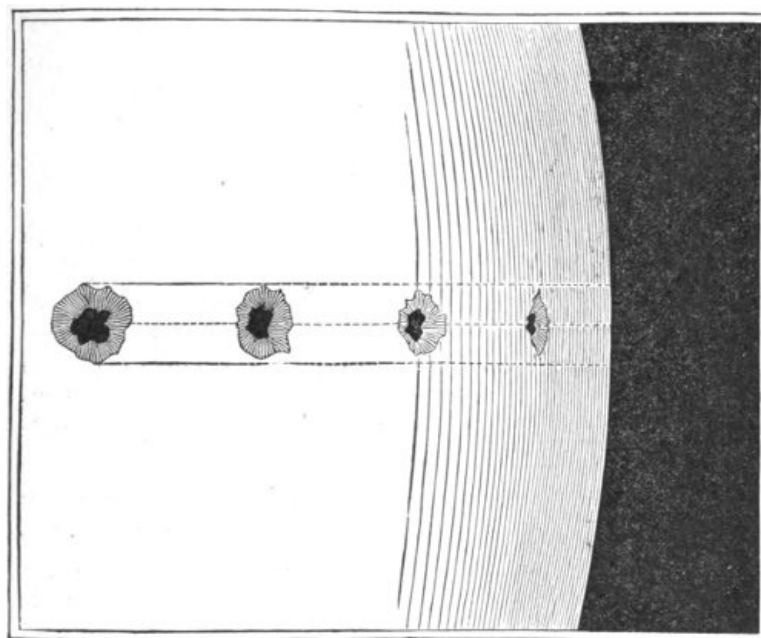
FIG. 6.—Change of Form in Sun-spots owing to the Sun's rotation. 29
