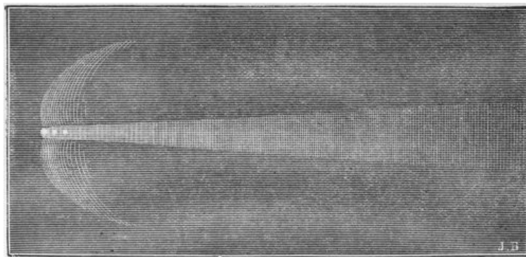
FIG. 25.—Sawerthal's Comet, June 4, 1888 (Charlois).
