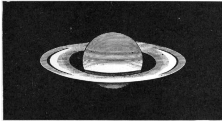
FIG. 15.—Saturn, Jan. 26, 1889 (Antoniadi).
