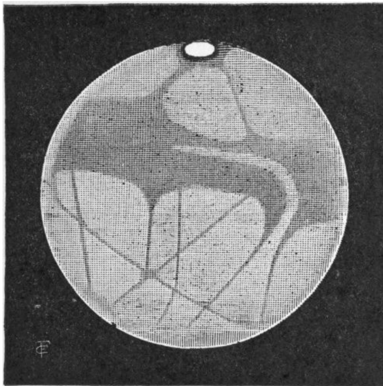
FIG. 13.—Mars, August 27, 1892 (Guiot).
