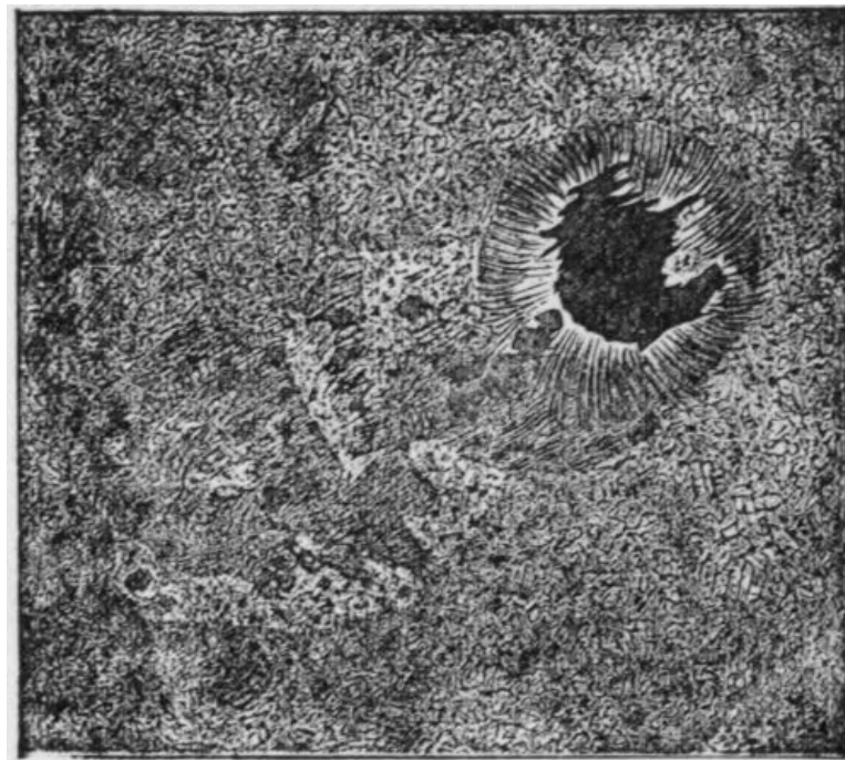
FIG. 5.—Ordinary Sun-spot, June 22, 1885. 22
