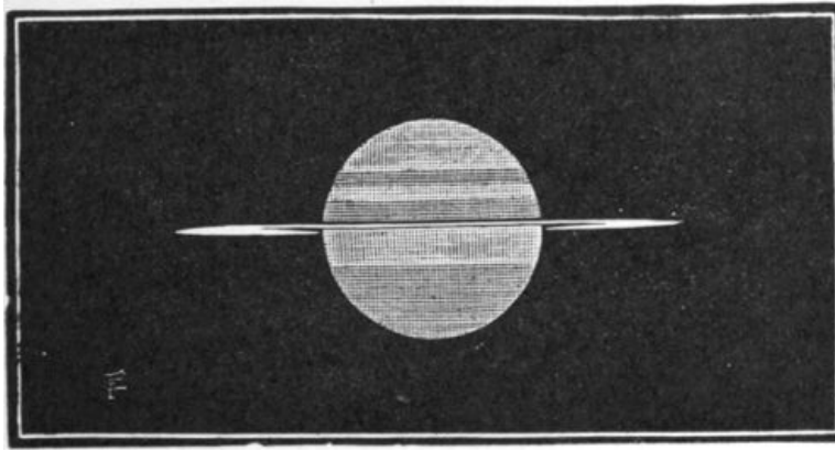
FIG. 18.—Saturn with the shadow of Titan on it, March 11, 1892 (Terby).
