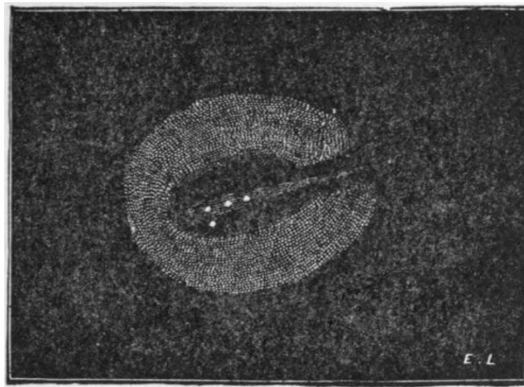
FIG. 23.—Holmes's Comet, Nov. 16, 1892 (Denning).
