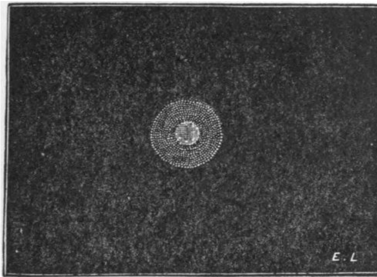
FIG. 22.—Holmes's Comet, Nov. 9, 1892 (Denning).
