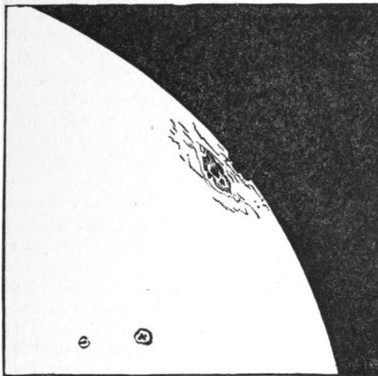
FIG. 7.—Sun-spot seen as a Notch.
