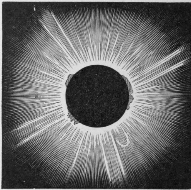
FIG. 8.—The Sun totally eclipsed, July 18, 1860 (Feilitzsch).
