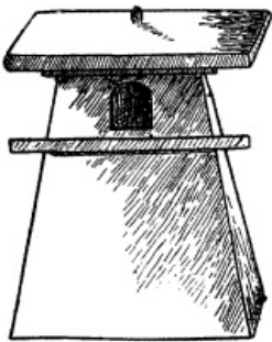
Made of rough boards. Size, 6 inches high, 5 1/2 inches square at the bottom, 3 1/2 inches square at the top.
