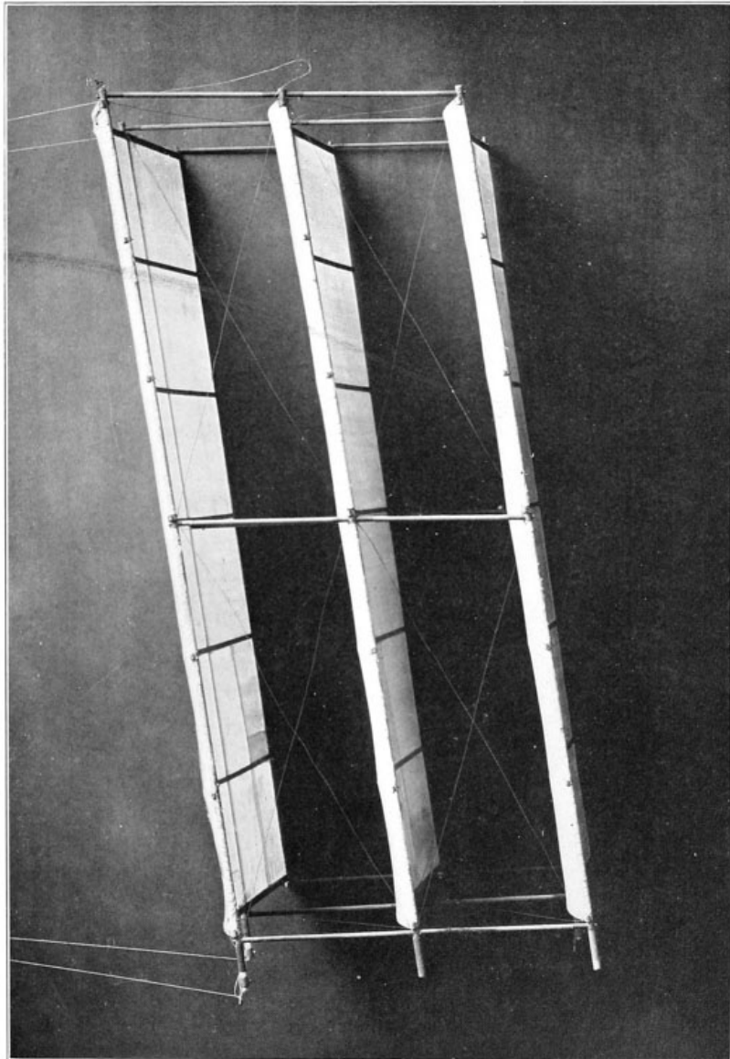
PL. 65. EXPERIMENTAL TYPE OF SUPERPOSED WINGS, MARCH 2, 1899 ◊
