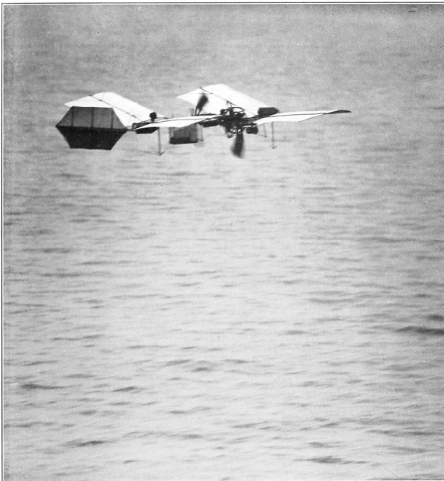
PL. 92. QUARTER-SIZE MODEL AERODROME IN FLIGHT, AUGUST 8, 1903 ◊
