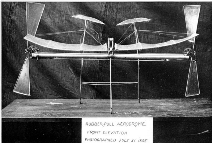
PL. 7. RUBBER-PULL MODEL AERODROME ◊
