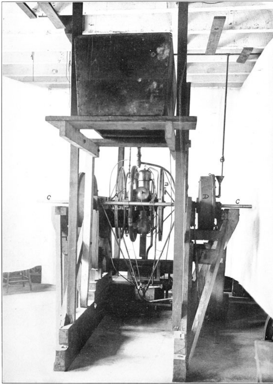
PL. 83. DYNAMOMETER TESTS OF LARGE ENGINE ◇
