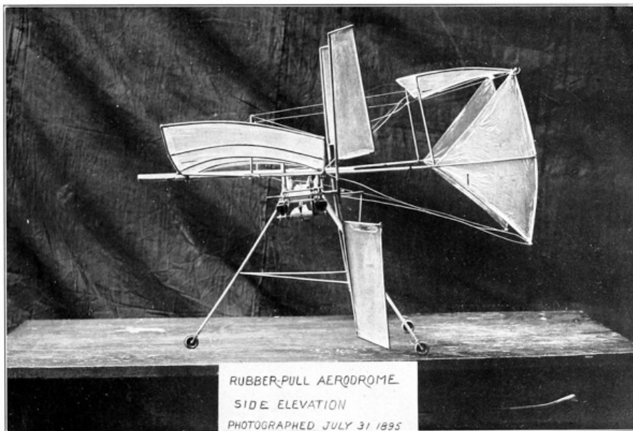
PL. 8. RUBBER-PULL MODEL AERODROME ◇
