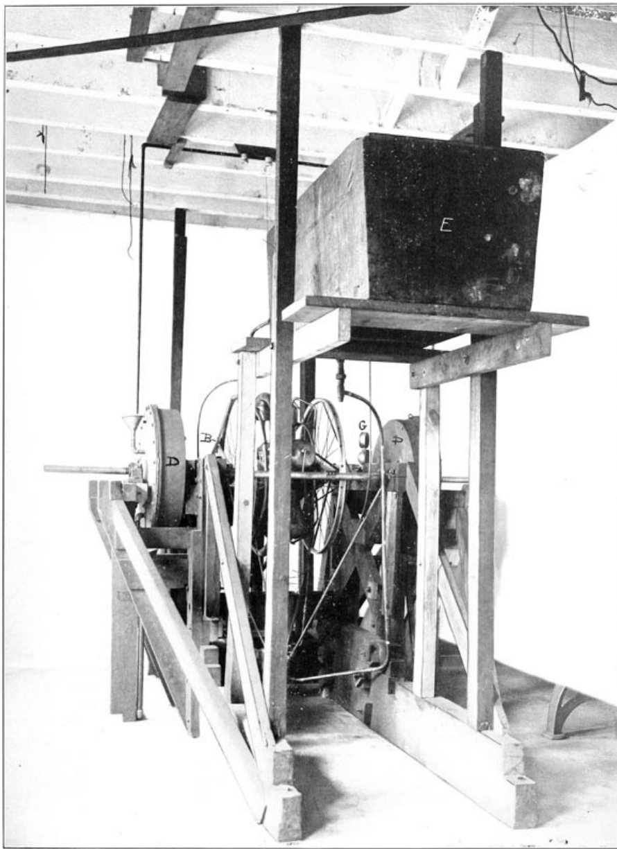
PL. 84. DYNAMOMETER TESTS OF LARGE ENGINE ◊
