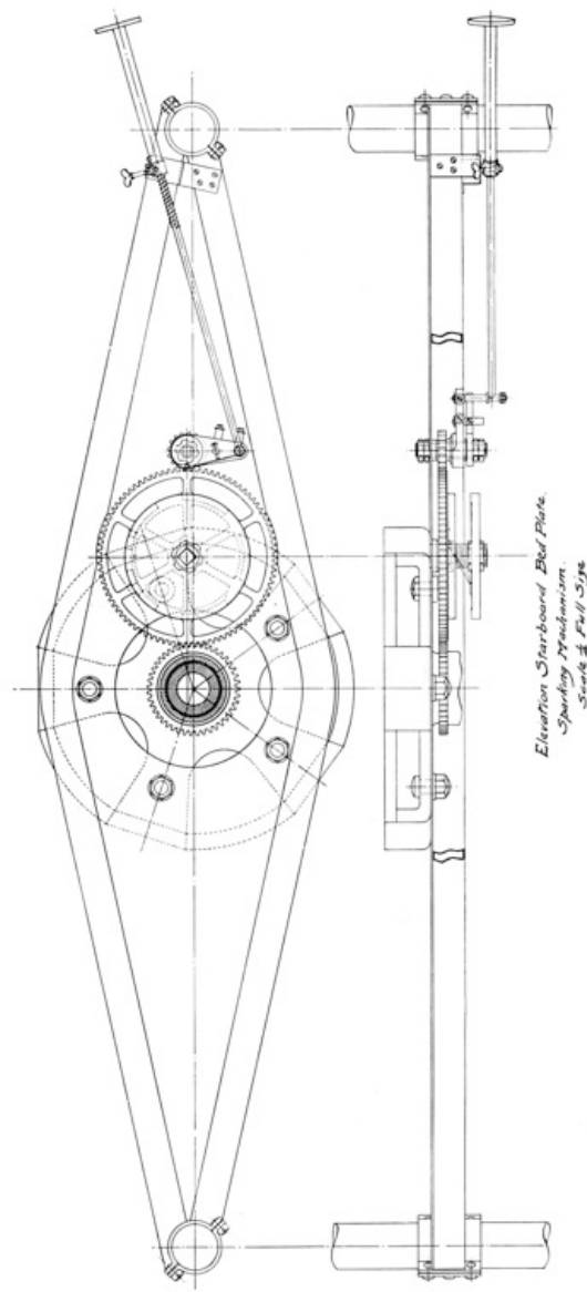
Scale \frac{1}{4} Full Size PL. 81 ENGINE OF AERODROME A. ELEVATION STARBOARD BED PLATE, SPARKING MECHANISM \diamond lgr
