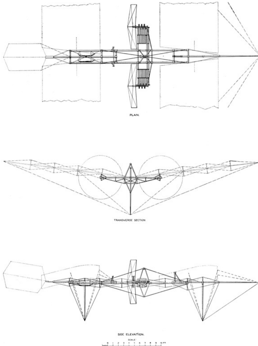
PL. 32. DRAWINGS OF PROPOSED MAN-CARRYING AERODROME, 1898 ◇ lgr
