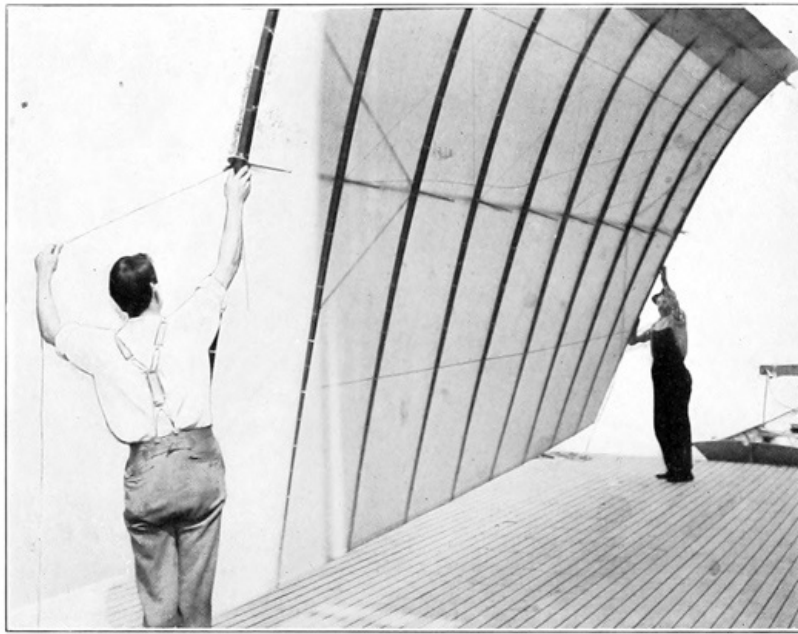
PL. 94. HOISTING WING OF FULL-SIZE AERODROME ◇
