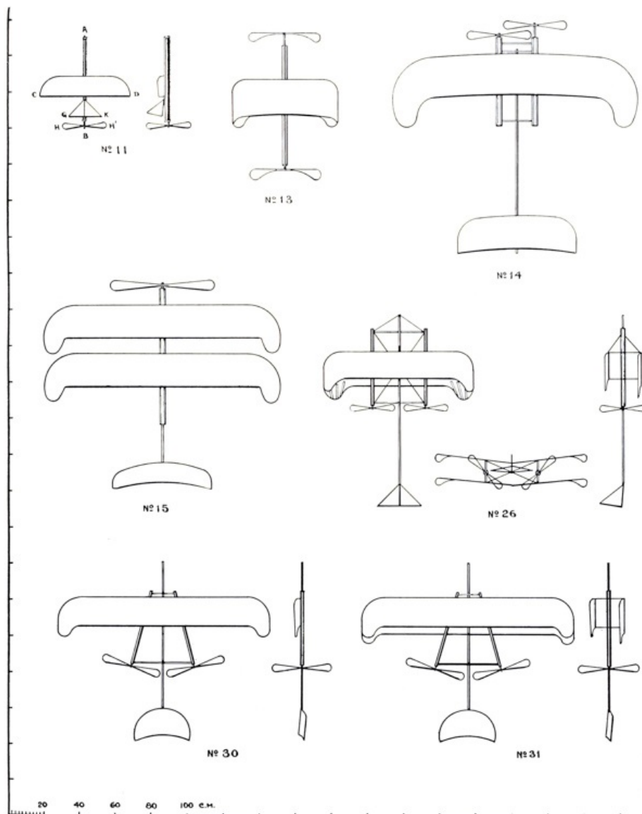
PL. 1. RUBBER-MOTOR MODEL AERODROMES NOS. 11, 13, 14, 15, 26, 30, 31 ◊
