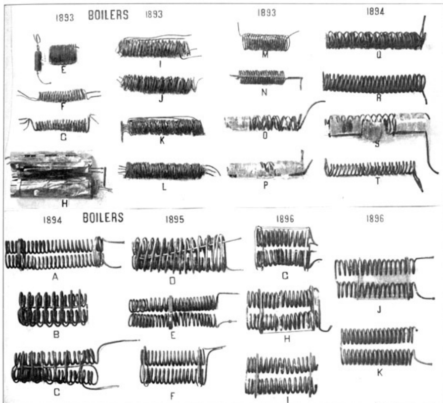
PL. 13. BOILERS OF AERODROMES ◊
