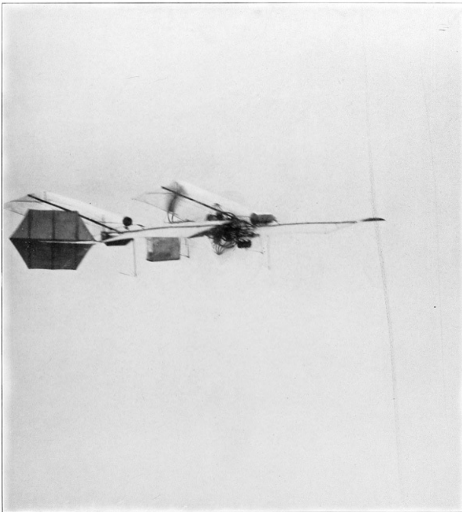
PL. 90. QUARTER-SIZE MODEL AERODROME IN FLIGHT, AUGUST 8, 1903 ◇
