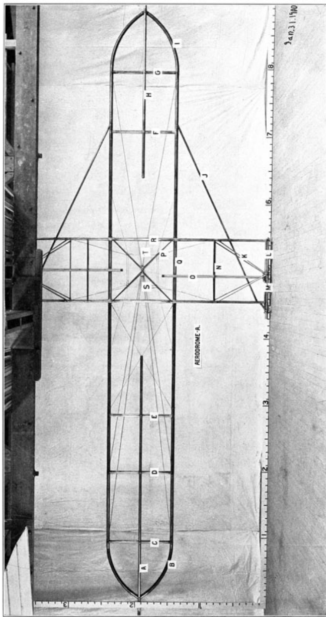
PL. 45. FRAME OF AERODROME A, JANUARY 31, 1900 ◊
