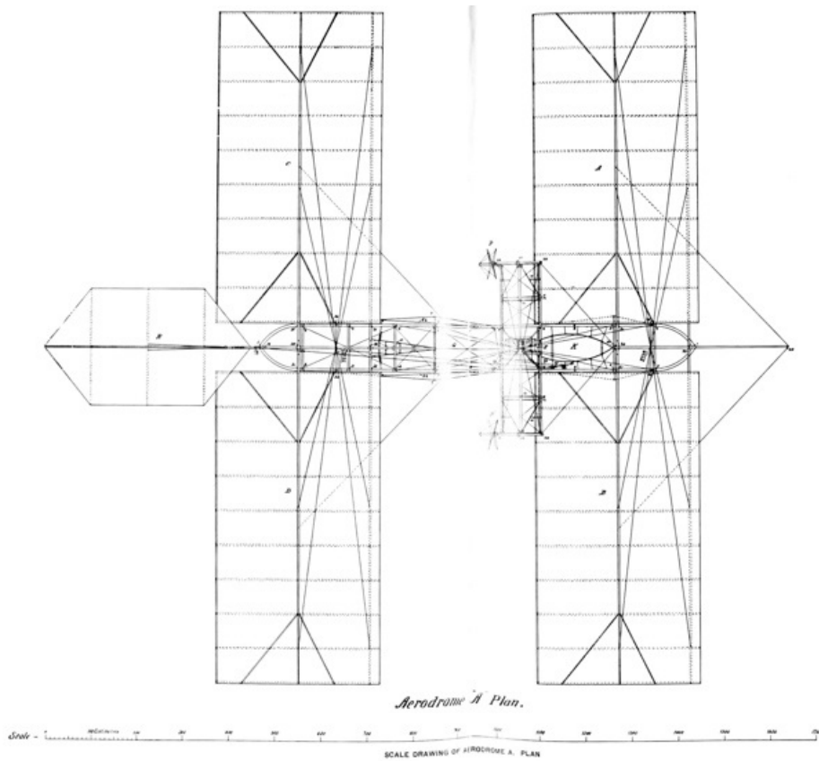
PL. 54. SCALE DRAWING OF AERODROME A, PLAN \diamond lgr
