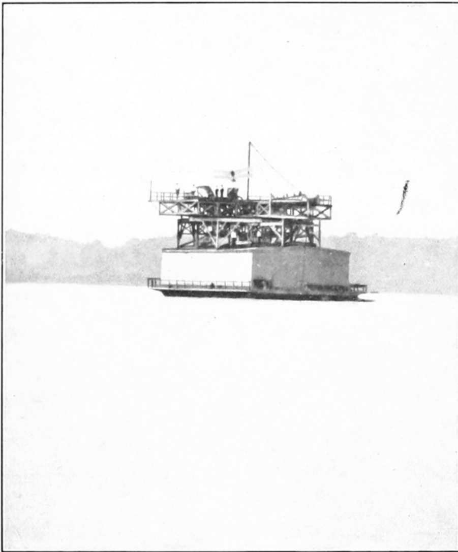
PL. 87. QUARTER-SIZE MODEL AERODROME IN FLIGHT, AUGUST 8, 1903 ◇
