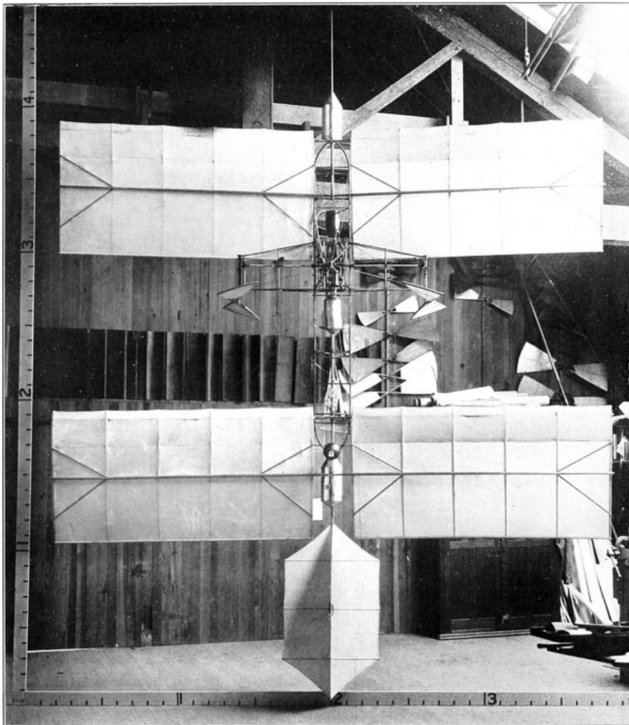
PL. 71. PLAN VIEW OF QUARTER-SIZE MODEL AERODROME ◊
