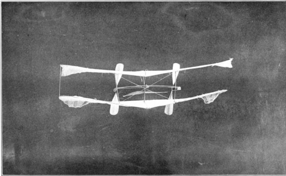
PL. 4. RUBBER-MOTOR MODEL AERODROME NO. 26 ◇
