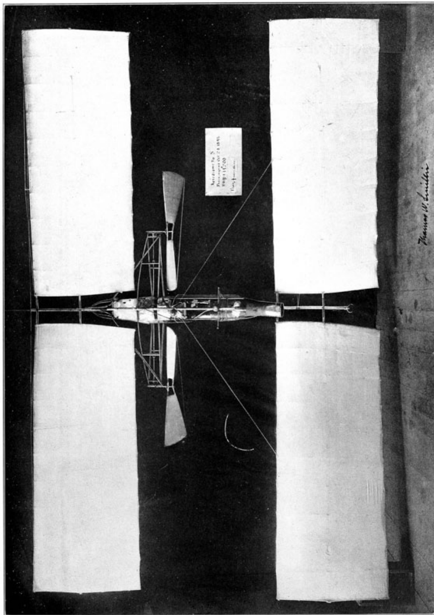
PL. 27B. AERODROME NO. 5 PLAN VIEW. OCTOBER 24, 1896 ◊
