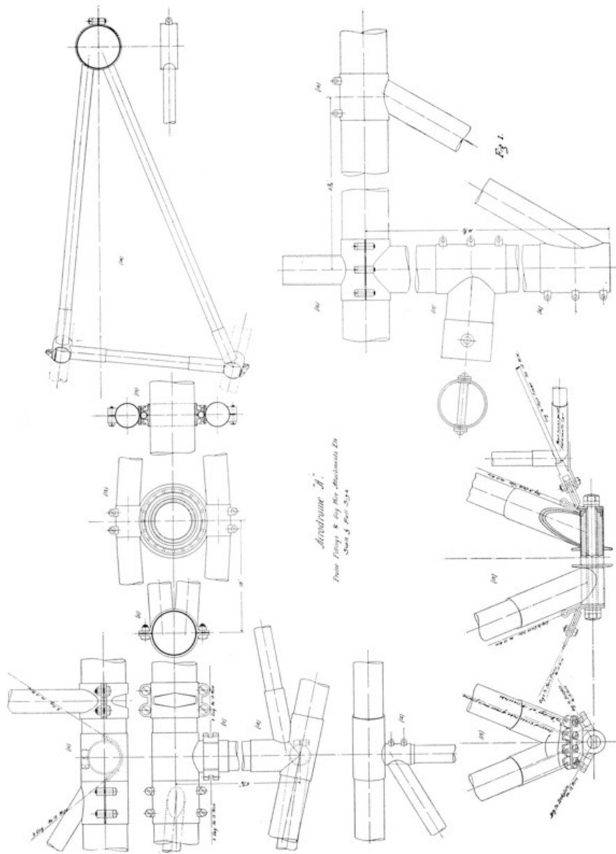
PL. 56. FRAME FITTINGS AND GUY-WIRE ATTACHMENTS, ETC. ◇ lgr
