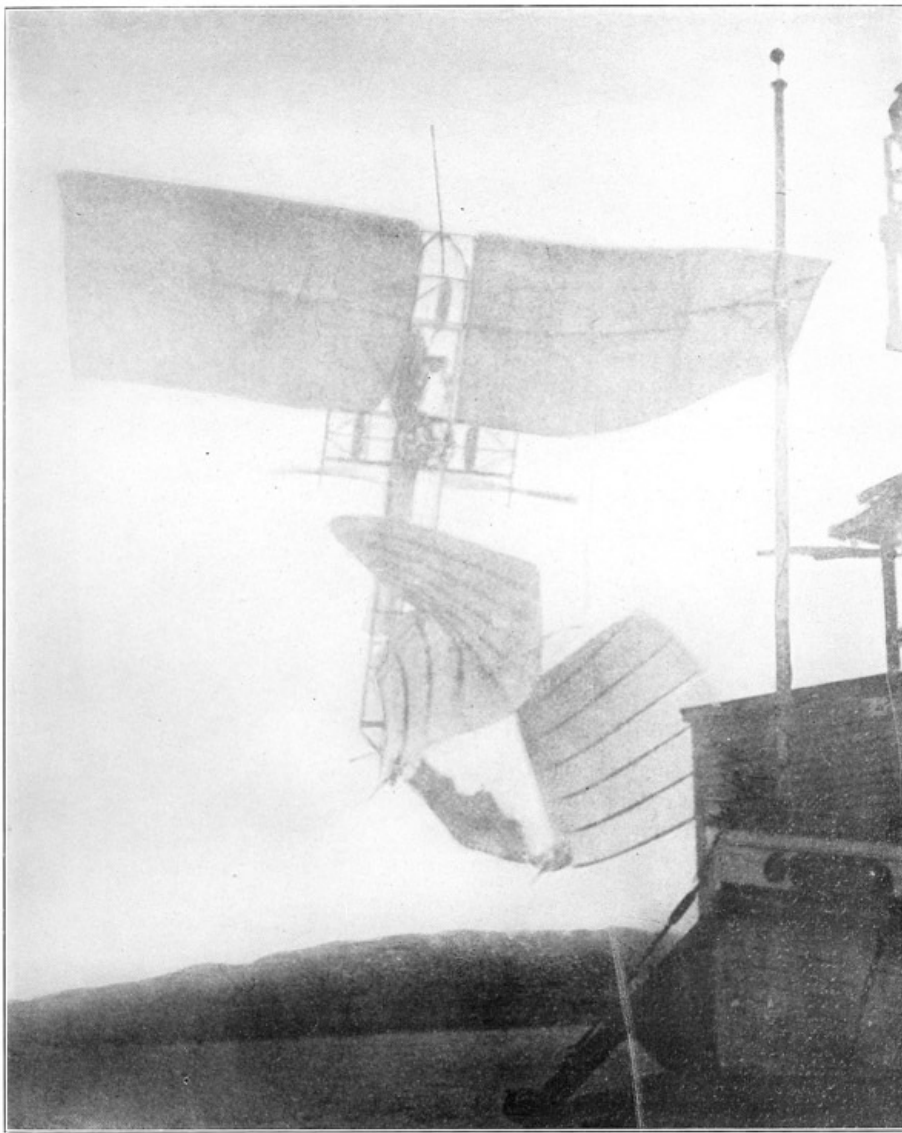
PL. 101. ATTEMPTED LAUNCHING OF AERODROME, DECEMBER 8, 1903 ◇ ENLARGEMENT OF PHOTOGRAPH BY THE WASHINGTON STAR
