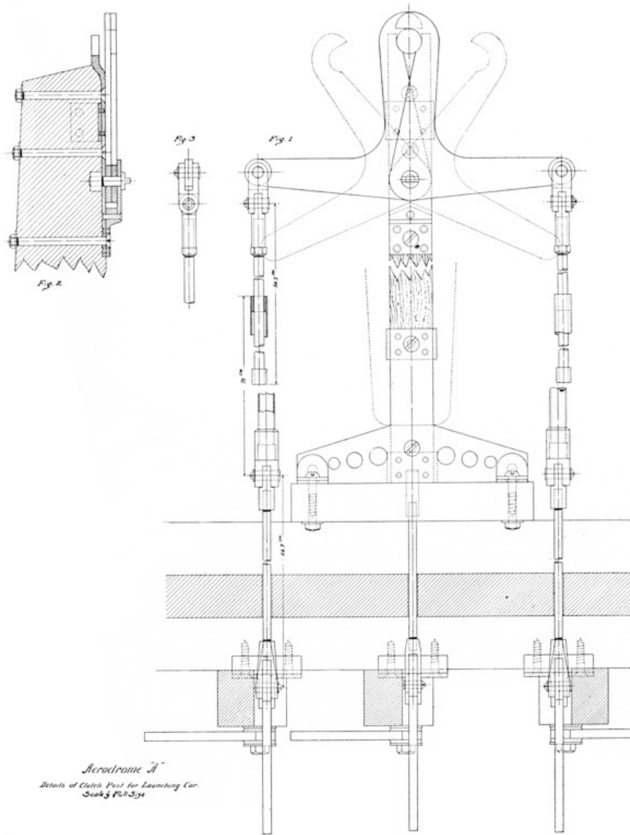
PL. 42. DETAILS OF CLUTCH POST FOR LAUNCHING-CAR ◊ lgr
