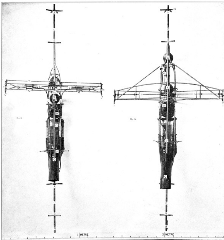
PL. 30. PLAN VIEW OF STEEL FRAMES AND POWER PLANTS OF AERODROMES NOS. 5, 6 ◇ lgr
