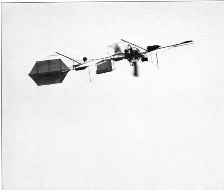
PL. 91. QUARTER-SIZE MODEL AERODROME IN FLIGHT, AUGUST 8, 1903 ◇
