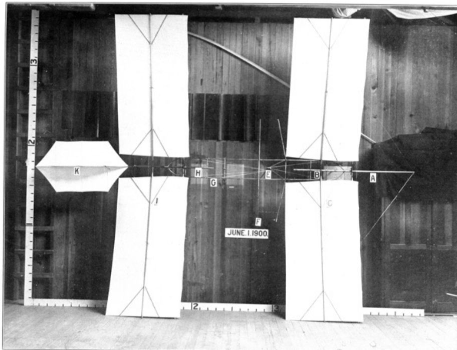
PL. 70. PLAN VIEW OF QUARTER-SIZE MODEL AERODROME, JUNE 1, 1900 ◊
