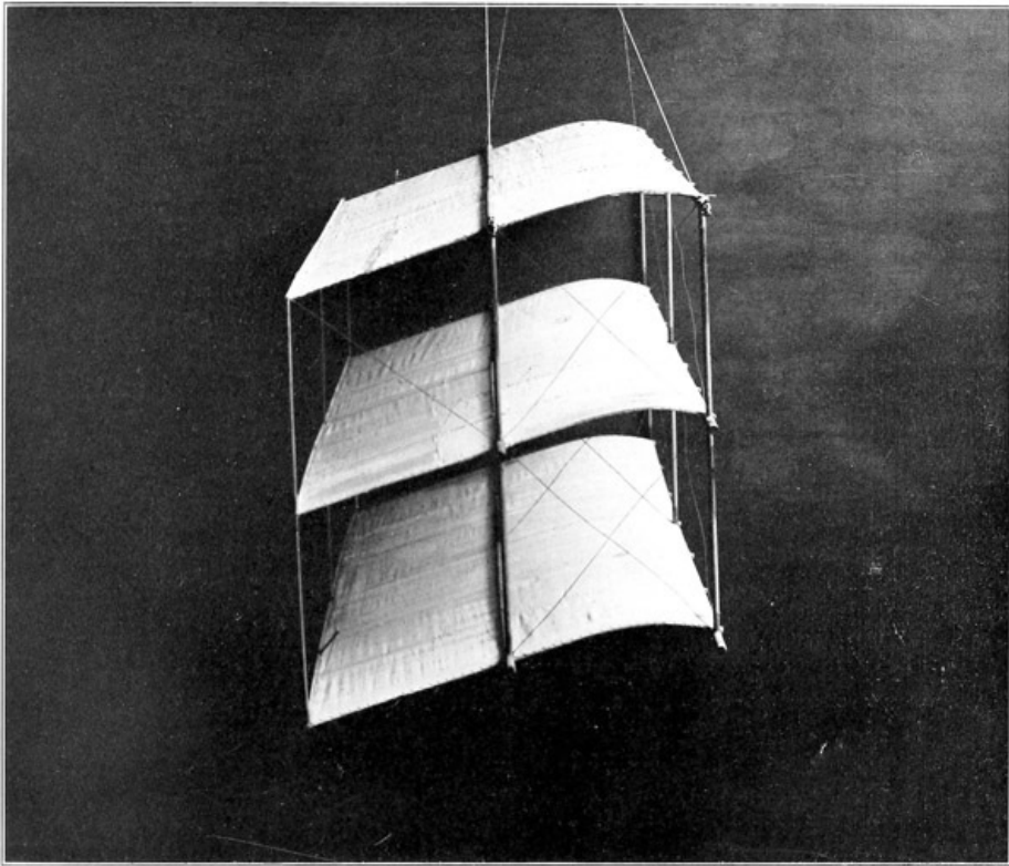
PL. 64. EXPERIMENTAL TYPE OF SUPERPOSED WINGS, MARCH 2, 1899 ◊
