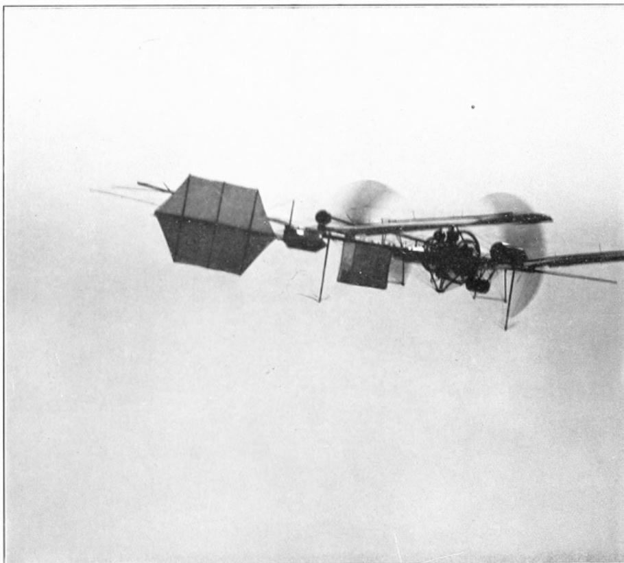
PL. 89. QUARTER-SIZE MODEL AERODROME IN FLIGHT, AUGUST 8, 1903 ◇
