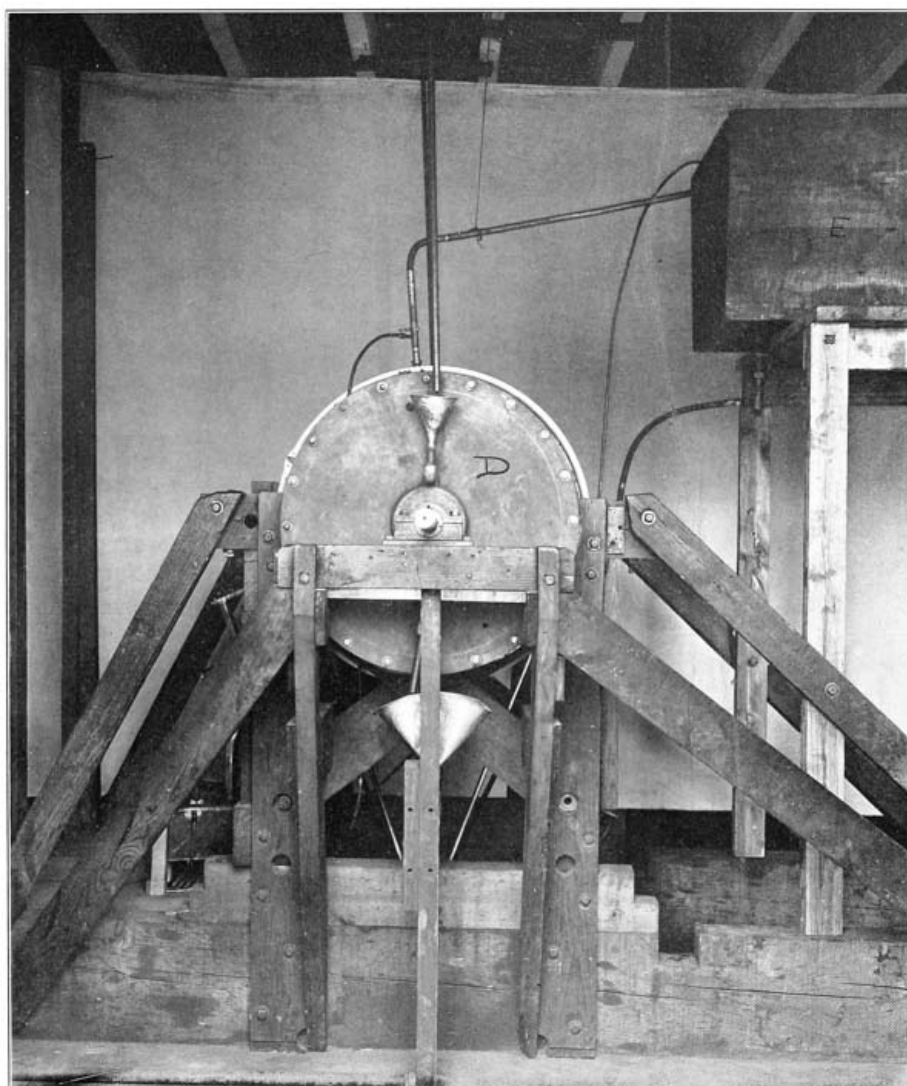
PL. 82. DYNAMOMETER TESTS OF LARGE ENGINE ◊
