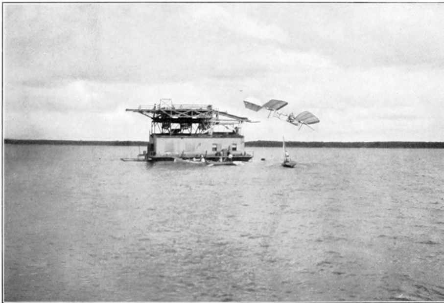
PL. 95. FLIGHT OF LARGE AERODROME, OCTOBER 7, 1903 ◊
