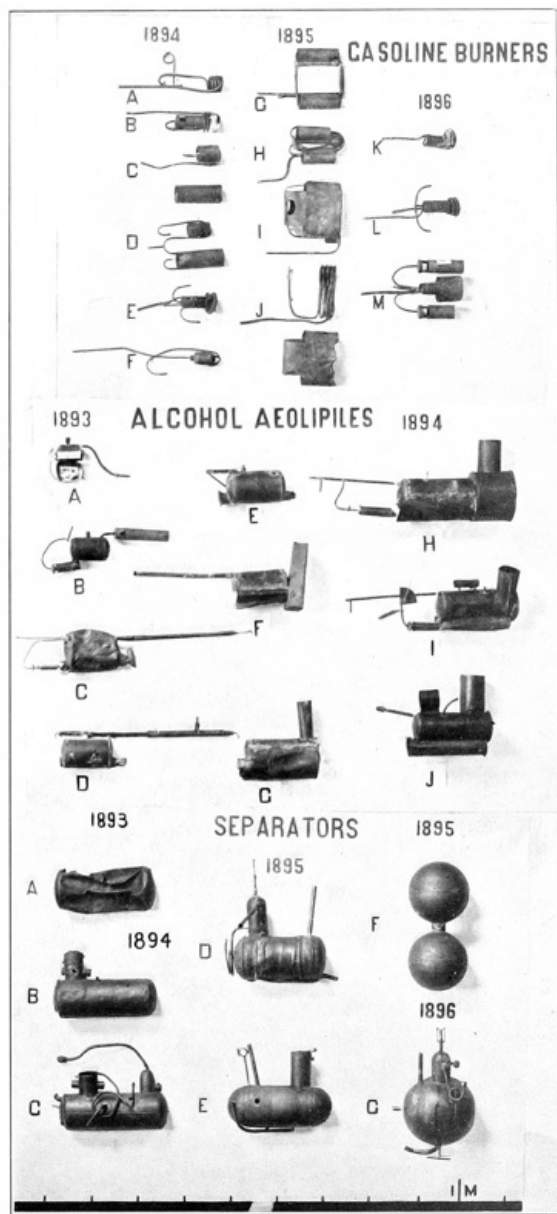
PL. 12. BURNERS, AEOLIPILES, AND SEPARATORS ◊
