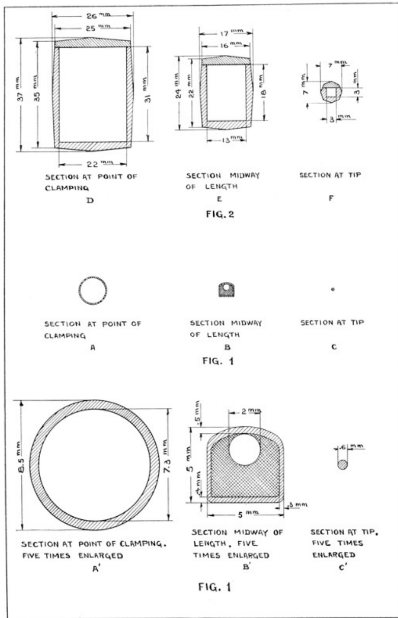
PL. 67. CROSS SECTION OF RIBS \diamond lgr
