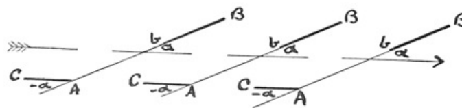
FIG. 6. Diagram showing effect of Pénaud tail.
