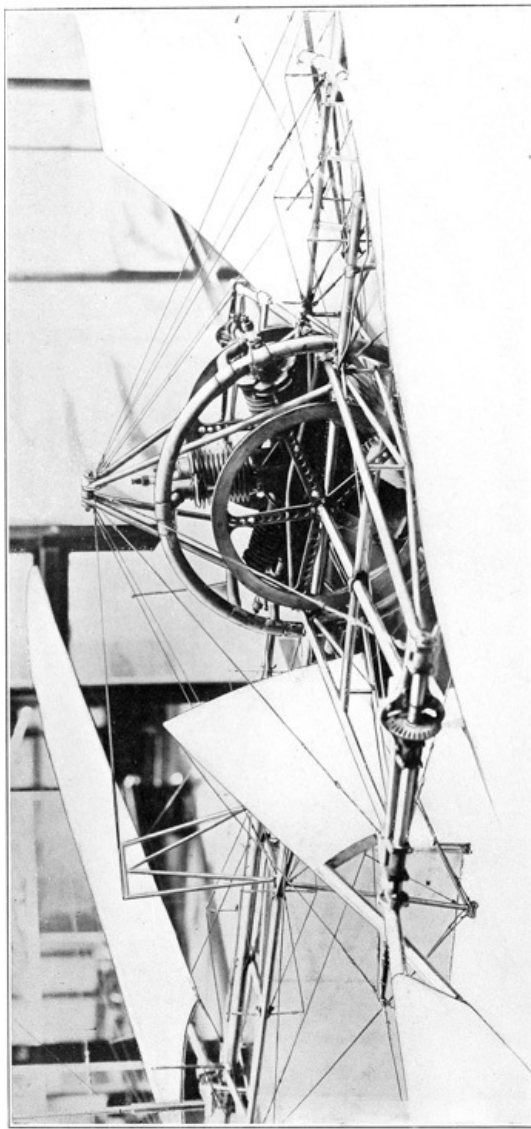
PL. 77. CYLINDERS OF ENGINE OF QUARTER-SIZE MODEL AERODROME ◇
