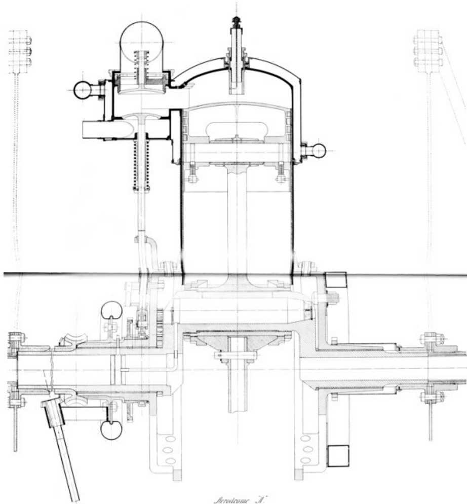
Aerodrome A. 5" Cylinder by 5 1/2" Stroke Engine. Section through Cylinder & Drum. See Fig. 20.
