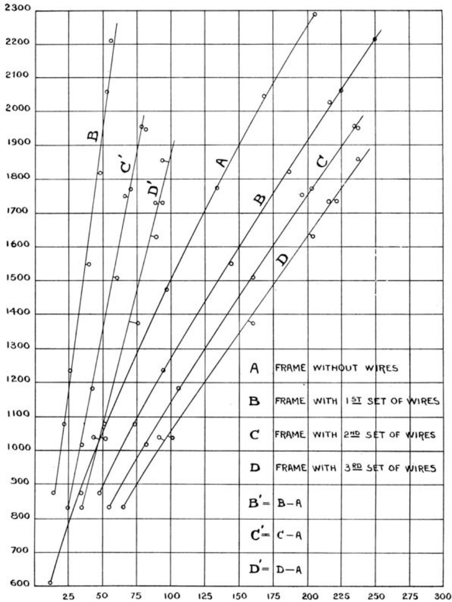
PL. 44. RESISTANCE OF WIRES AT GIVEN VELOCITIES ◊
