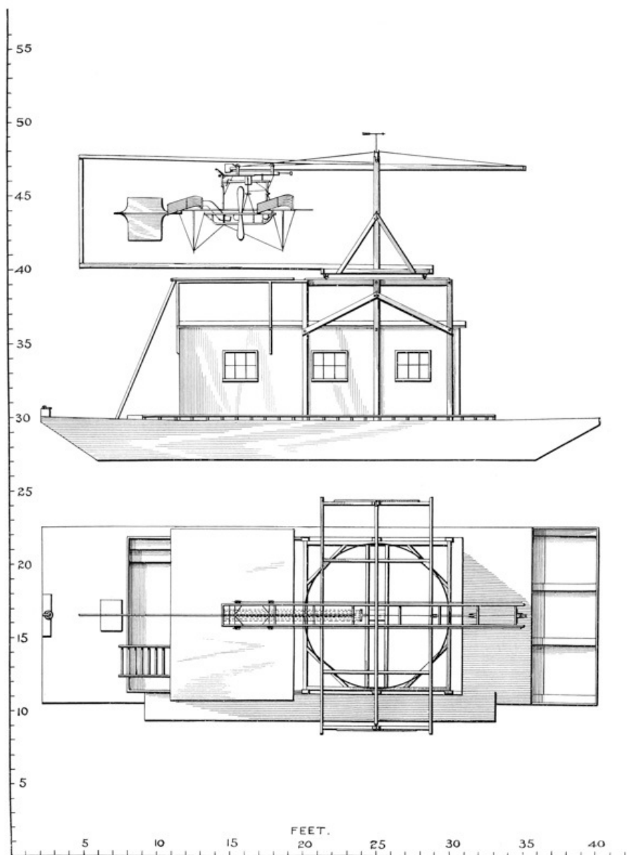
PL. 18. HOUSE-BOAT WITH OVERHEAD LAUNCHING APPARATUS, 1896 ◊
