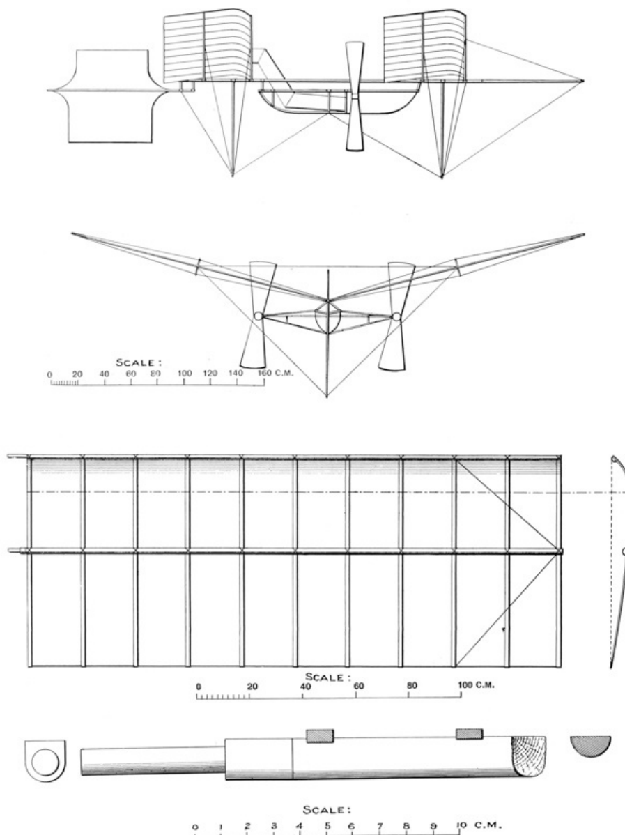
PL. 17. AERODROME NO. 5. PLAN OF WINGS AND SYSTEM OF GUYING \diamond
