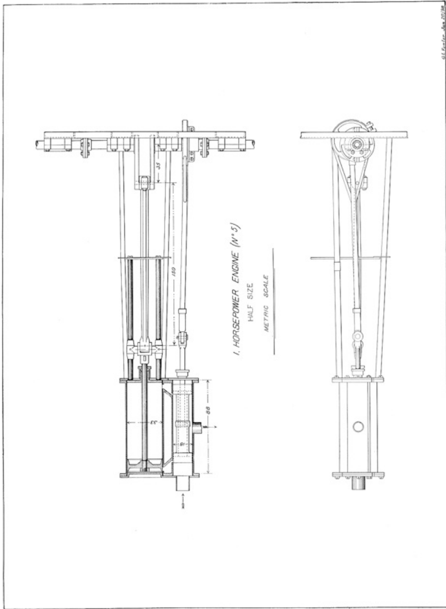
PL. 26B. DIMENSIONED DRAWING OF ENGINE NO. 5 ◇ lgr
