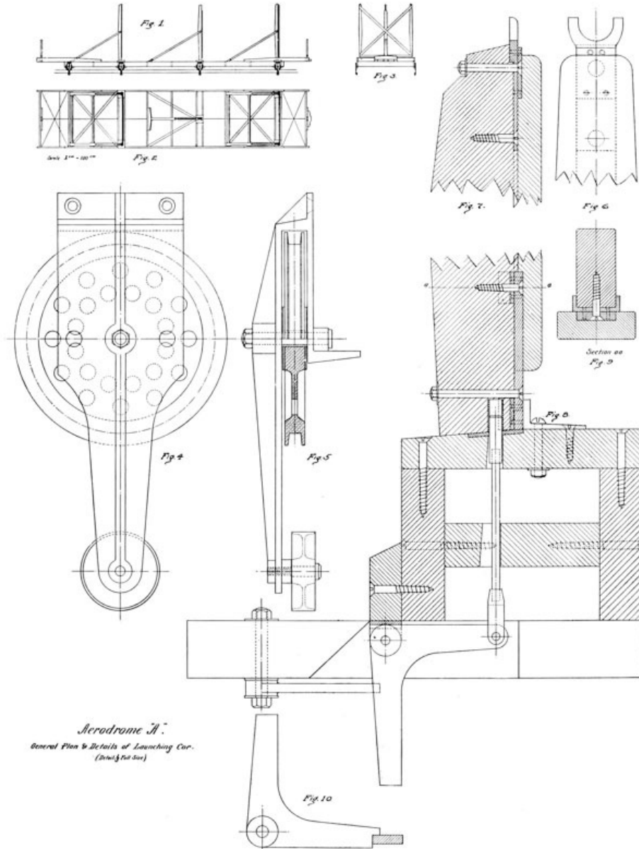
Aerodrome "A." (Details \frac{1}{2} Full Size)
