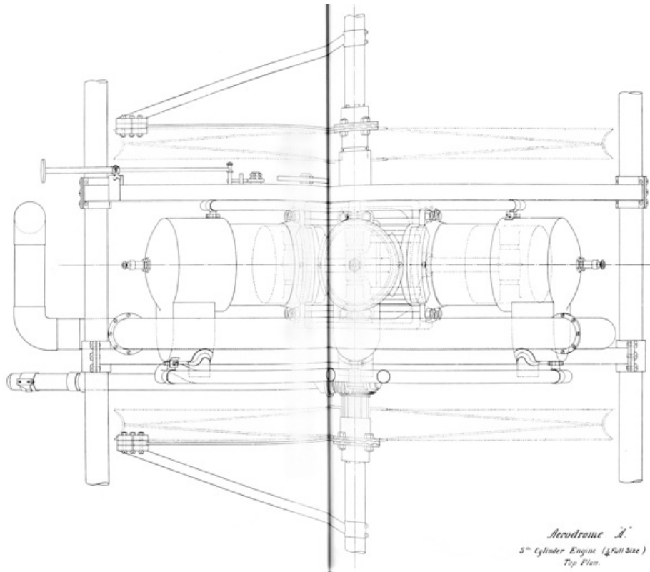
5 th Cylinder Engine ( \frac{1}{2} Full Size) PL. 80. ENGINE OF AERODROME A. TOP PLAN \diamond lgr
