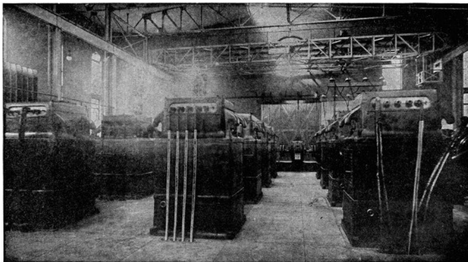
FIG. 53.—Transformers at Central Sub-station, Montreal.
