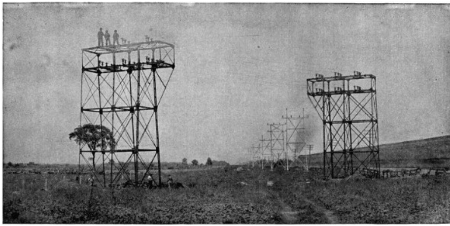
FIG. 103.—Angle Tower Near Bronte.
