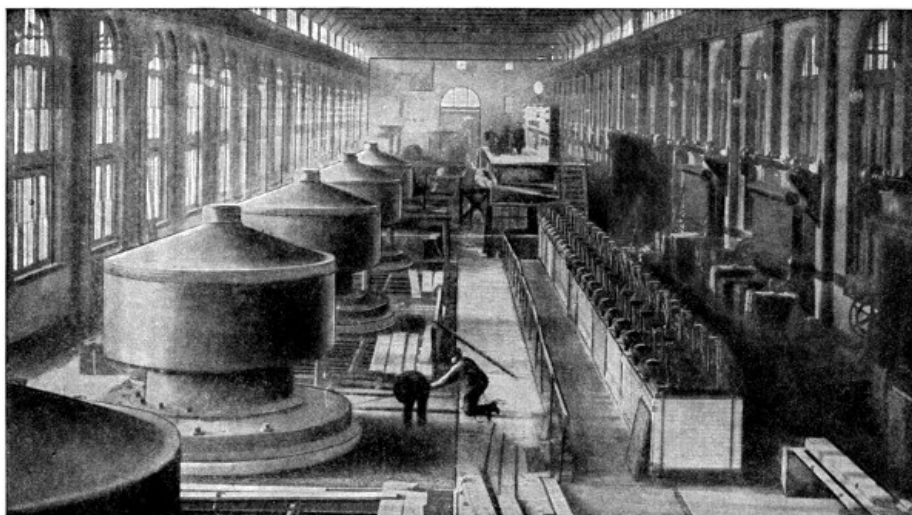
FIG. 41.—Interior of Power-house No. 2, Niagara Falls.
