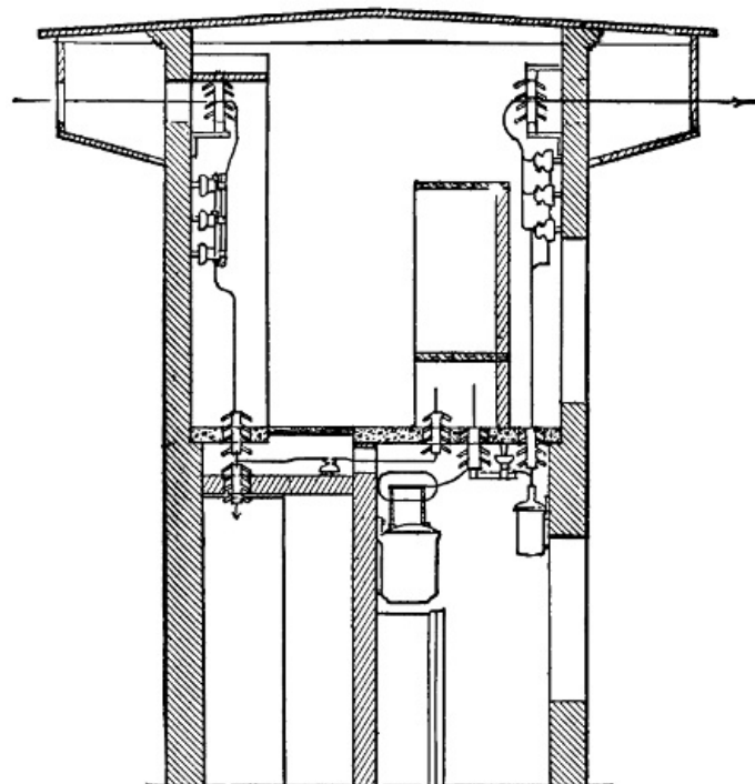
FIG. 58.—Schenectady Switch-house on Spier Falls Line.
