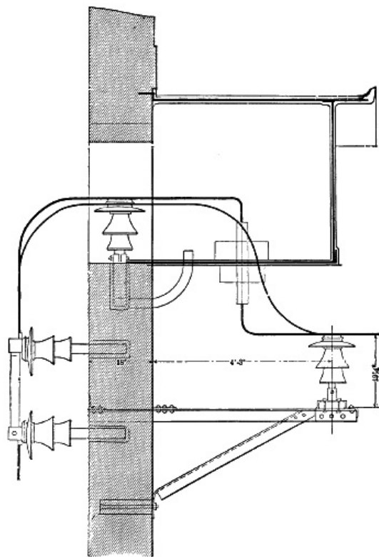
FIG. 89.—Cable Entering Building.
