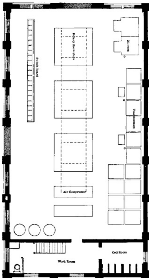
FIG. 54.—First Floor of Saratoga Sub-station.
