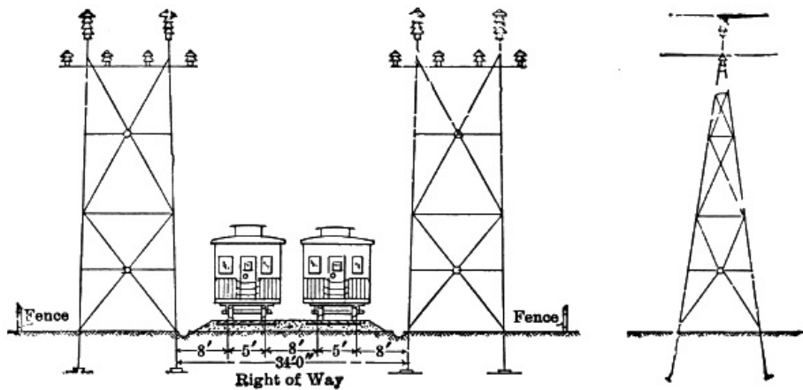
FIG. 100.—Steel Tower for Transmission Line.
