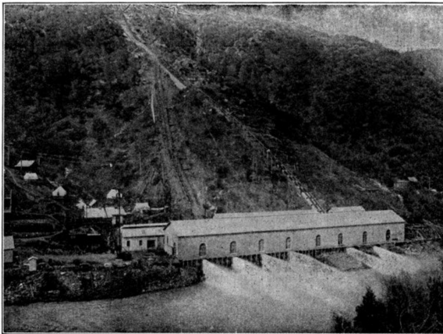
FIG. 24.—Colgate Power-house.
