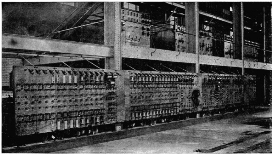
FIG. 64.—Arc-lighting Switchboard at Central Sub-station, Montreal.
