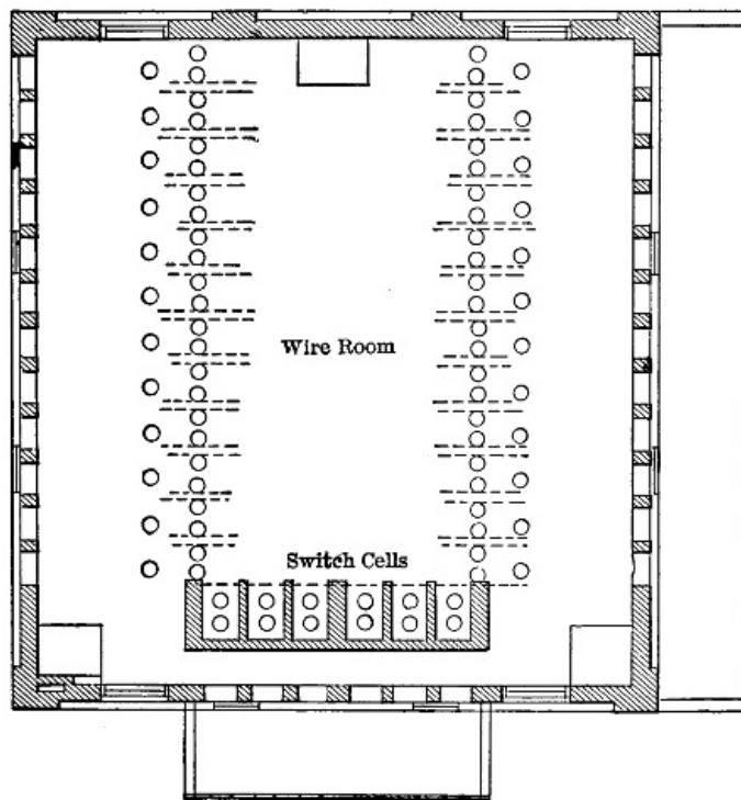
FIG. 59.—Second-floor Plan of Saratoga Switch-house on Spier Falls Line.
