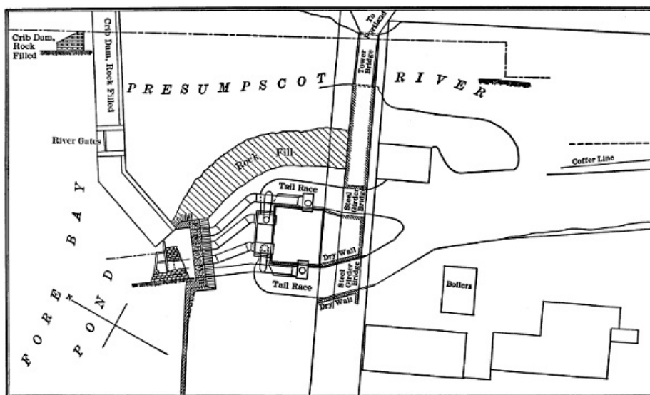
FIG. 21.—Power-house at Great Falls, Presumpscot River.
