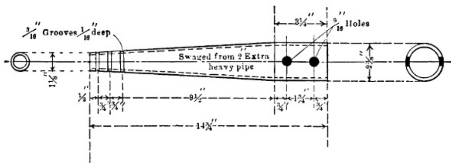
FIG. 93.—Standard Pin, Toronto and Niagara Line.
