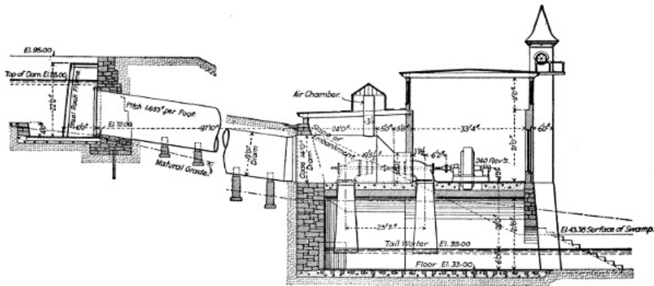
FIG. 38.—Power Plant of Ludlow Manufacturing Company.
