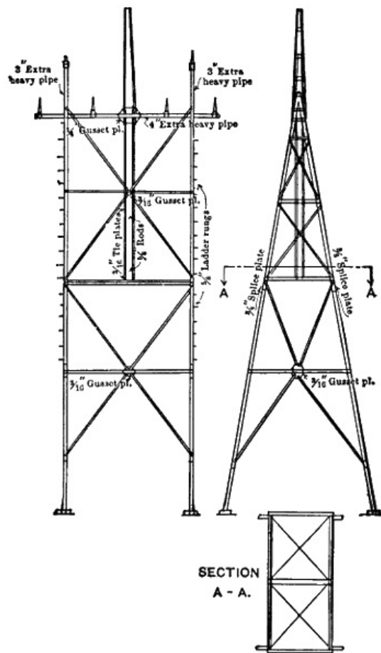
FIG. 95.—Elevations and Plan of Tower.
