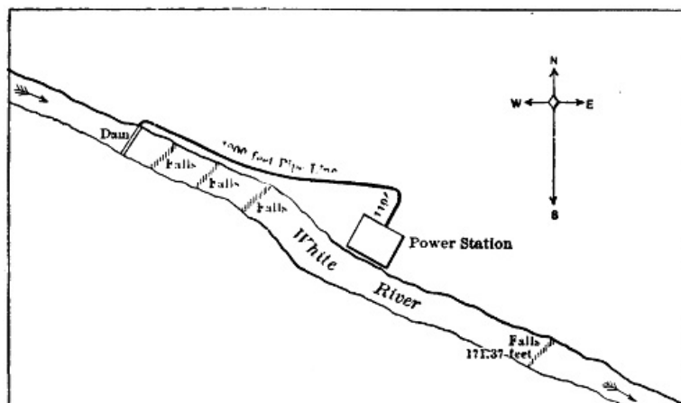
FIG. 16.—Power-house on White River, Oregon.
