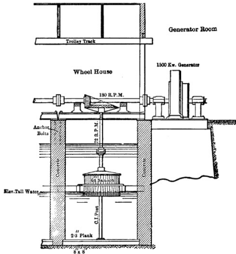
FIG. 28.—Longitudinal Section of Buchanan, Mich., Power-house.
