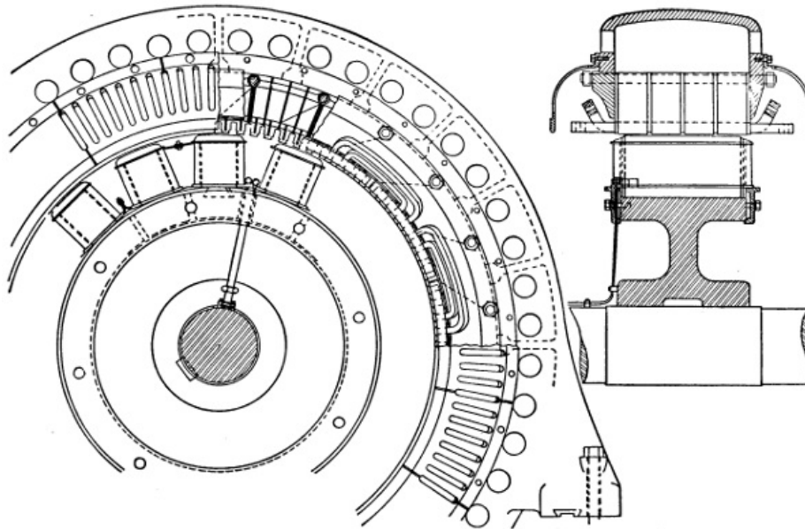
FIG. 50.—1065-Kilowatt, 2300 volt Generator Connected to Motor in Shawinigan Sub-station at Montreal.
