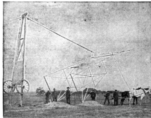
FIGS. 96, 97, 98.—Raising Towers on Niagara Transmission Line.
