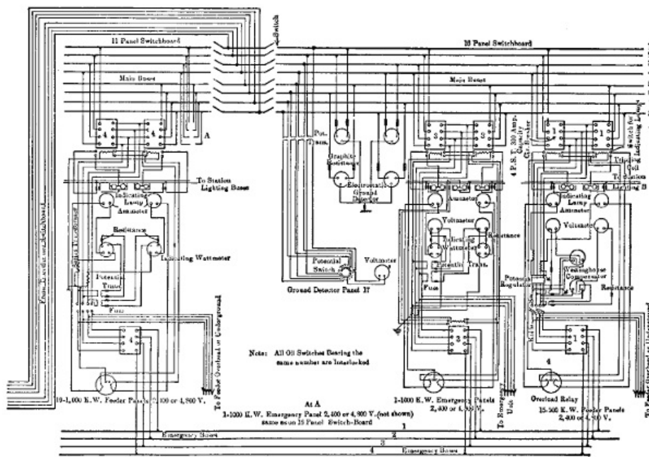
FIG. 62.—Distributing Switchboard, Central Sub-station, Montreal.
