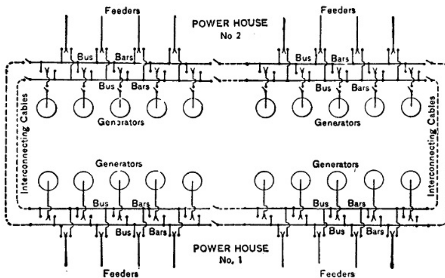
FIG. 55.—Connections between Power-houses 1 and 2 at Niagara Falls.
