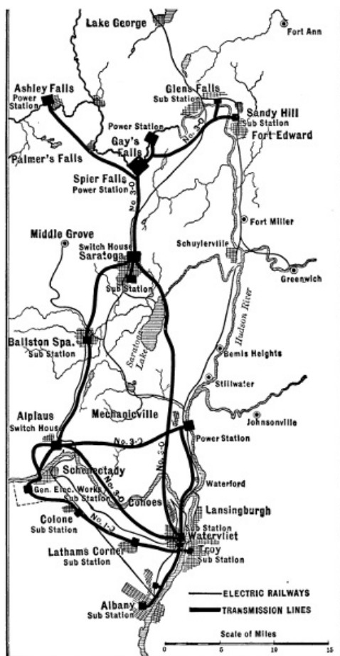
FIG. 1.—Spier Falls Transmission Lines.
