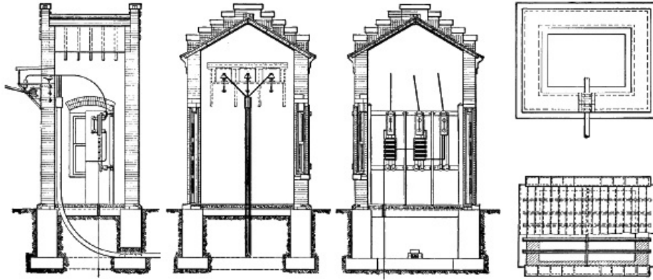
FIG. 75.—Cable Terminal House at Piscataqua River Crossing.
