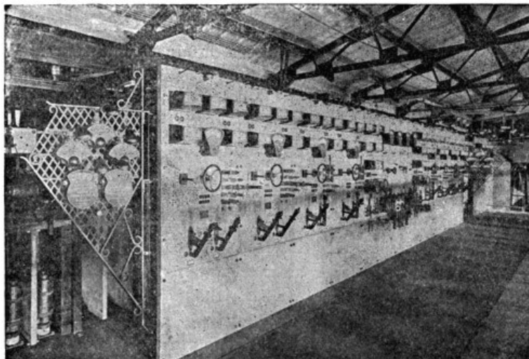
FIG. 63.—Switchboard at Chambly Power-station.
