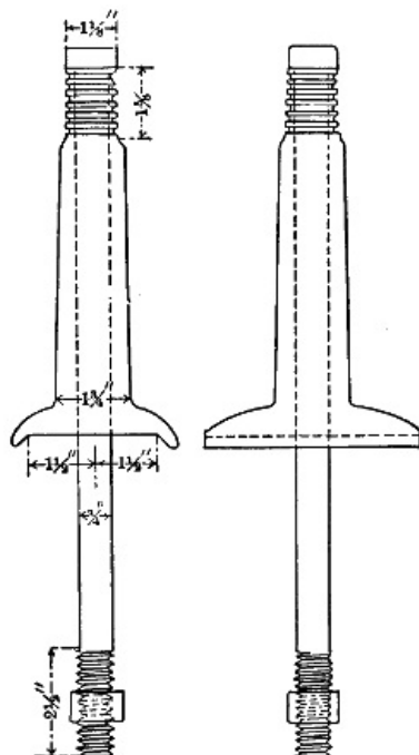
FIG. 92.—Iron Pins on Spier Falls Line.
