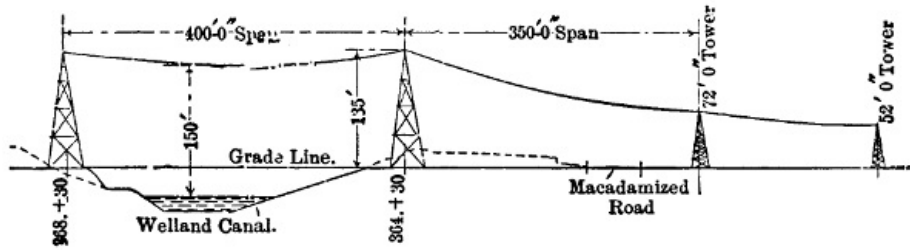
FIG. 101.—Transmission Line at Welland Canal.
