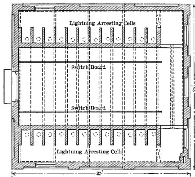
FIG. 60.—Ground Floor of Saratoga Switch-house.
