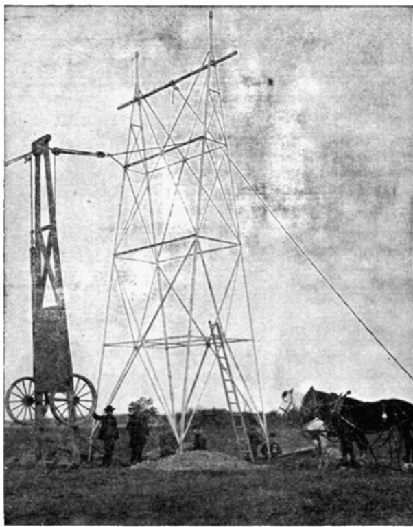
FIG. 99.—One of the Towers in Position.
