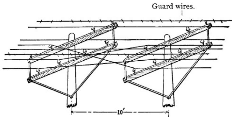
FIG. 72.—Transposition of Wires on Chambly Montreal Line.
