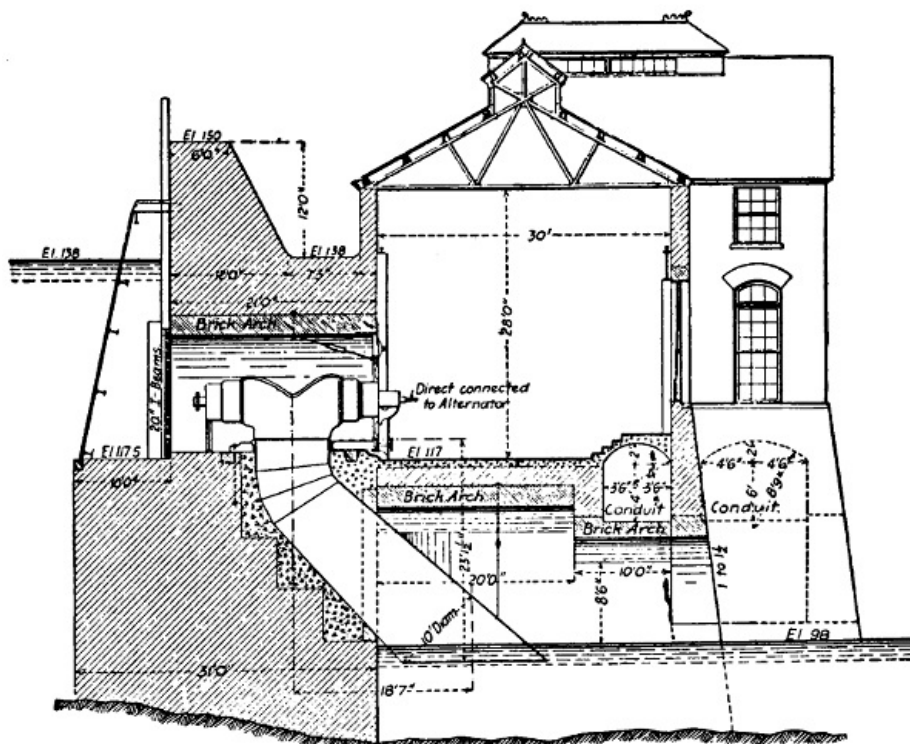
FIG. 25.—Cross Section of Columbus, Ga., Power-station.
