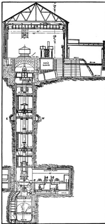
FIG. 29.—Section of Power-house No. 2 at Niagara Falls.
