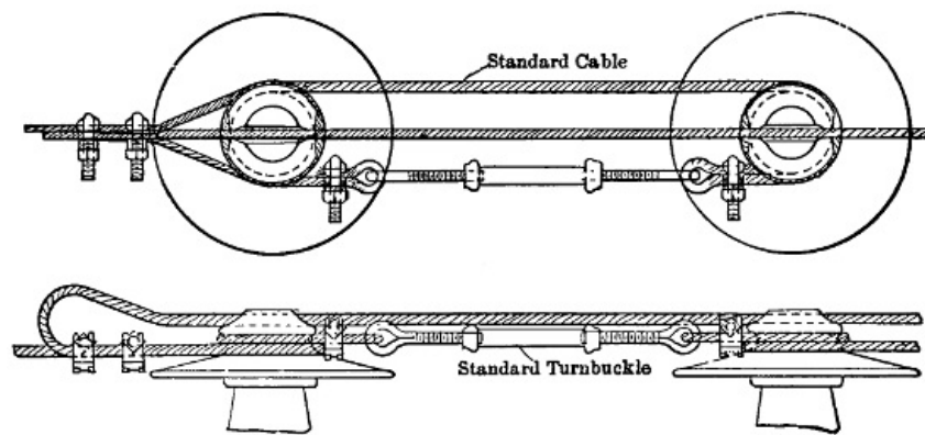
FIG. 105.—Take-up Arrangement on Terminal Tower.
