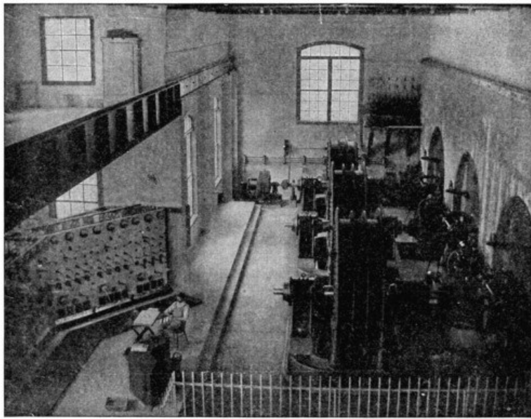
FIG. 49.—Columbus, Ga., Water-power Station.
