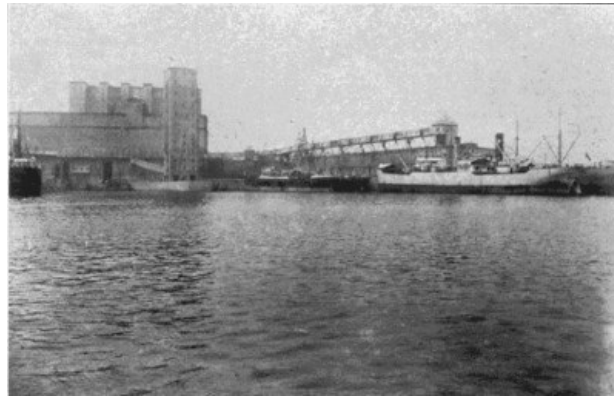
Grain Elevator No. 2. First entire concrete elevator in the world. Capacity 2,622,000 bushels
