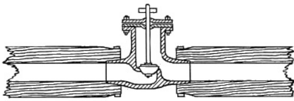
Valve for Wooden Pipes Used in the Philadelphia Water Supply
