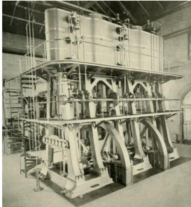
Modern Vertical Triple-Expansion Pumping Engine
