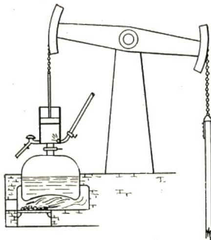
Newcomen's Engine
