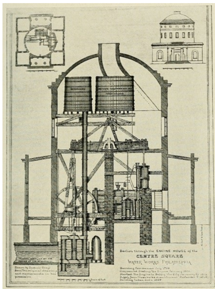
Section Through the Engine House of the Centre Square Water Works, Philadelphia
