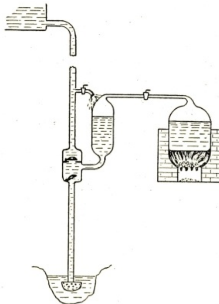
Savery's Engine
