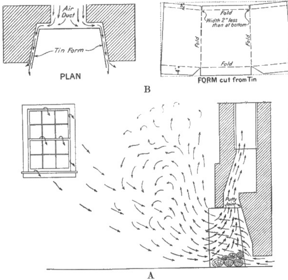
Fig. 19.—Simple form of warm-air flue for outside chimney. Air required for feeding the fire is brought in from the outside around a metal form set in the fireplace, with a space between it and the back and sides of the brickwork. As the cold outside air passes around the metal it becomes heated and is delivered into the room at a temperature much higher than where it is pulled in through window and door cracks. The result is a much more comfortable room.
