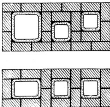
Fig. 6.—A division wall of at least 4 inches of brick should separate each flue from any others in the same chimney. Either of the arrangements shown will produce a good bond.
